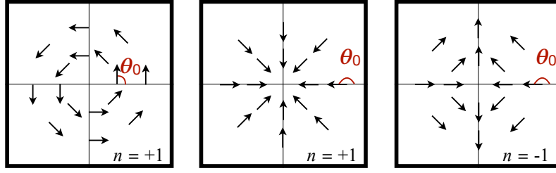
FIGURE 2.9 – Sketches of defects of the polar field. Left and center panels show respectively an anti-clockwise vortex and a sink, defined by a positive charge and a phase shift \theta_0 = \frac{\pi}{2} and \pi . Right panel represents a saddle that is negatively charged and for which \theta_0 = \pi .
