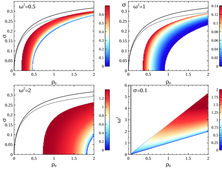
FIGURE 5.13 – Growth rate of the instability of the cholesteric solution of the active nematics equation for various twists \omega^2 . The dashed line represents the instability of the disordered solution and the full line above the existence of the homogeneous ordered solution. The first three panels show the linear stability of various fixed twist solutions in the density-noise plane. The fourth, bottom right panel shows the linear stability at fixed noise \sigma = 0.1 varying twist and density. The lower limit of the colored area corresponds to \omega^2 = \omega_u^2 , the upper limit of linear stability of the solution.
