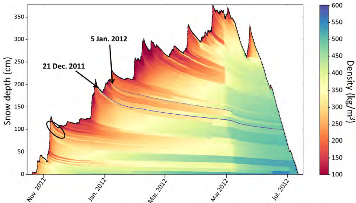
FIGURE 5.12 – Snow depth and snowpack density simulated at point A ( 42.65^{\circ}\text{N} , 0.65^{\circ}\text{E} , 2563 m, Fig. 5.3) during winter 2011/2012 by Crocus-ice, driven by AROME meteorological fields with freezing precipitation diagnostic (FPD). Ice layers are identified by a dark blue colour (more than 600 \text{ kg m}^{-3} ). The black circle indicates the formation of lower density crusts.
