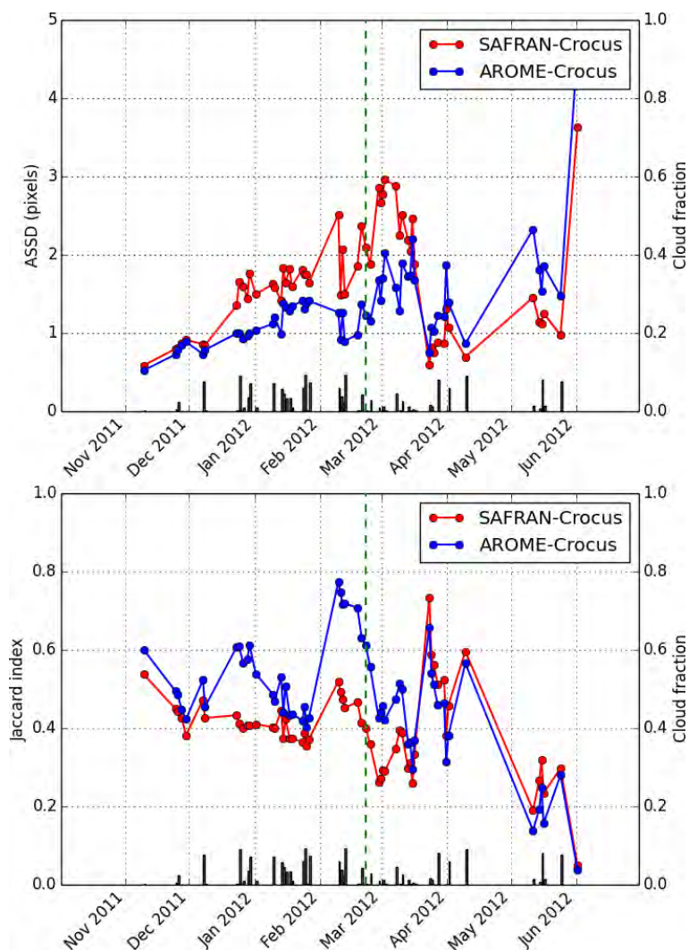
FIGURE 3.7 – Daily ASSD (top) and Jaccard index (bottom), within all massifs, AROME–Crocus vs MODIS (blue) and SAFRAN–Crocus vs MODIS (red), 2011-2012. Smaller ASSD and higher J mean better match with MODIS. The green line indicates 22 February 2012. The cloud fraction is represented by the black bars.
