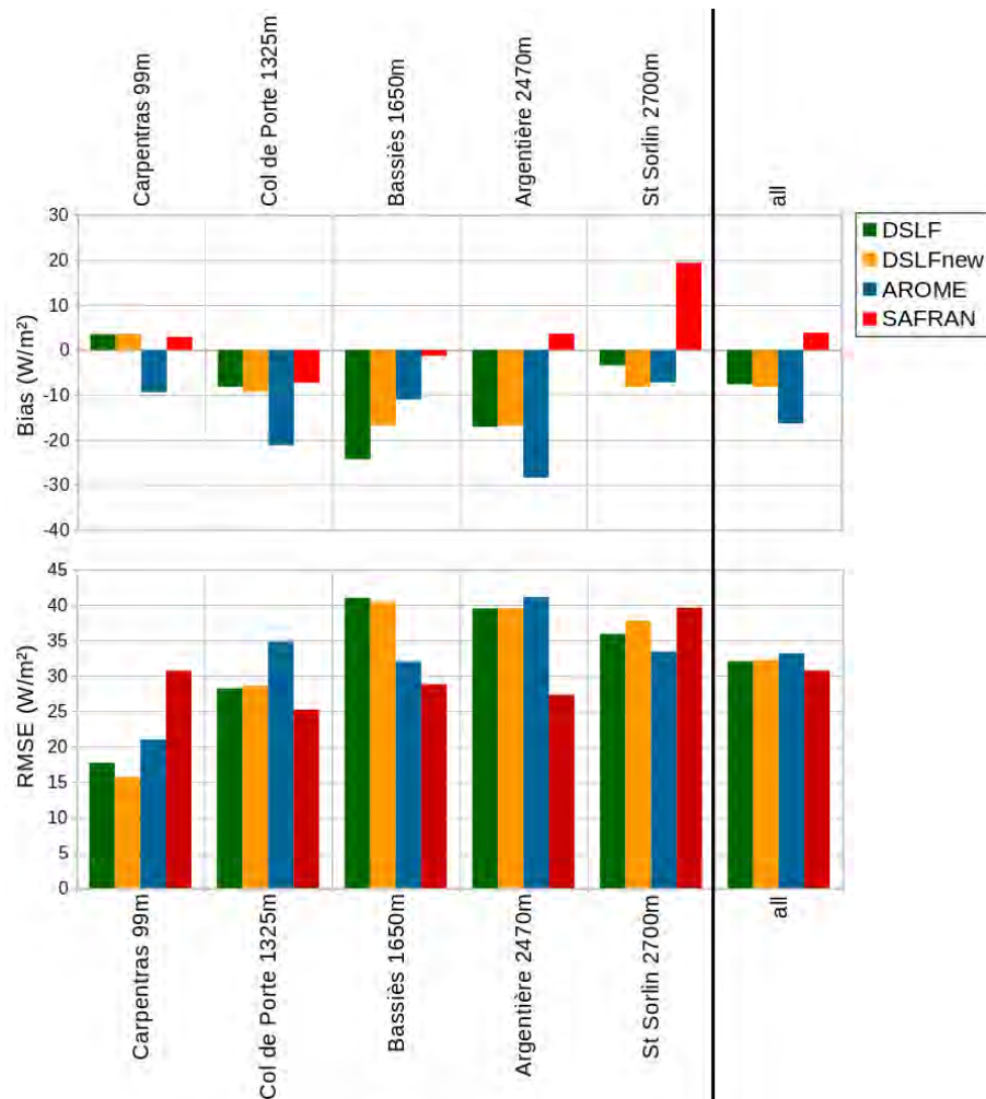
FIGURE 4.4 – Bias and RMSE of LW_{\downarrow} irradiance products (DSLF in green, DSLFnew in orange, AROME in blue, SAFRAN in red) compared to each station (left) and all stations (right).
