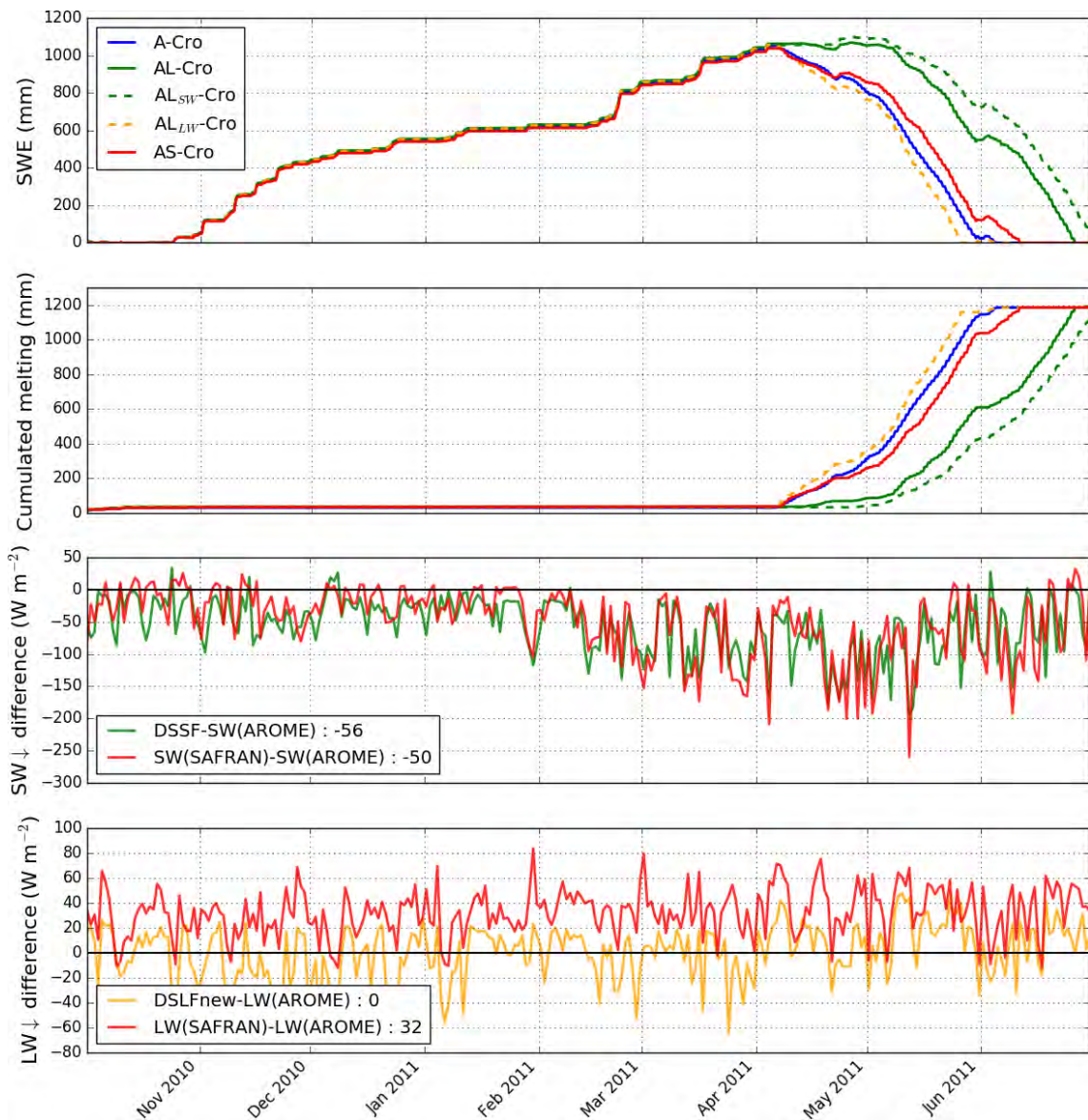
FIGURE 4.12 – Top : Snow Water Equivalent simulated by A-Cro (blue), AL-Cro (green), AL SW -Cro (dashed green), AL LW -Cro (dashed orange), AS-Cro (red) from 1 October 2010 to 30 June 2011 at point B in the Pyrenees (2459 m, Fig. 4.10). Middle : Cumulated melting represented with the same colours. Bottom : Mean daily irradiance differences with AROME for DSSF (green), DSLFnew (orange) and SAFRAN irradiances (red).
