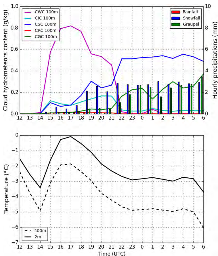
FIGURE 5.6 – Evolution of cloud hydrometeor content at 100m level (top, lines), hourly precipitation (top, bars) and temperature at 100m and 2m levels (bottom), forecast by AROME at point A ( 42.65^{\circ}\text{N} , 0.65^{\circ}\text{E} , 2563 m, Fig. 5.3) from 5 January 2012, 12 UTC, to 6 January 2012, 6 UTC.
