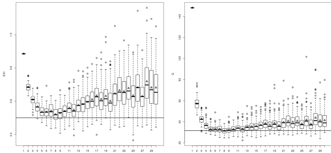
Figure 2.1 – Boxplot (with respect to the observation order) for \hat{\gamma} (left) and \hat{q}_{X,p} (right) in function of the block size.
