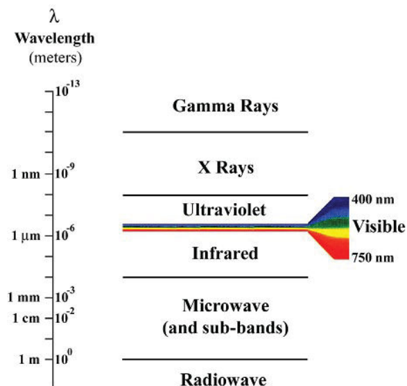
Figure 1: Electromagnetic spectrum (1)
