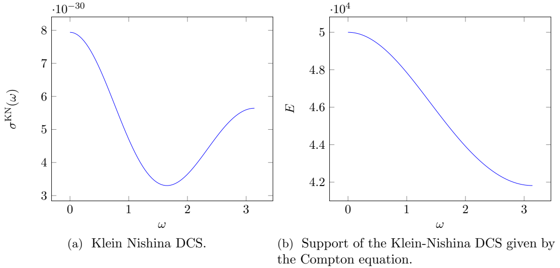
Figure 5.2: The Klein-Nishina differential cross section (DCS)
