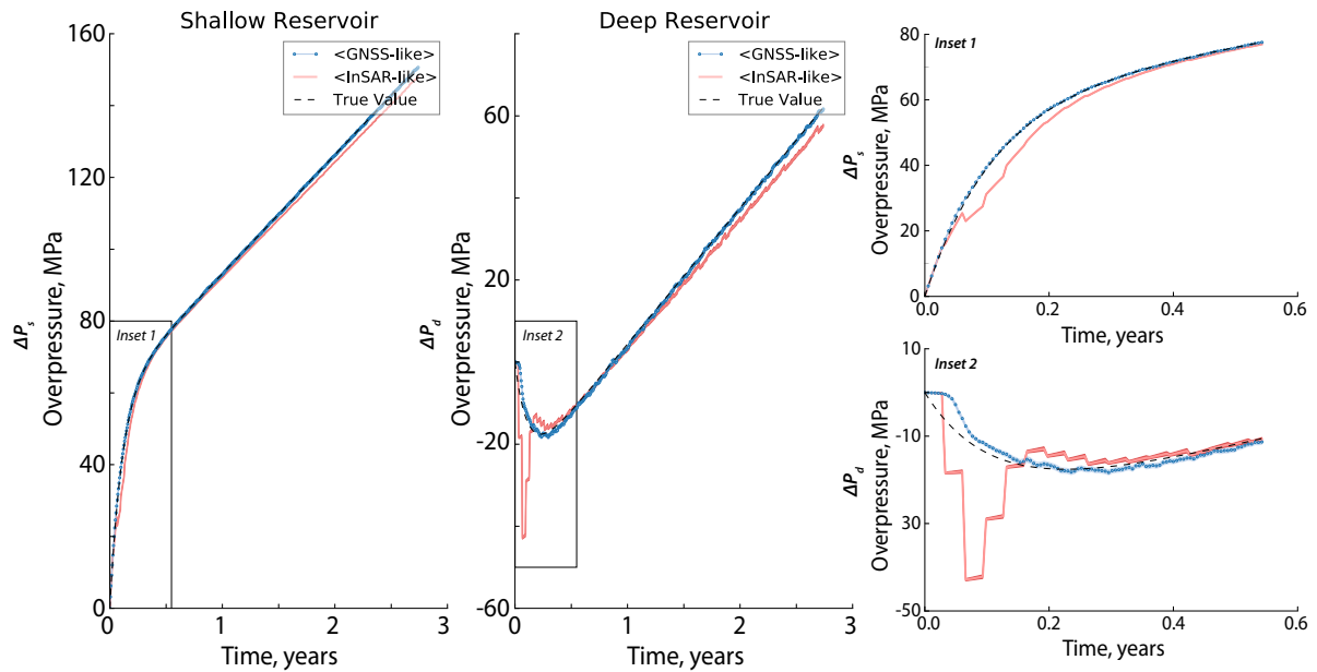
Figure 3.11: Influence of the frequency of observations on the assimilation: GNSS (10 observations that are assimilated every time step, f_{obs} = 1 , with distance to the volcanic center ranging from 1 to 5 km) vs. InSAR-like dataset (242 observations that are assimilated every 12 days, f_{obs} = 1/6 , with distance to the volcanic center ranging from 1 to 5\sqrt{2} km). Since parameter estimation is not possible to perform when InSAR dataset is used (see text), only the estimated overpressures are presented. Note that the initial conditions of the uncertain parameters are similar to those of in Figure 3.5C. The insets provide a closer image of the overpressures at the beginning of the assimilation. The light blue and red shades correspond to their spread ( 1\sigma ). Note that these values are difficult to discern since they are very small when compared to the scale of the plot. The black broken lines represent the true values.
