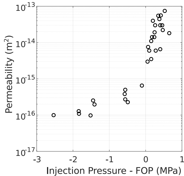
Figure 4.1: Permeability as a function of pressure in the injection borehole relative to the Fracture Opening Pressure (FOP) for all tests performed during the Tournemire tests. The FOP is defined for a resulting injection flow higher more than 100 mL/min.
