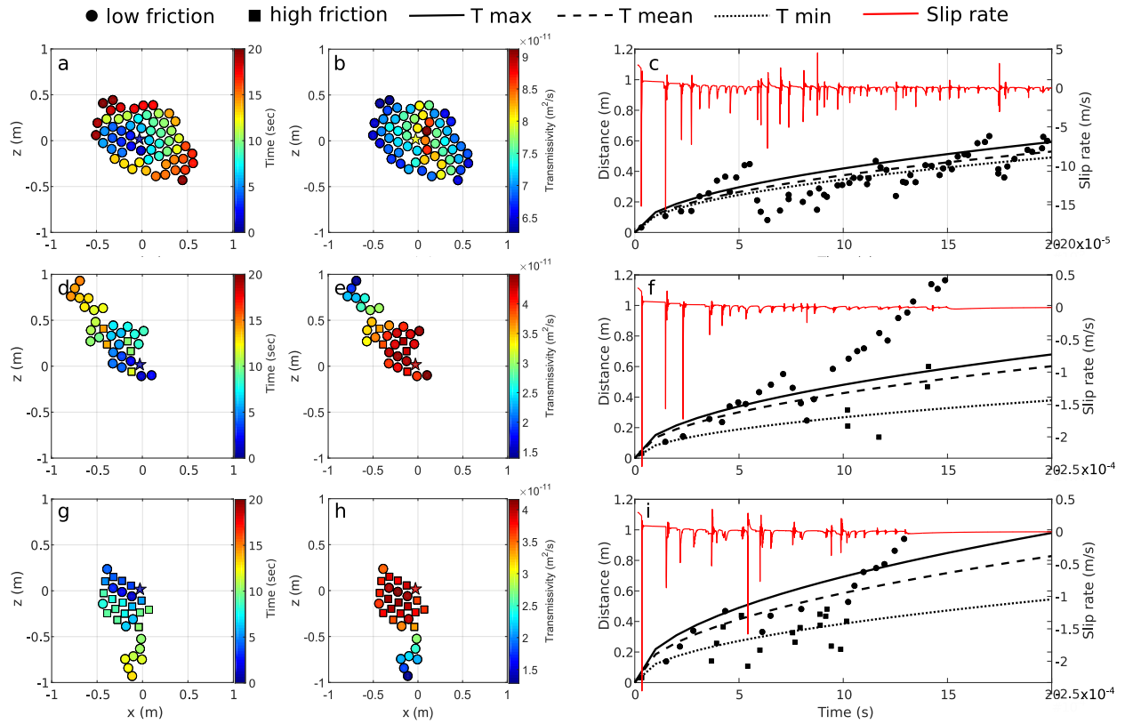
Figure 5.4: Heterogeneous distribution of the Coulomb friction: a) occurrence time and coordinates b) transmissivity values c) distance of the events from the injection point versus injection time and triggering front envelopes for 20% of frictional heterogeneities, d) occurrence time and coordinates, e) transmissivity values, f) distance of the events from the injection point versus injection time and triggering front envelopes for 60% of frictional heterogeneities, g) occurrence time and coordinates h) transmissivity values i) distance of the events from the injection point versus injection time and triggering front envelopes for 80% of frictional heterogeneities.
