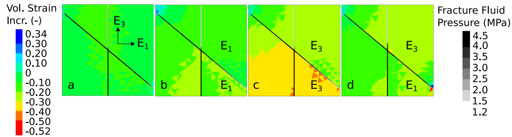
Figure 3.15: Volumetric strain increment and fracture fluid pressure variation for a) transversely isotropic material (reference), b) isotropic material with E = E_1 and \nu = \nu_{12} , c) isotropic material with E = E_3 and \nu = \nu_{13} = \nu_{23} , d) bi-material model with E = E_1 and \nu = \nu_{12} below the natural fracture and E = E_3 and \nu = \nu_{13} = \nu_{23} above the natural fracture.
