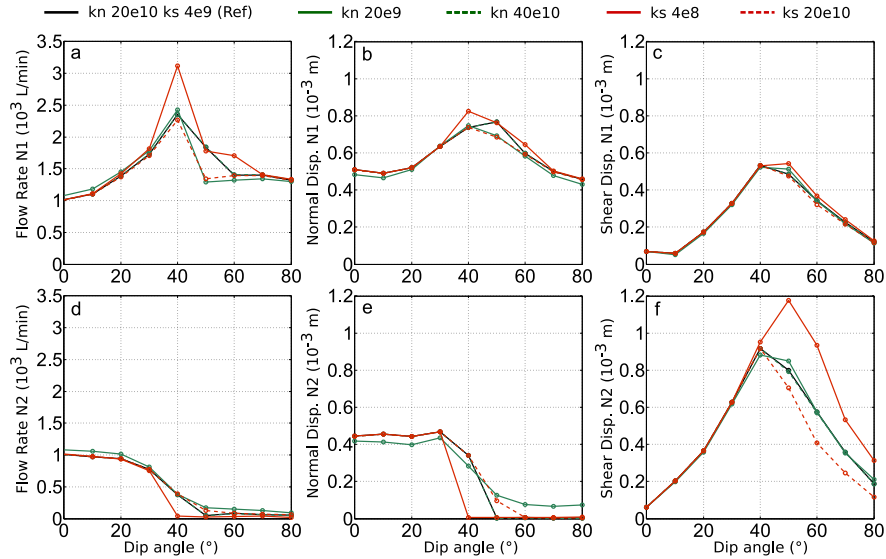
Figure 3.12: Variation of flow rate (left column), normal displacement (middle column) and shear displacement (right column) for N1 (top line) and N2 (bottom line) as a function of the elastic properties of the natural fracture.
