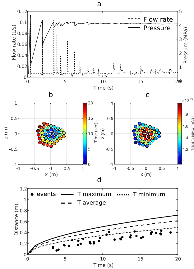
Figure 5.2: Reference case, the fault plane is aligned with the principal axes. a) Flow rate and pressure versus injection time recorded at the injection point throughout the calculation, b) occurrence time and coordinates of the rupture events, c) transmissivity values for each event, d) distance of the events from the injection point versus injection time and triggering front envelopes calculated using the maximum (solid line), the average (dashed line) and the minimum (dotted line) transmissivity value.
