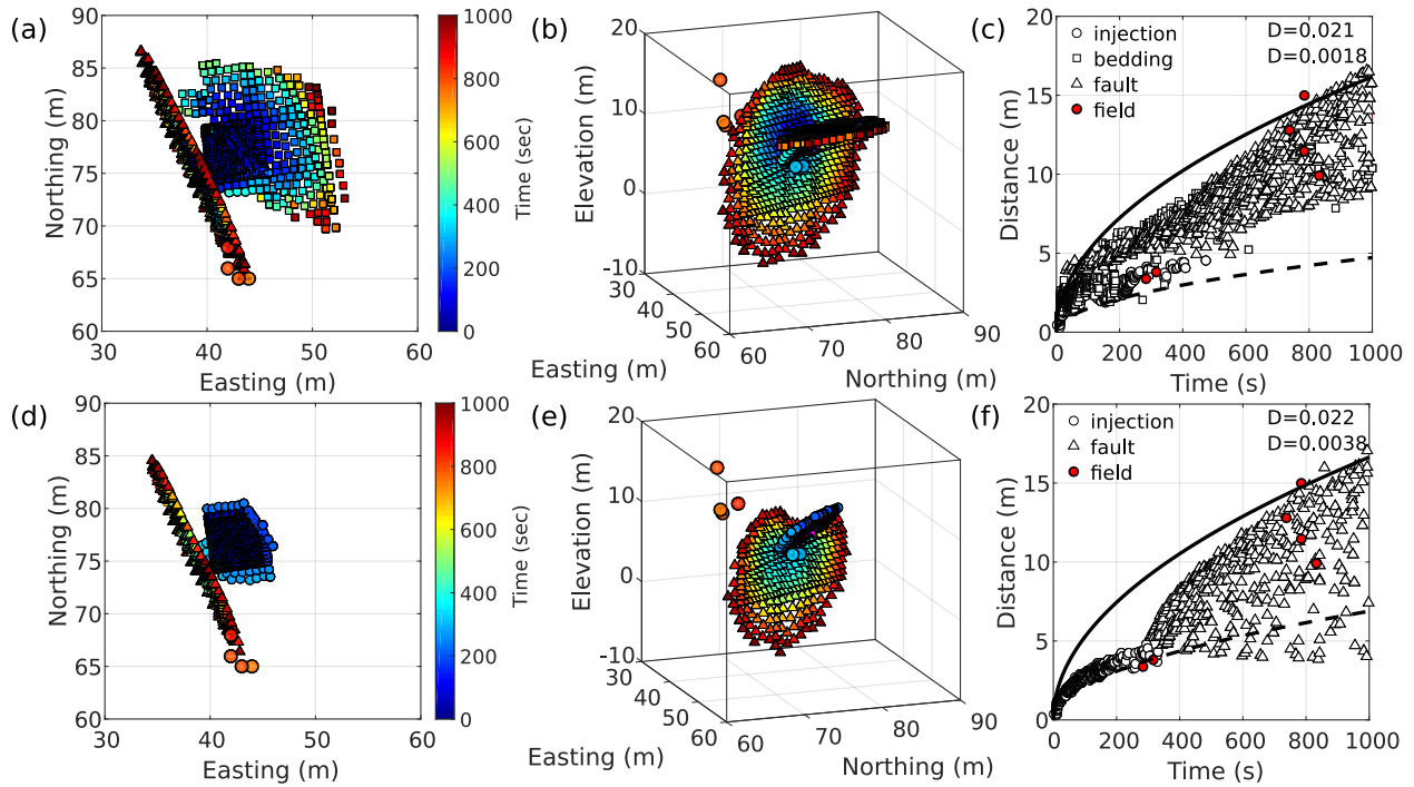
Figure 5.10: (Left) Map view, (middle) view from the East and (right) Distance of the rupture (model) and microseismic (field) events from the injection point as a function of time (r-t plot) for 3 planes model (top) and 2 planes model (bottom). The disks represent the injection plane events, the squares the bedding plane events, the triangles the fault plane events and the field microseismic events are disks characterized by a thicker line (red disks in r-t plots) The triggering front lines correspond to the maximum and minimum diffusivity of the injection plane.
