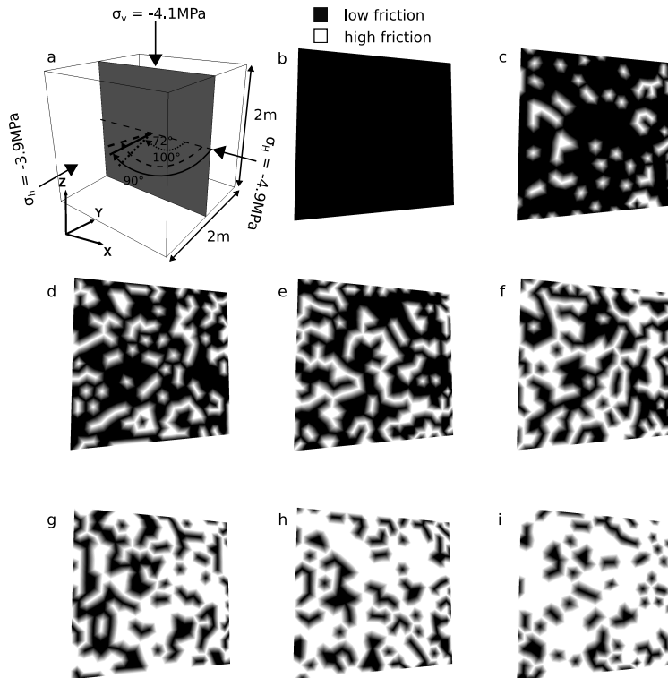
Figure 5.1: a) base case numerical model with the in situ stress field and the fault represented as a discontinuity separating two blocks, b) fault plane with homogeneous friction, c) with 20% of contacts, d) with 30% of contacts, e) with 40% of contacts, f) with 50% of contacts, g) with 60% of contacts, h) with 70% of contacts, i) with 80% of contacts.
