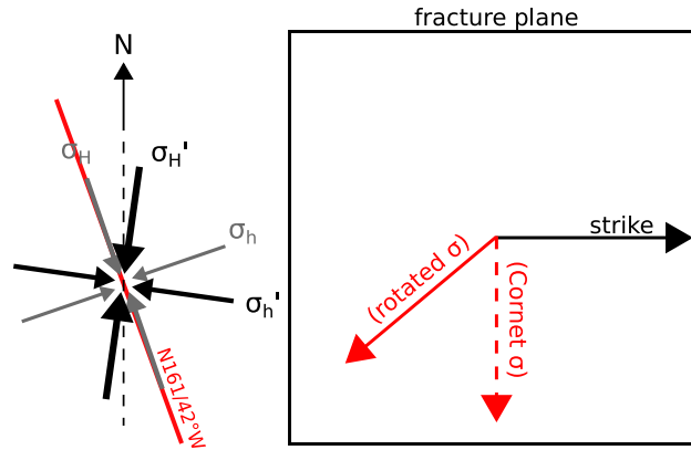
Figure 5.6: (Left): Rotated horizontal stresses 27° clockwise ( \sigma' ), and the N161-42°W fracture's strike line. (Right): Slip vector projected on the N161-42°W fracture resulting from the stress tensor as estimated by [Cornet, 2000] and Test 1 and for the rotated stress field (measured slip vector).
