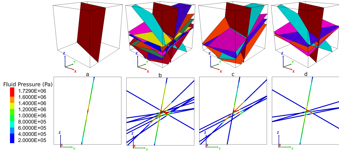
Figure 3.4: Model geometry and fluid pressure distribution shown along a vertical plane at the center of the model for t = 537 seconds corresponding to the end of the highest pressure test, for: (a) single secondary fault, (b) secondary fault with the sub-vertical and sub-horizontal families, (c) secondary fault with the sub-vertical family, (d) secondary fault with the sub-horizontal family.
