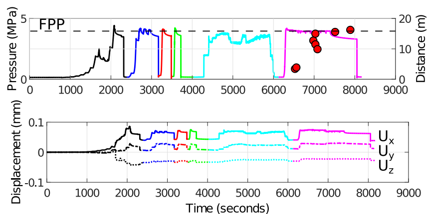
Figure 2.9: Test 2 results. Top: variation of pressure-versus-time, Fracture Propagation Pressure (FPP) and event distance from the injection test-versus-time (modified from De Barros et al. [2016]). Bottom: variation of probe displacements-versus-time.
