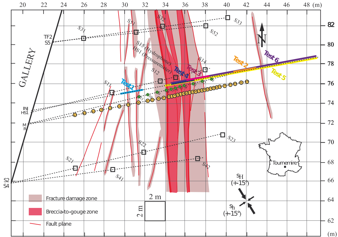
Figure 2.3: Horizontal map view of the instrumented experimental site. The locations of the different tests are shown along the injection borehole with different colors. The orange dots correspond to strain sensors, the green dots to resistivity sensors and squares correspond to accelerometric sensors (modified from De Barros et al. [2016]).
