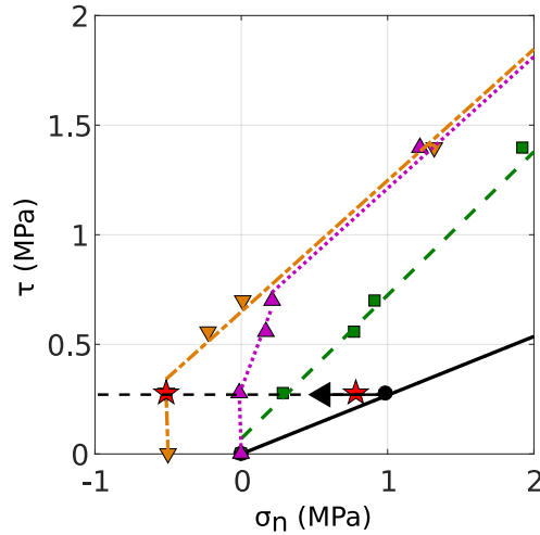
Figure 4.3: Equivalent failure envelopes for the fault plane: the black solid line corresponds to the homogeneous plane, the green dashed line to the case of higher friction heterogeneities, the purple dotted line to the case of higher friction, cohesion heterogeneities and the orange dash-dot line to the higher friction, cohesion, tensile strength heterogeneities. The black arrow indicates the direction of the evolution of the effective stress as the fluid pressure increases. The two red stars correspond to the two configurations presented in Figure 4.5 for the frictional case, i.e. the failure envelope corresponds to the green dashed line.
