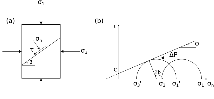
Figure 1.1: (a) Normal and shear stresses resolved on the plane of rupture; (b) Mohr diagram of shear stress ( \tau ) versus normal stress ( \sigma_n ) showing how the increasing fluid pressure ( \Delta P ) moves the Mohr circle towards the failure envelope.
