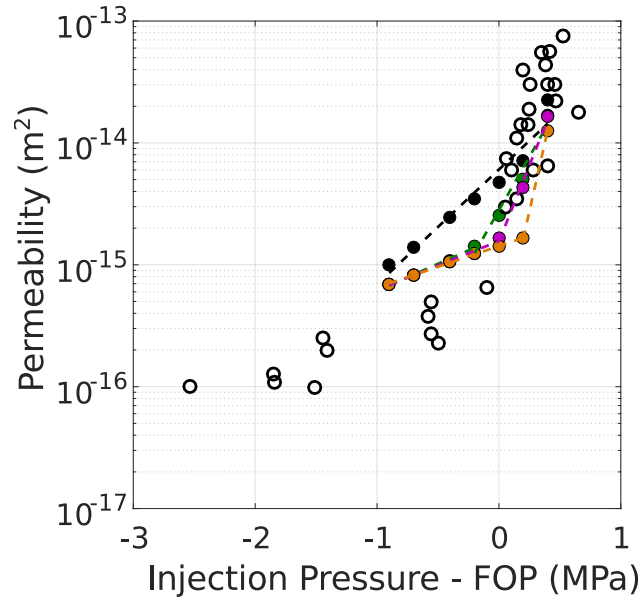
Figure 4.4: Permeability as a function of pressure in the injection borehole relative to the Fracture Opening Pressure (FOP) for (i) all tests performed during the Tournemire tests in black circles, (ii) the numerical tests for the uniform fault plane in black disks, (iii) the numerical tests for the heterogeneous fault plane with only frictional asperities in green disks, (iii) the numerical tests for the heterogeneous fault plane with frictional-cohesive asperities in purple disks and (iv) the numerical tests for the heterogeneous fault plane with frictional-cohesive-tensile strength asperities in orange disks.
