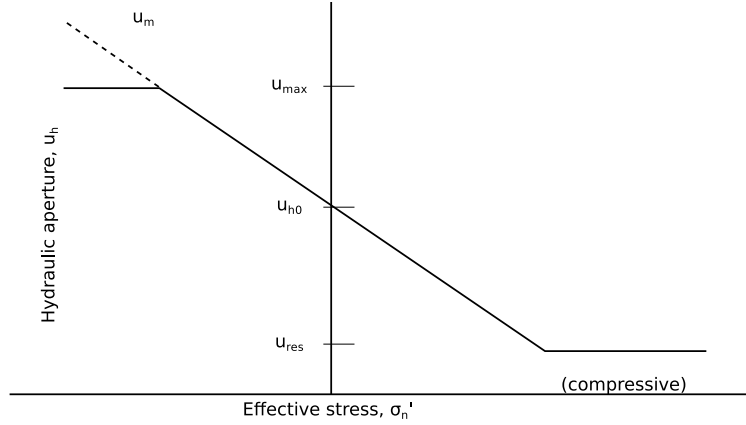
Figure 2.13: Idealized relation between hydraulic aperture and effective normal stress for a rock joint (after Itasca Consulting Group [2013]).
