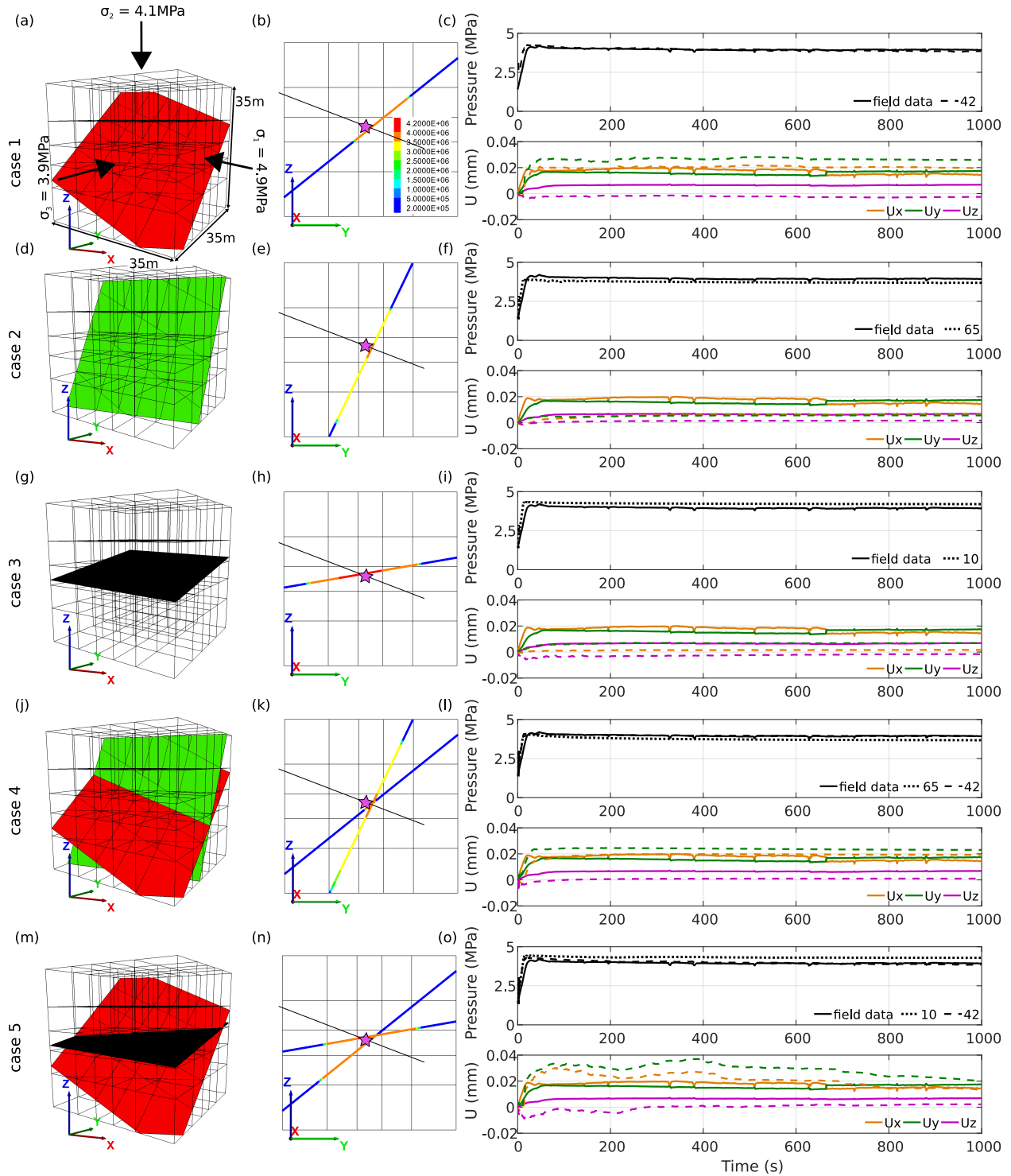
Figure 5.7: Left: model, middle: fluid pressure distribution along the fracture(s) in the z-y plane for t = 1000 seconds, right: fluid pressure and displacement variation versus time of the injection for the different configurations studied.
