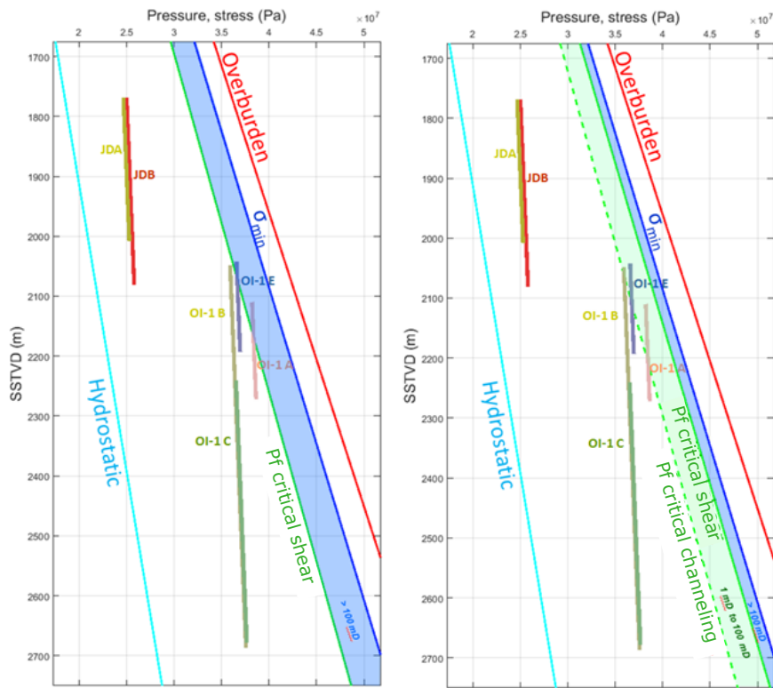
Figure 4.8: Pressure and stress state of the OI-1 and JD sands in minibasin fault blocks A. On the left the Finkbeiner et al. [2001] is presented. On the right, for the same stress states of the reservoirs OI-1 and JD but taking into account the critical fluid pressure above which channeling migration can be triggered while remaining in the stable mechanical domain of the fault zone.
