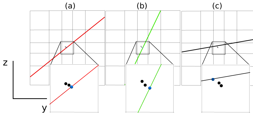
Figure 5.8: z-y view of the model with the zoomed in area (5 m × 5 m) around the anchors location for (a) N161-42°W fracture, (b) N174-65°W fracture and (c) N166-10°W fracture.
