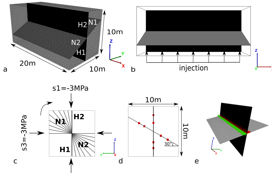
Figure 3.6: (a) Geometry of the numerical model, (b) application of injection pressure at the bottom of the hydraulic fracture plane, (c) stress field and rotation of the natural fracture dip from 0^\circ (perpendicular to the hydraulic fracture) to 80^\circ (almost parallel to the hydraulic fracture), (d) fluid pressure and displacement recording points (red squares) along the hydraulic and natural fractures, (e) flow zones (red and green) around the intersection for the calculation of the flow rate for each half-plane.
