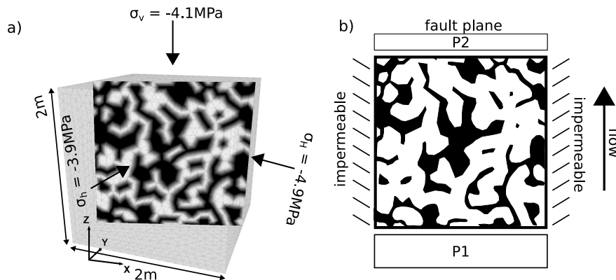
Figure 4.2: Geometry of the numerical model with the stress field applied and the distribution of the heterogeneities along the plane. The white areas represent low friction areas while the black areas represent the high friction areas. (b) Hydraulic pressure applied at the boundaries with P1 larger than P2.
