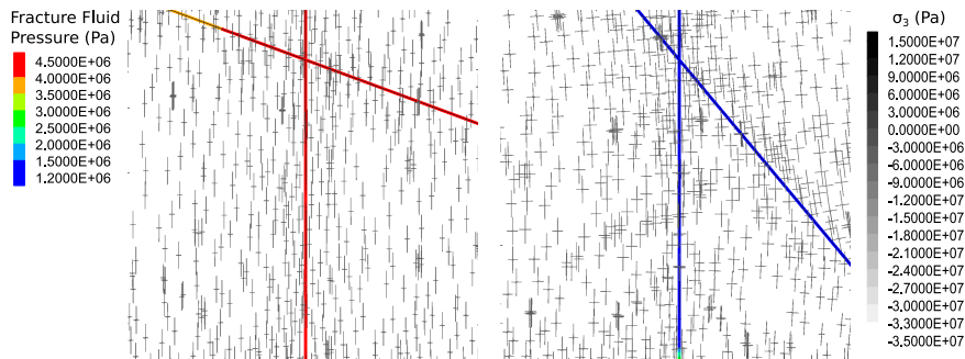
Figure 3.11: Stress tensor magnitudes inside the model and fluid pressure variation along the fracture for 20° (left) and 50° (right) natural fracture dip angle.
