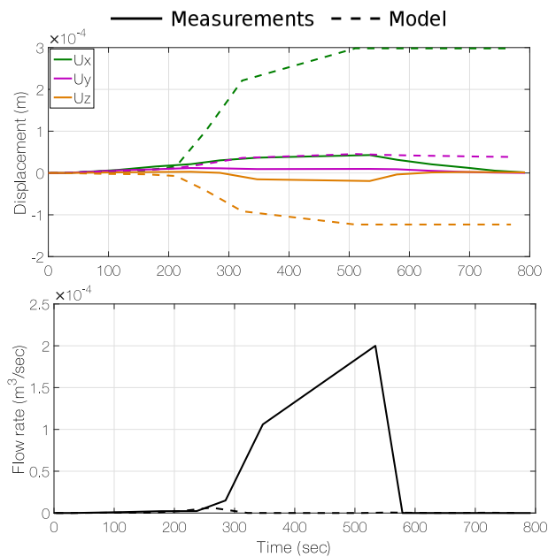
Figure 3.3: Displacements variation versus time (top), flow rate variation versus time (bottom) for the finite size fault.
