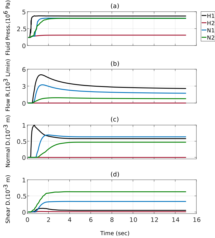
Figure 3.7: From top to bottom: (a) fracture fluid pressure, (b) flow rate, (c) normal displacement, (d) shear displacement versus time for the half-planes H1, H2, N1, N2.
