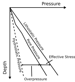
Figure 1.9: Schematic view of a pore pressure profile vs depth, bounded between the hydrostatic and the lithostatic pressure.
