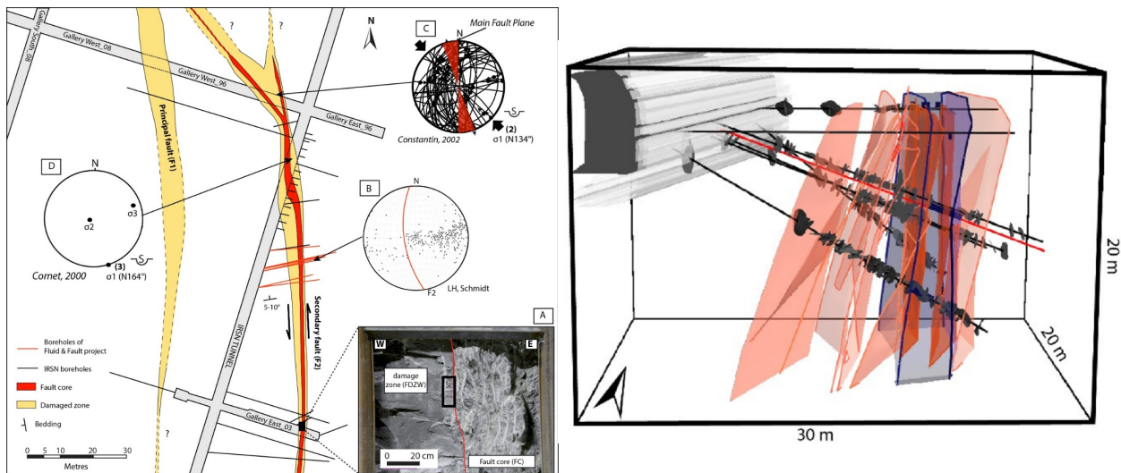
Figure 2.2: Left: IRSN URL structural map showing faults F1 and F2 (after Lefèvre et al. [2016]), right: 3D view of the secondary fault architecture (after Lefèvre [2016]).
