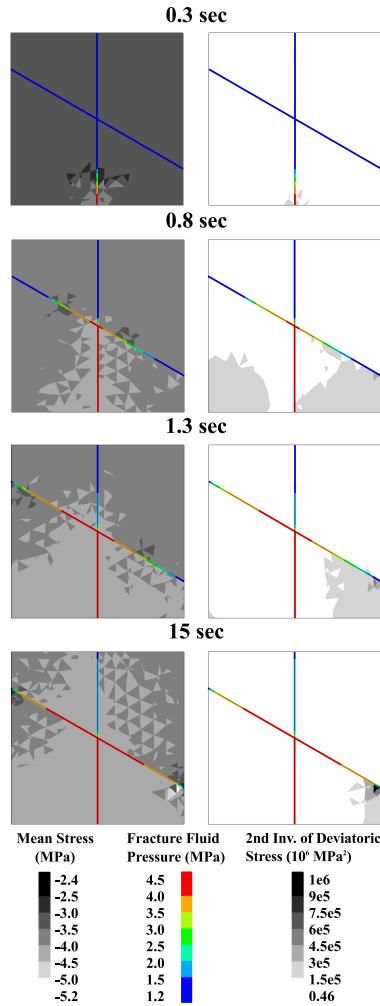
Figure 3.8: Evolution of the mean stress (left column), the second invariant of deviatoric stress (right column) and of the fracture fluid pressure at different injection times.
