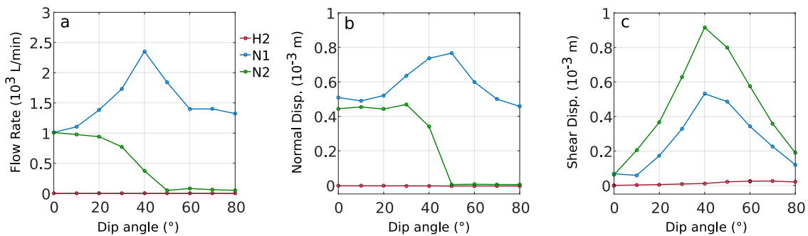
Figure 3.9: From left to right; (a) variation of the flow rate, (b) the normal displacement and (c) the shear displacement versus the dip angle of the natural fracture at the end of the simulation for half-planes H2, N1, N2.
