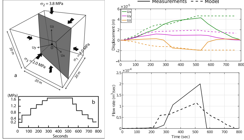
Figure 3.1: Left: Geometry of the single persistent fault model and the applied stresses. Right: Best-fit numerical solutions of fault hanging wall displacements (upper graphs) and flow rate (lower graphs) (modified from Guglielmi et al. [2015b]).
