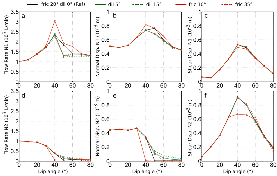
Figure 3.13: Variation of flow rate (left column), normal displacement (middle column) and shear displacement (right column) for N1 (top line) and N2 (bottom line) as a function of the strength properties of the natural fracture.
