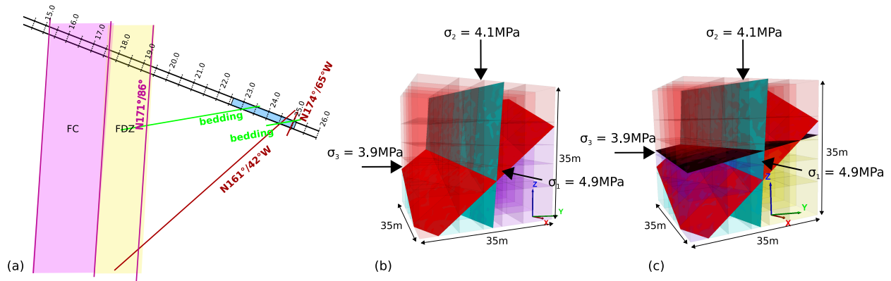
Figure 5.9: (a) Conceptual model showing the intersection of the injection planes with the fault planes. (b) Single injection plane (N161-42°W) and fault plane model. (c) Two injection planes (N161-42°W and N166-10°W) and fault plane model.
