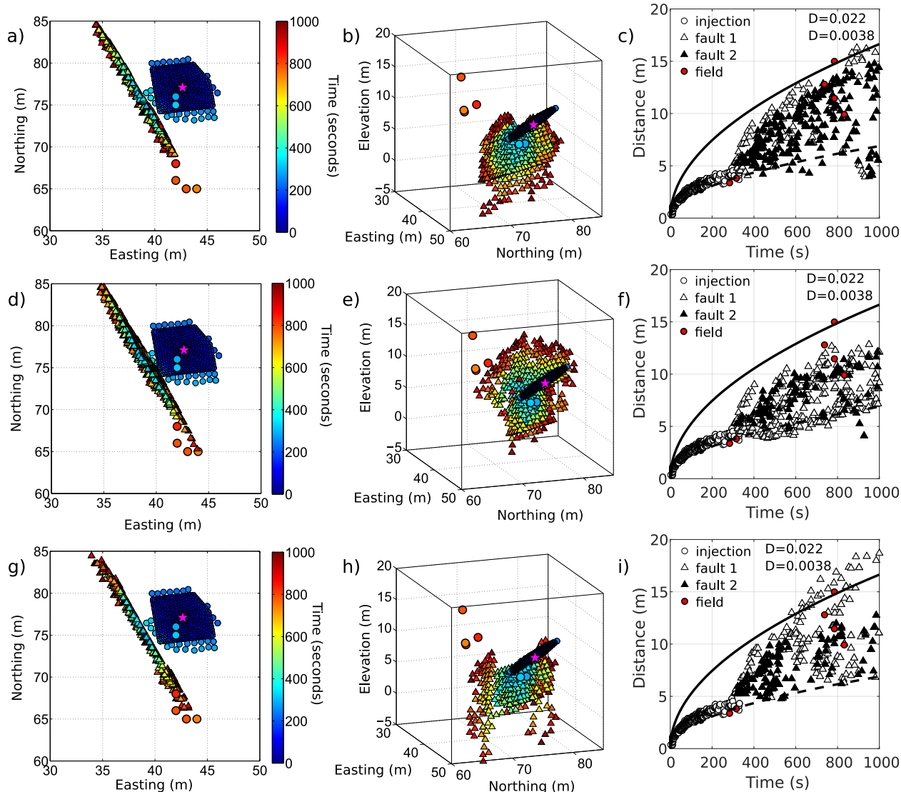
Figure 5.12: (Left) Map view, (middle) view from the East and (right) Distance of the rupture (model) and microseismic (field) events from the injection point as a function of time (r-t plot) for 3 planes model (top) and 2 planes model (bottom). In the r-t plot, the disks represent the injection plane events, the hollow triangles the low friction fault plane events, the solid triangles the high friction events and the field microseismic events are the disks characterized by a thicker line (red disks in r-t plots) The triggering front lines correspond to the maximum and minimum diffusivity of the injection plane.
