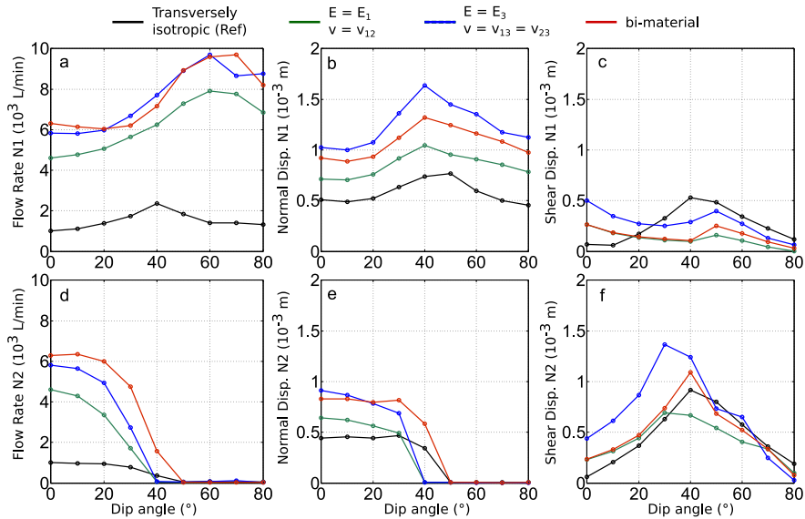
Figure 3.14: Variation of flow rate (left column), normal displacement (middle column) and shear displacement (right column) for N1 (top line) and N2 (bottom line) as a function of the elastic properties of the surrounding medium.
