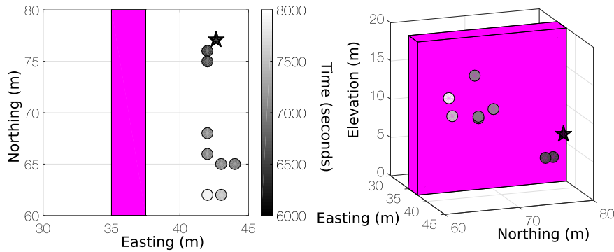
Figure 2.10: Left: map view, right: view from the East of the location of the microseismic events for Test 2 results. The occurrence time of the results is also shown. The position of the center of the injection interval is represented by a star (modified from De Barros et al. [2016]).
