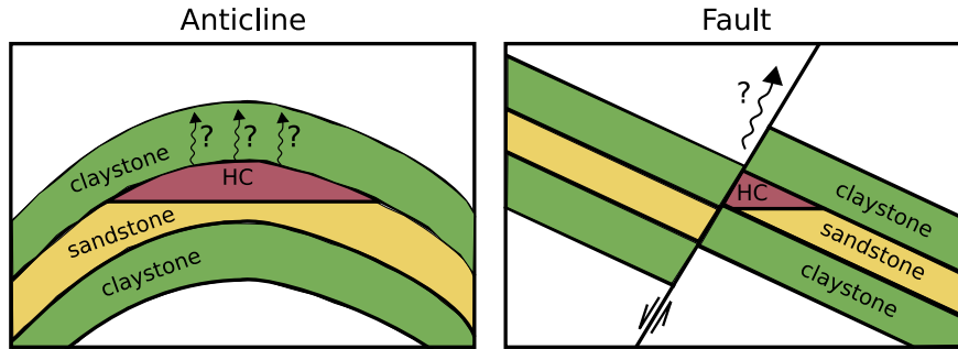
Figure 1: Examples of structural traps and the associated questions related to caprock or fault seal integrity.
