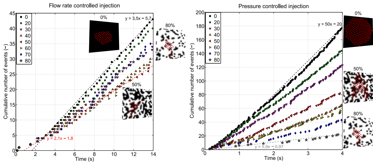
Figure 5.5: Cumulative number of events for a flow rate controlled injection (left) and a pressure controlled injection (right). Pressurized and rupture zones for 0%, 50% and 80% of heterogeneities for a flow rate and pressure controlled injection.
