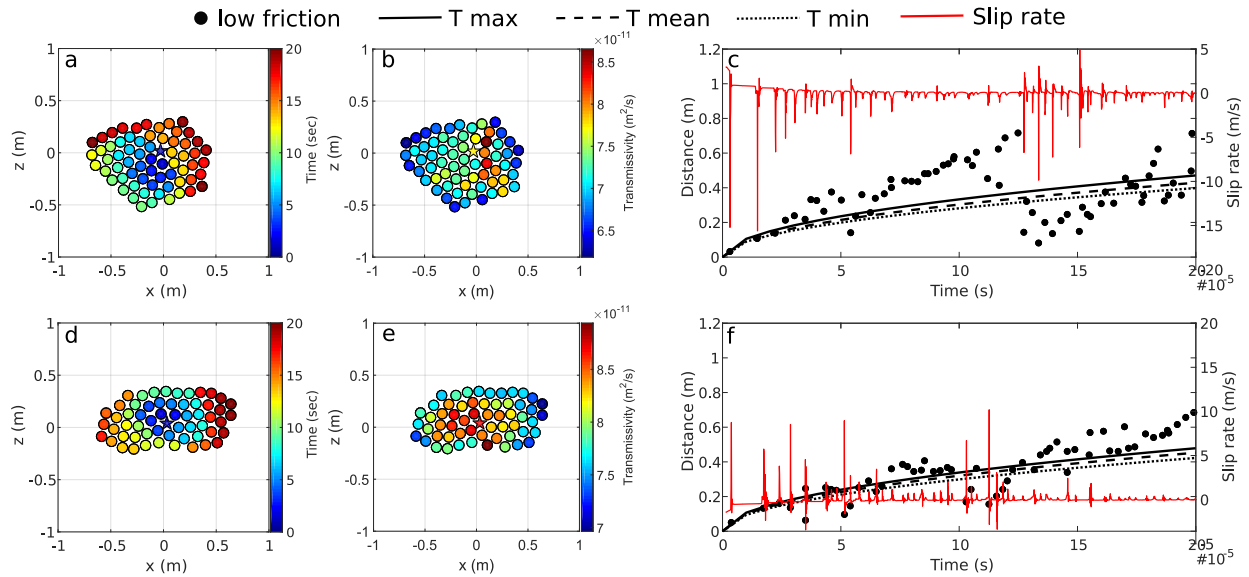
Figure 5.3: Fault plane orientation: a) occurrence time and coordinates b) transmissivity values c) distance of the events from the injection point versus injection time and triggering front envelopes for an angle of 72° between the normal of the fault and the maximum horizontal stress, d) occurrence time and coordinates e) transmissivity values f) distance of the events from the injection point versus injection time and triggering front envelopes for an angle of 100° between the normal of the fault and the maximum horizontal stress.
