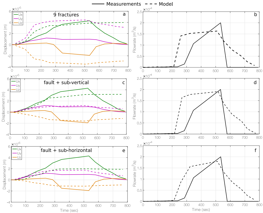
Figure 3.5: Displacement (top) and flow rate versus time for: 1st line: secondary fault with the sub-vertical and sub-horizontal families (9 fractures), 2nd line: secondary fault with the sub-vertical family, 3rd line: secondary fault with the sub-horizontal family.
