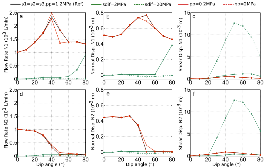
Figure 3.10: Variation of flow rate (left column), normal displacement (middle column) and shear displacement (right column) for N1 (top line) and N2 (bottom line) as a function of stress and initial pore pressure.
