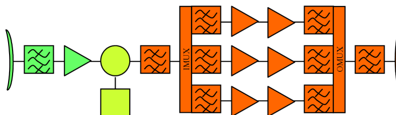
FIGURE 1.10 – Design multicanaux
