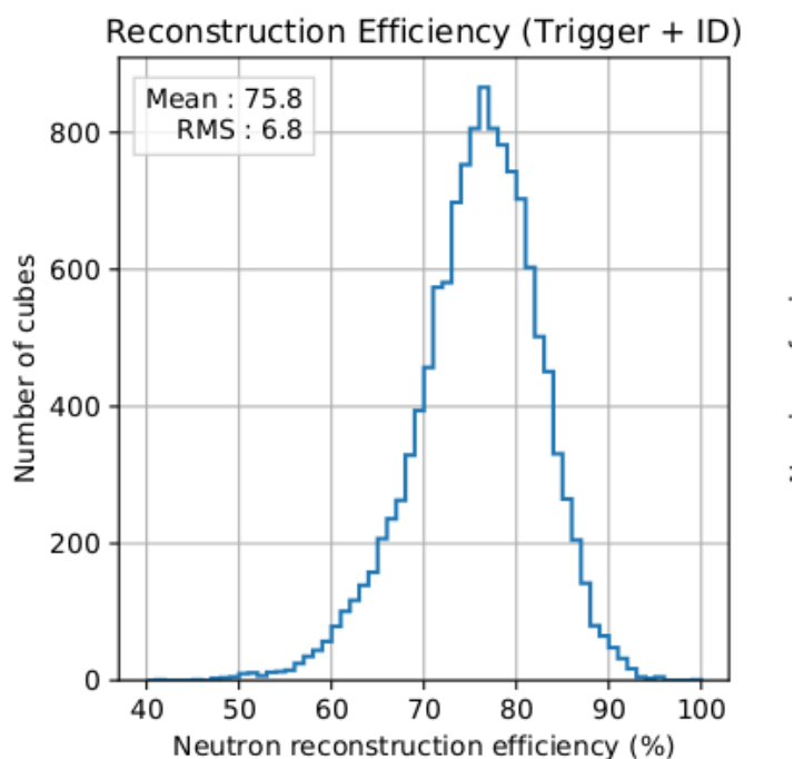
Figure 6.17: Neutron reconstruction efficiency from calibration campaigns with CROSS.
