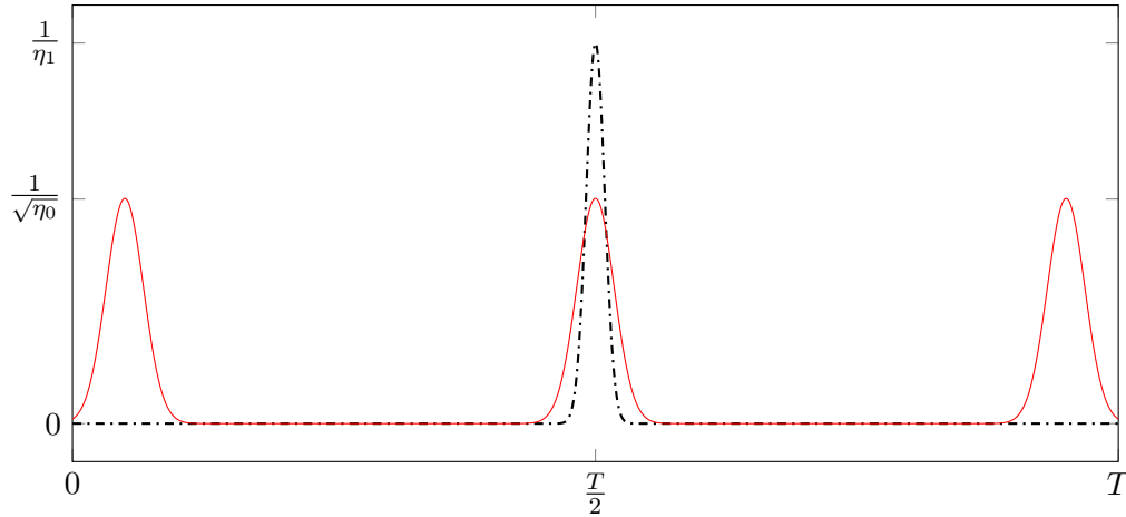
FIGURE 4.2: A comparison of the amplitudes of the controls g^0 (red continuous line) and g^1 (black dotted line) over the time interval [0, T]
