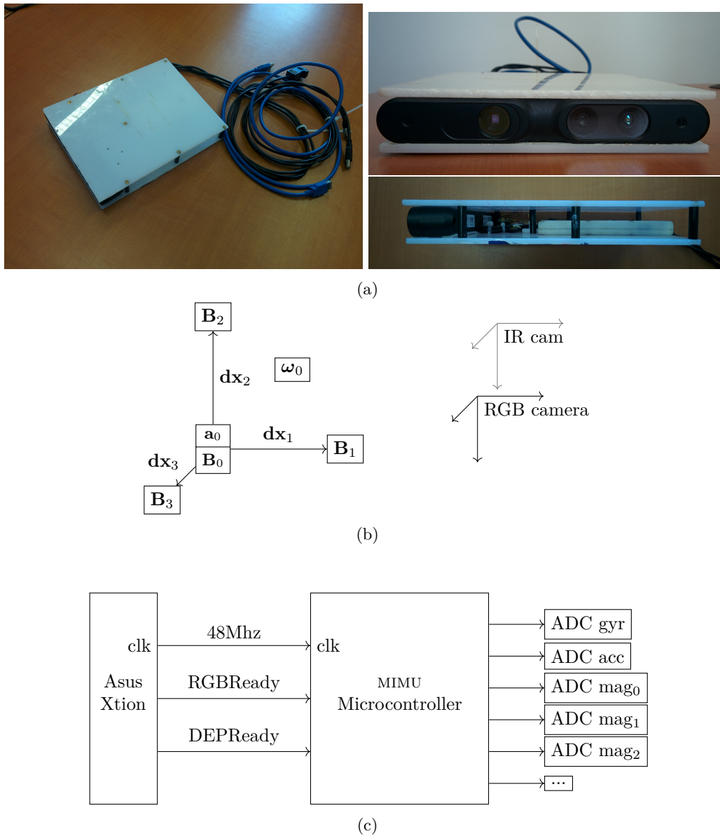
Figure 3.1: Hybrid sensor combining MIMU + RGBD camera used in this chapter. (a) Views of the system; (b) schematic view of the coordinate frames at play; (c) Schematic of electronic of the prototype built for the experiment of this chapters. Note that MIMU microcontroller is cadenced with Asus Xtion clock (clk arrow). This simple hack allows timestamping consistently Asus Xtion image with respect to MIMU digitization of sensors.
