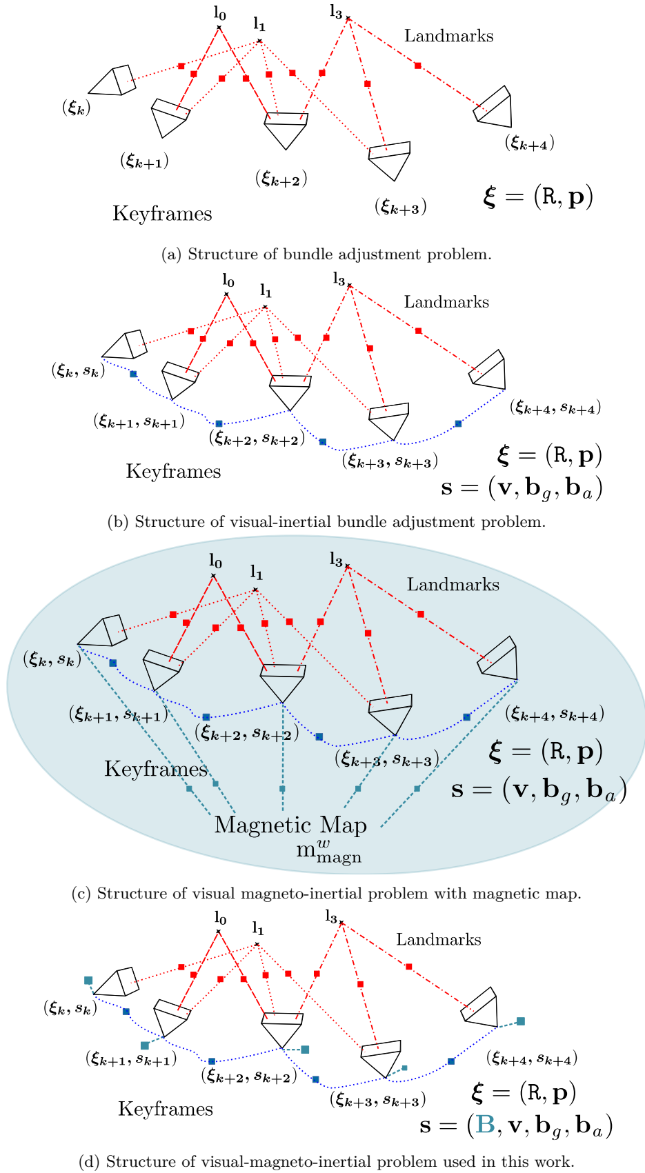
Figure 5.1: Bundle adjustment problems
