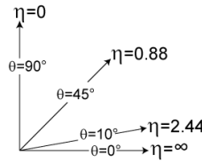
Figure 2.8: Some useful pseudorapidity values and the respective \theta values
