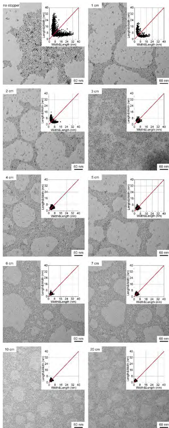
Figure III.9. TEM images and 2D size plots of the ZnO/2DDA NPs versus length tube (diameter 2 mm).
