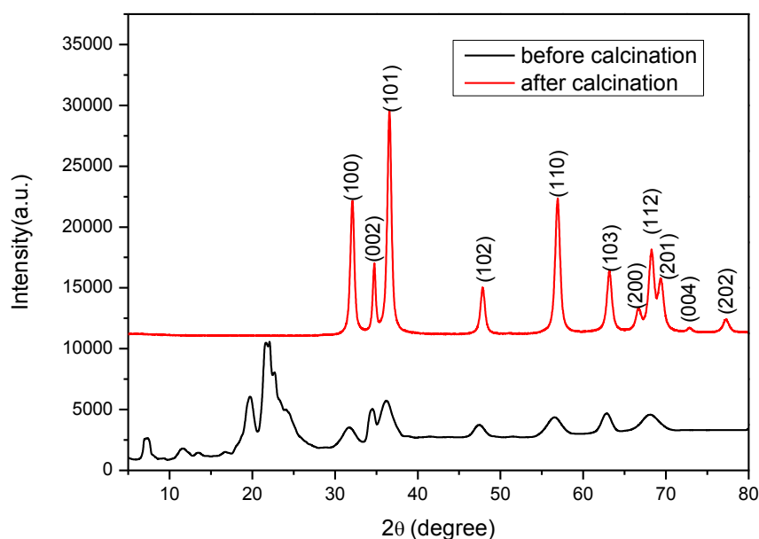
Figure IV.17 PXRD patterns before (a) and after (b) calcination of the ZnO hybrid material. The peak indications correspond to the hexagonal zincite phase, space group P63mc.
