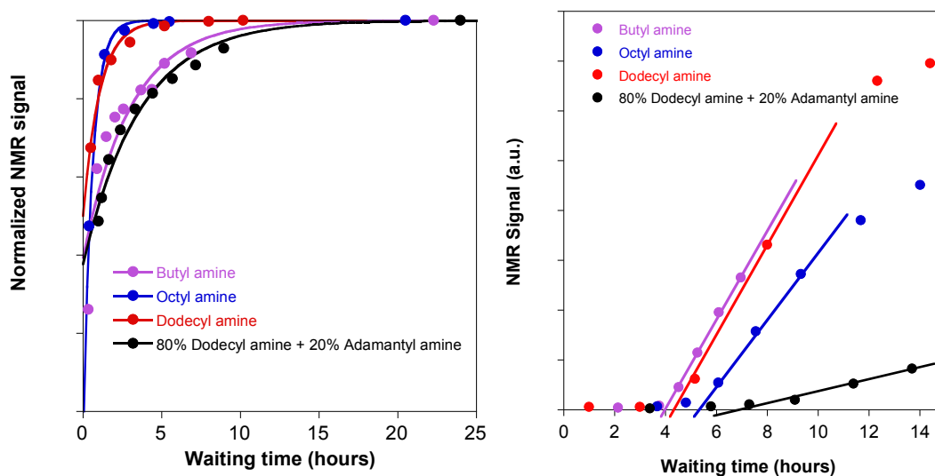
Figure IV.11 (Left) Normalized area of the cyclohexane ^{13}\text{C} resonance (in the DP-MAS experiment) as a function of waiting time for the [\text{ZnCy}_2]/\text{amine} (1:2) mixture, for four types of amine. The data are roughly fitted with the following equation: y = \ln\left(\frac{I_f - I(t)}{I_f}\right) I_{\text{normalized}} = 1 - \exp(-(t+t_a)/t_c) where t_a and t_c are respectively an adjusting time and a characteristic time of cyclohexane formation. The adjusting time (which was found positive and can be related to some fast initiation process - the kinetic is not a simple exponential decay-) as well as the characteristic time (see Table 1 in the main text) increased with the amine order Octyl amine ( t_a \sim 0 h) < Dodecyl amine ( t_a \sim 0.7 h) < Butyl amine ( t_a \sim 1.5 h) < Mixture 80% of dodecyl amine + 20% adamantyl amine ( t_a \sim 1.8 h). (Right) Integrated area of the whole ^{13}\text{C} spectrum (in the CP-MAS experiment, see Figure SI8) as a function of waiting time for the [\text{ZnCy}_2]/\text{amine} (1:2) mixture, for four types of amine. For each sample, a line is drawn to estimate the onset time of gelification (see Table IV.2).
