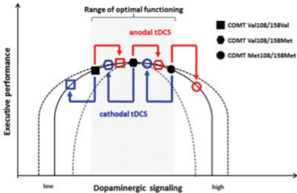
Figure 37 - Role of COMT polymorphism on tDCS effects - Inverted U-shape hypothesis - Based on the U-shape hypothesis, anodal and cathodal tDCS could exert a differential impact of executive performance depending on the individual dopaminergic signal level in the frontal cortex, which is related to individual genetic profile. COMT Val/Val would have a lower dopaminergic signal compared to COMT Val/Met, whereas COMT Met/Met would have a higher dopaminergic signal. Adapted from Wiegand et al, 2016.
