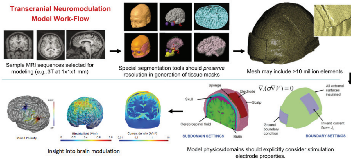
Figure 23: Imaging and Computational workflow - Individualized model of the electric field and current during tDCS - Adapted from Bikson et al., 2012; Peterchev, 2017; Rawji et al., 2018. This workflow represents the general steps involved in the generation of realistic MRI-derived finite-element head models. It should be noted that this workflow can vary depending on the software used.
