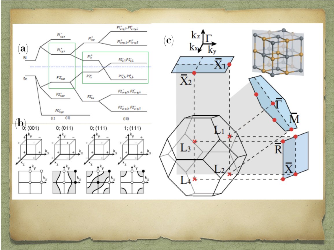
Figure 2.1: (a) The band inversion as seen in Bi 2 Se 3 shown by means of bonding and anti-bonding orbitals derived from the atomic orbitals of Bi and Se . Adapted from [54] (b) The trivial (0) and topological (1) phases of a 3D TI as derived by Kane and Mele using the parities of the wavefunction at TRIM [44]. (c) Surface topological states arise at TRIM given by the projections on the (001), (111) and (110) surfaces respectively of the bulk symmetries. Adapted from [51].
