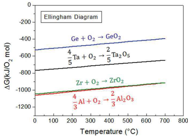
Figure 70: Ellingham diagram
