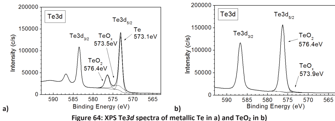
Figure 64: XPS Te3d spectra of metallic Te in a) and TeO 2 in b)
