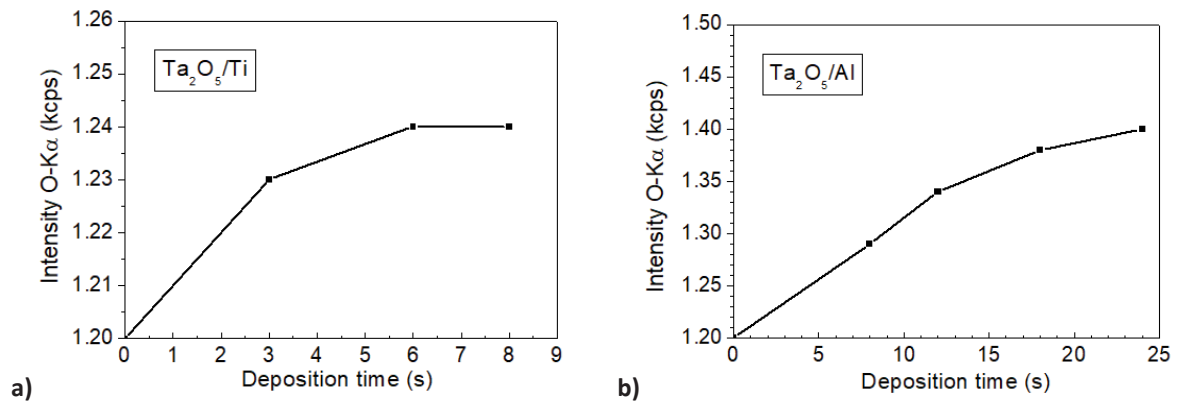
Figure 45: WDXRF O-K \alpha intensity in function of the deposition time for a) Ta 2 O 5 /Ti-based samples and b) Ta 2 O 5 /Al-based samples
