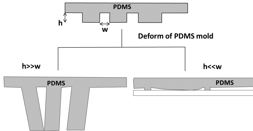
Figure II-9: Deformation of PDMS molds.
