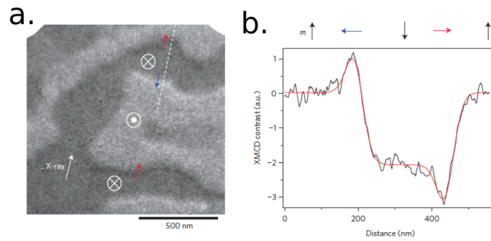
Fig. 7.4: Imaging of the chiral Néel structure of domain walls using XMCD-PEEM magnetic microscopy. a. Magnetic image of a multidomain state in the continuous Pt/Co/MgO film. For DWs lying perpendicular to the X-ray beam direction, thin white and black lines can be seen, corresponding to the magnetization being aligned antiparallel and parallel to the photon beam respectively. b. Line scan of the magnetic contrast corresponding to the dotted white line in (a). Image from [Bou+16].
