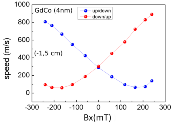
Fig. 6.9: DW speed vs. in-plane magnetic field B_x , measured in the position -1.5cm for up/down and down/up DW propagating in \pm direction, driven by 20ns long B_z pulses of 77.5mT in -1.5cm position.
