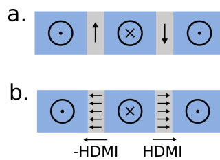
Fig. 2.12: Sketch of a. a Bloch wall and b. a chiral Néel domain wall, stabilized by DMI (top view).
