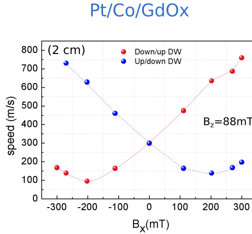
Fig. 4.14: DW speed vs in-plane magnetic field H_x , measured for up/down and down/up DW propagating in \pm direction, driven by 20ns long B_z pulses of 88mT in 2cm position.
