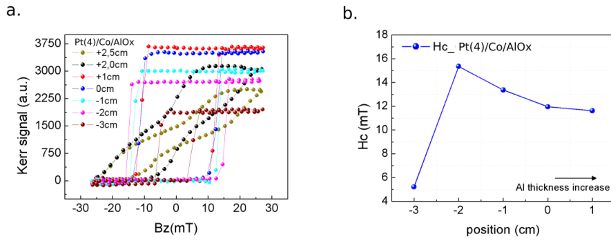
Fig. 5.8: a. Hysteresis loops measured by magneto-optical Kerr effect in different positions of the Pt(4)/Co/AlOx wedge b. curve of coercive field of the same sample.
