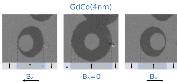
Fig. 6.8: Differential Kerr images showing the expansion of a bubble domain, driven by an out-of-plane field B_z = 77\text{mT} , in the presence of an in plane magnetic field of -62\text{mT} , 0\text{mT} and +62\text{mT} .
