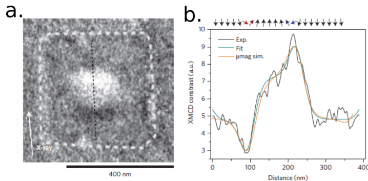
Fig. 7.5: Magnetic skyrmion observed at room temperature and zero applied external magnetic field a. XMCD-PEEM image of a 420 nm square dot (indicated by the dotted line) and b. line scan along the dotted black line (black line). The line scan has been averaged perpendicularly to the linescan over 30 nm. Image from [Bou+16].
