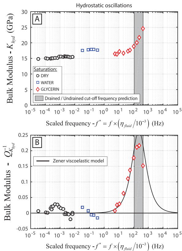
Figure 11. (a) Bulk modulus K_{hyd} and (b) Q_{K_{hyd}}^{-1} resulting from the hydrostatic oscillations at P_{diff} = 2.5\text{MPa} , under dry-, water-, and glycerin-saturated conditions. The frequency is scaled with the viscosity of the saturating fluid \eta_{fluid} . The factor Q_{K_{hyd}}^{-1} is compared with Zener's model. The range for the drained/undrained cutoff frequency f_1^* is represented by the gray area.
