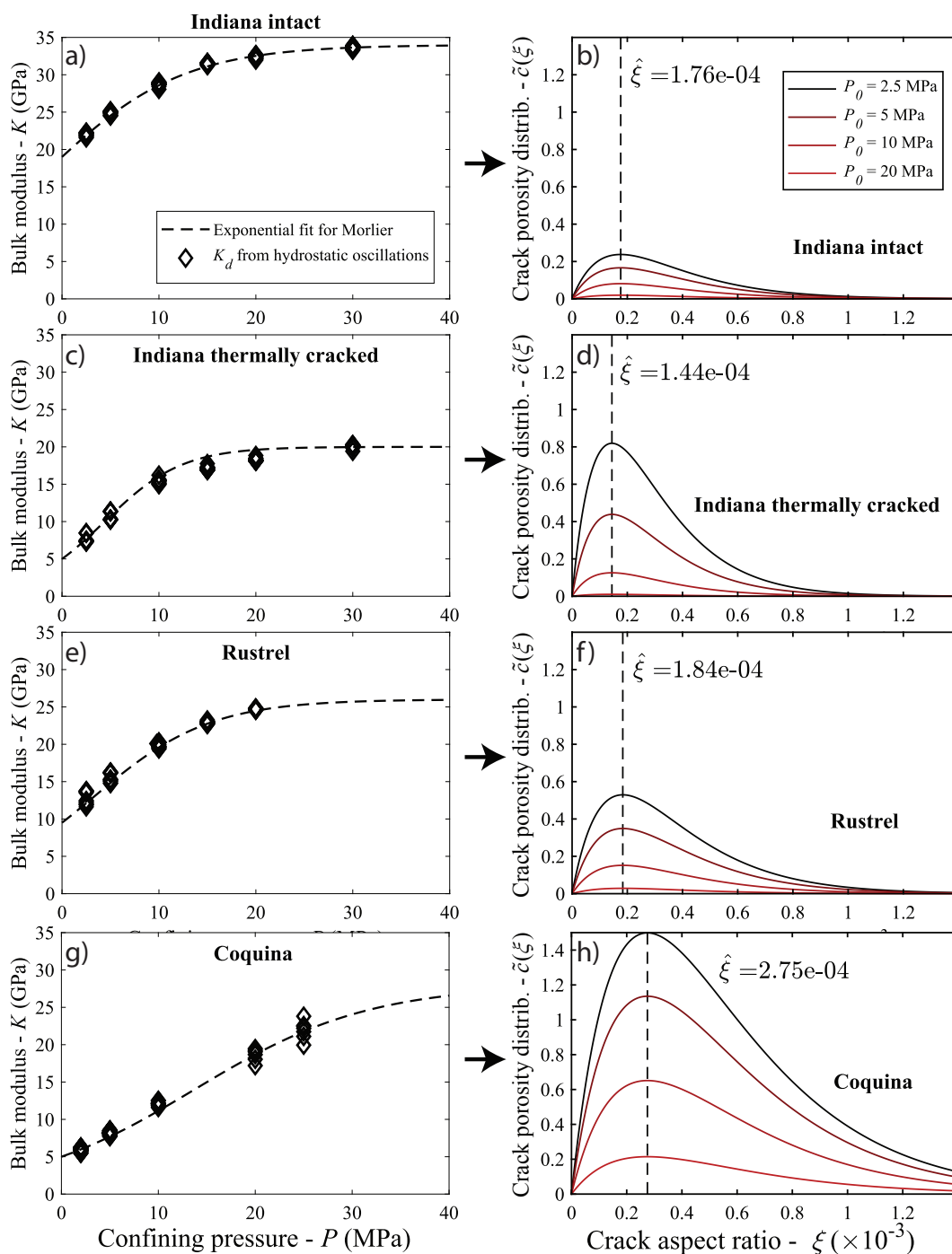
Figure 10.8: Pressure dependence of the bulk modulus and deduced crack distributions at different differential pressures for the intact Indiana (a-b), the thermally cracked Indiana (c-d), the Rustrel (e-f) and the Coquina samples (g-h). We use the pressure-dependence of the dynamic bulk modulus K_d obtained from hydrostatic oscillations in dry conditions to adjust the crack distributions with Morlier's method. For a given pressure, K_d is plotted for all the measured frequencies. The fitting parameters for each sample are presented Table 10.1.
