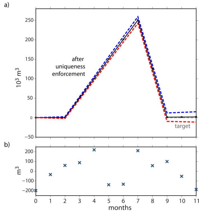
Fig. 4: Evolution of volume variation \Delta V along time for case 1b a) comparison of target volume variation (grey dotted line), modeled volume variation after flow correction (black plain line), upper and lower modeled volume variation at 2\text{-}\sigma uncertainties (blue and red dashed lines); b) residual volume equal to the difference between target and modeled volume with the linear trend removed for both solutions.
