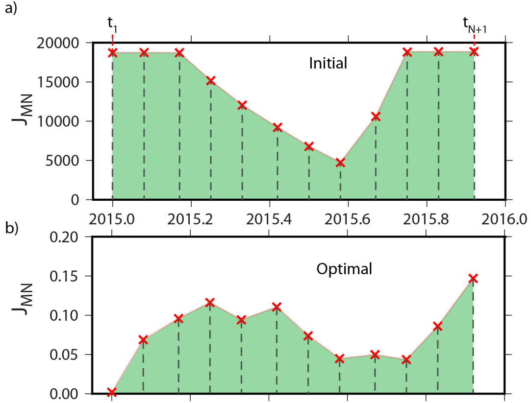
Figure 4.6: Construction of J_{MN} for one type of data and N = 12 time series, a) from the first iteration of the optimization to b) the optimal state. Note the difference in the vertical scale between a) and b).
