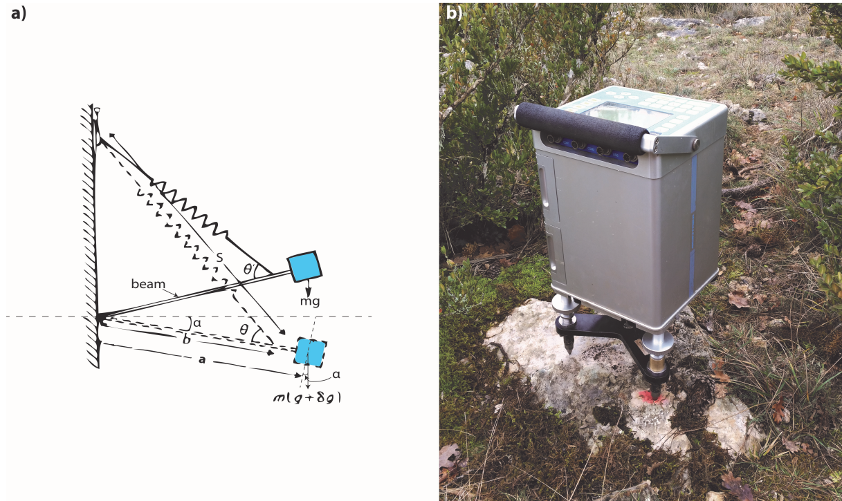
Figure 2.7: a) Principle of spring-base gravimeter. b) The CG5 relative gravimeter from Lacoste & Romberg.
