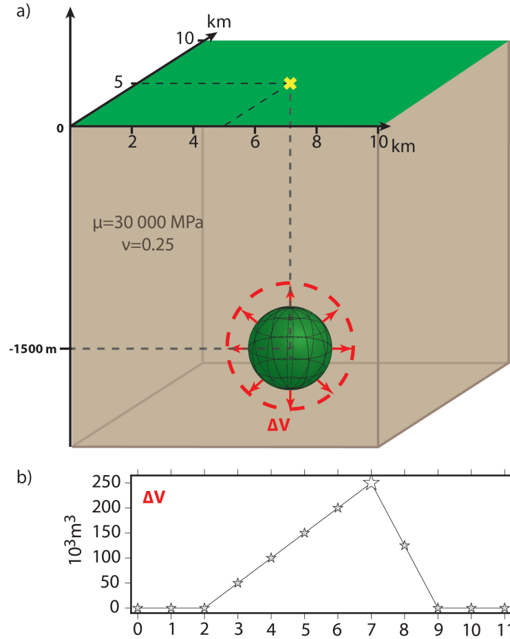
Figure 7.1: a) Configuration of the Mogi model with the source centered in a 10 km by 10 km domain. The sphere is embedded in a homogeneous, isotropic, elastic flat half space characterized by a shear modulus \mu=30\,000 \text{ MPa} and a Poisson's coefficient \nu=0.25 . b) History of volume variations of the source over 11 months of experiment.
