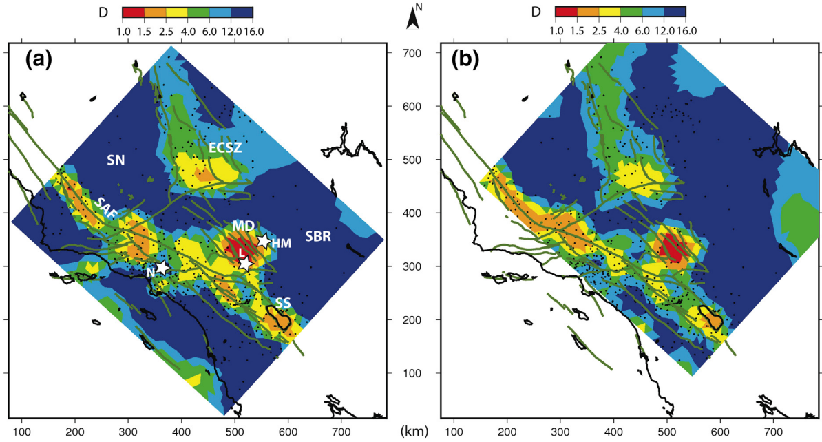
Fig. 8. Distributions of the relative rigidity D represented for Zone 1 (a) and for Zone 2 (b). According to Eq. (23), the elastic thickness T_e is proportional to D . The GPS data are represented by black dots, the faults by green lines and the Landers (L), Northridge (N) and Hector Mines (HM) earthquakes by white stars. SAF, SN, ECSZ, SBR, MD and SS stand for San Andreas Fault, Sierra Nevada, Eastern California Shear Zone, South Basin and Range, Mojave Desert and Salton Sea respectively. (For interpretation of the references to color in this figure legend, the reader is referred to the web version of this article.)
