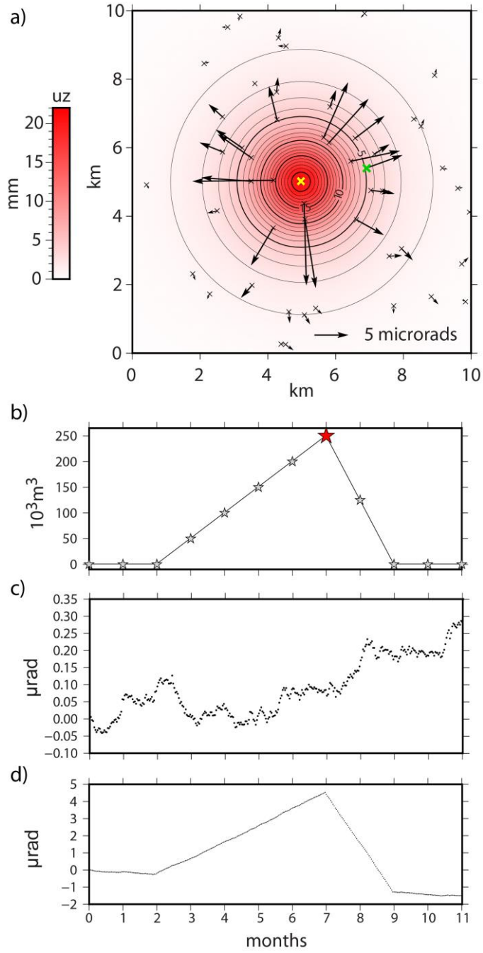
Fig. 1: Synthetic tilt produced by volumetric changes of a spherical source with an added drift of 2.4 \mu\text{rad/yr} and a Brownian noise, during 11 months of the experiment. a) Screenshot of the vertical displacement u_z (color scale) and tilt signal (black arrows) induced by a volumetric variation at t=7 ( \Delta V = 250\,000 \text{ m}^3 , red star on b) of a spherical source (yellow cross). b) Evolution of the targeted volumetric changes over one year c) Typical random walk noise associated to the tilt over 11 months d) Synthetic tilt signal with drift and noise in x-direction for one tiltmeter (green cross on Fig. 1a).
