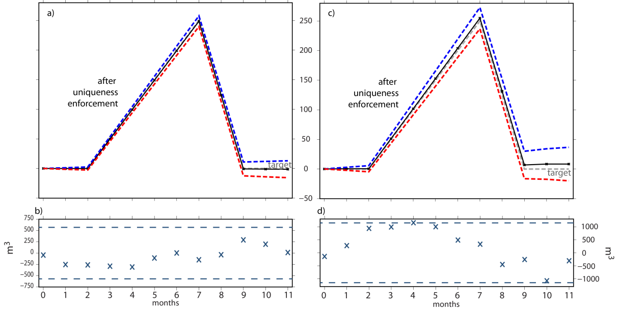
Figure 6.3: a) Comparison of target volume variations (grey dashed line), modeled volume variations after flow correction (black plain line), upper and lower modeled volume variations at 2- \sigma uncertainties (colored dashed lines); b) residual volume showing the difference between target and modeled volumes with the linear trend removed for both solutions. Blue dashed lines represent the volume resolutions \delta V estimated from Eq.11b.
