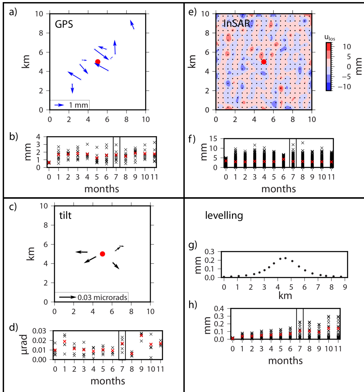
Figure 7.5: Spatial and temporal distributions of GPS (upper left), tilt (lower left), InSAR (upper right) and levelling (lower right) residuals. The source of deformation is indicated by a red dot on a), c) and e). a) Spatial distribution of the GPS residuals at time t=7 (rectangle on b). b) Temporal distribution of the GPS residuals and mean residual for each time series (red crosses). c) and d), e) and f), g) and h) represent the same as a) and b) for tilt, InSAR and levelling data respectively.
