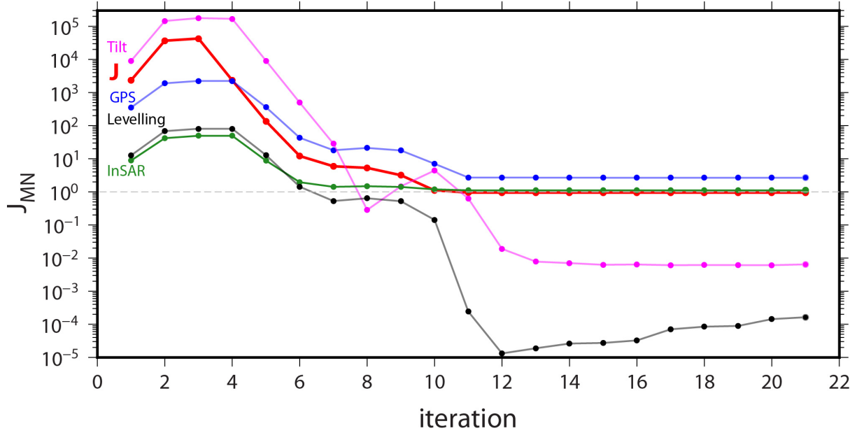
Figure 7.4: Convergence of individual J_{MNi} (blue curve for GPS, pink curve for tilt, green curve for InSAR and black curve for levelling) and global J (red curve) functionals. The global functional is built using the individual functionals, each one weighted by 0.25. The global minimum is reached at iteration 15.
