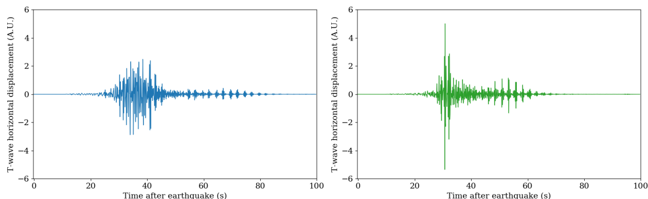
Figure 4.20 – T-wave horizontal displacement (after body wave subtraction) generated by the two earthquakes marked as blue and green circles in Figure 4.18. The green signal is more impulsive.
