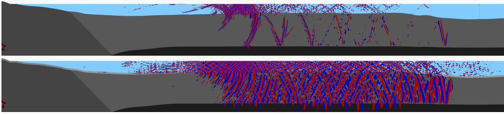
Figure 4.6 – Snapshots of the horizontal displacement field at time t = 40 s, showing the effect of the presence of sediments. Blue: negative horizontal displacement, red: positive horizontal displacement. The symmetry axis is at the left-hand side of the figures, and the source position is shown as a (partly cut) red star on the symmetry axis. Top: no sediments (case 3). Bottom: with sediments (case 1). The amplitude scales used in each case are different, the display being independently normalized to the maximum amplitude of a given figure.
