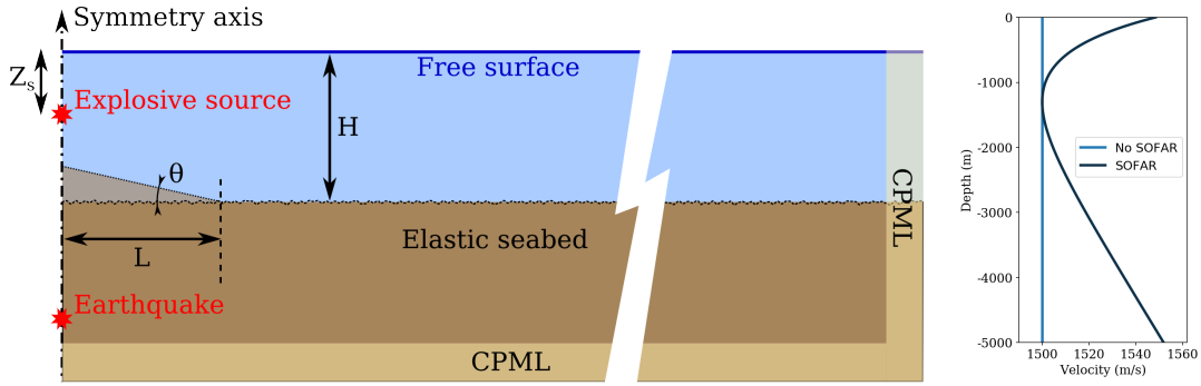
Figure 5.4 – Left: this picture depicts the simulations performed in this section. The setup is 2-D axisymmetric. The ocean depth is H = 5000 m. Right: sound speed profiles in the sea used for the numerical simulations. “SOFAR” means a classical idealized ocean sound-speed profile (Munk [1974]) with a minimum velocity set at depth 1300 m.
