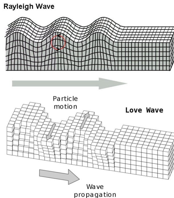
Figure G.1 – Comparison of Love and Rayleigh wave particle motions. Adapted from Wikipedia.
