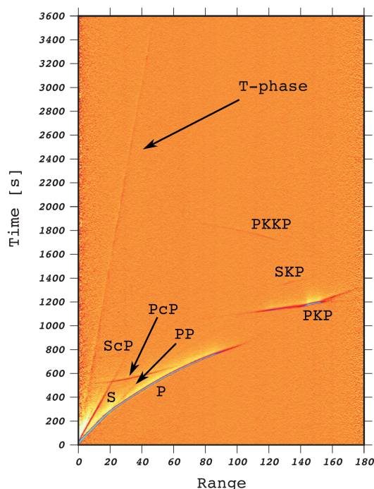
Figure 1.6 – Adapted from Buehler & Shearer [2015]. Global broadband STA/LTA seismogram stack with traces filtered at 2-8 Hz. See Figure G.2 on page 197 for a description of the seismic phases mentioned.
