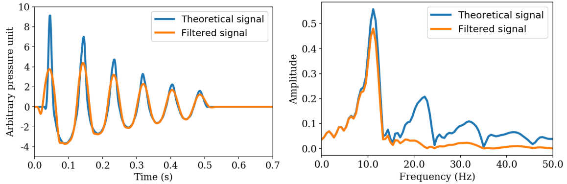
Figure A.4 – Comparison in the time (left) and frequency (Power Spectral Density, right) domains between the theoretical pressure signal generated from the source used (Coles et al. [1946]; Jones & Miller [1948]) and the pressure signal used in our simulations.
