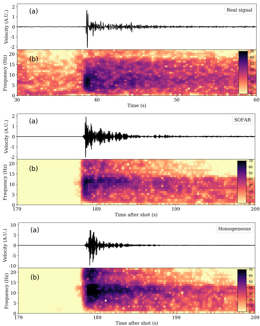
Figure A.5 – Comparison of the synthetic signals to the real one at station VAH. The top figure is the real signal (bandpass-filtered between 0.5 Hz and 25 Hz), and the middle and the bottom ones are the synthetic signals, respectively with and without a SOFAR channel. For the three pictures: (a) Seismogram of the vertical component of the velocity vector (arbitrary velocity unit). (b) Power Spectral Density (in dB) as a function of time and frequency. Note that the time of the shot is not known, consequently the time shown in the top figure is arbitrary. The amplitude of the synthetic signals can be compared.
