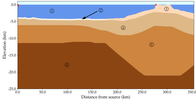
Figure A.2 – Setting of the 2.5-D experiment together with a realistic geological structure (extrapolated from Patriat et al. [2002]), to which we added the sedimentary layer discovered by Talandier & Okal [1987b]. The source is on the axis on the left hand side at depth 215 m. The velocity profile in the water is depicted in Figure A.3. Station VAH at which the wave field is recorded is shown as a small red triangle. The seismic properties of each domain are shown in Table A.1.
