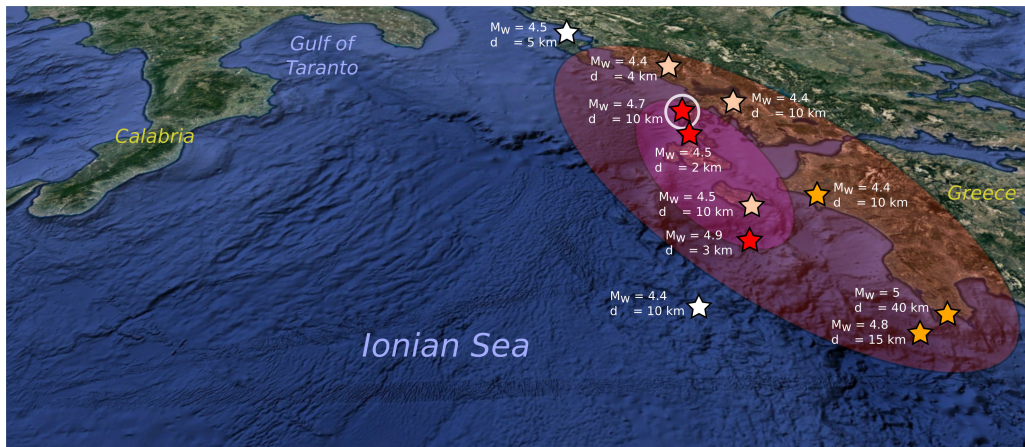
Figure 2.5 – For each earthquake indicated on the above map (star), both the characteristics from NOAA (magnitude and hypocenter depth d ) and the quality of the generated T-waves are detailed. The classification has been made from the same kind of map than the one presented in Figure 2.1. Red stars: more than 5 Italian stations have recorded strong T-phases ("red" stations), orange stars: some Italian stations have recorded strong T-phases, light orange stars: T-phases recorded by several Italian stations, white stars: no T-waves visible. Earthquakes occurring in the red area are prone to generate T-waves. Earthquakes occurring in the purple area are particularly prone to generate strong T-waves. That area corresponds to the Greek peninsula of Paliki. The circle indicates the earthquake shown above.
