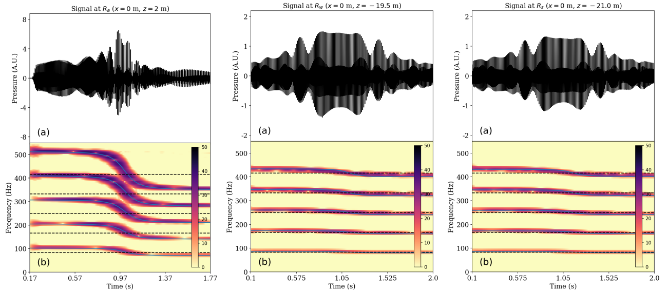
Figure 6.7 – Signal recorded at the three receivers R_a (left), R_w (middle) and R_s (right) shown in Figure 6.5. For each sub-figure: (a) Pressure seismogram (arbitrary pressure unit). Although arbitrary, the amplitude of the synthetic signals can be compared because the arbitrary scaling is the same in the linear wave equation. (b) Power Spectral Density (in dB) as a function of time and frequency. The black dashed lines refer to the frequencies of the harmonics emitted by the source. The blue curves represent the theoretical Doppler shifts expected, which are given by equation (6.28).
