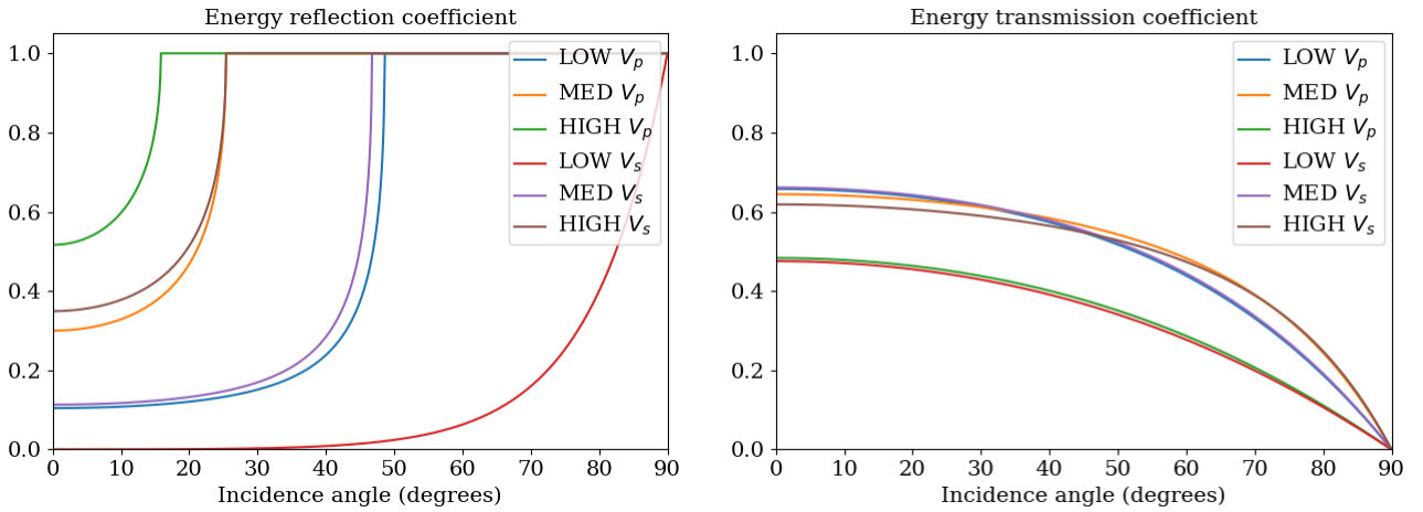
Figure 4.14 – Left: energy reflection coefficient for oceanic rays as a function of incidence angle (with respect to the normal to the interface) at the water-sediments interface. Right: semi-infinite bottom \rightarrow sediments \rightarrow water energy transmission coefficient as a function of incidence angle. “LOW V_s ” for example means that the sediment density is equal to that of the case labeled LOW in Table 4.2 and that the velocity corresponds to shear-wave velocity of case LOW.
