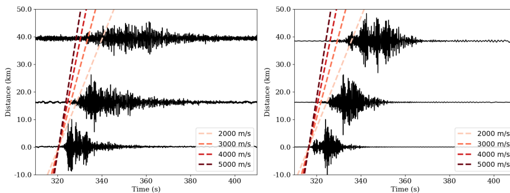
Figure 4.7 – Comparison between the observed inland T-wave speed for the synthetic (case 1) and real cases. The traces are the normalized north-south displacement seismograms at stations MEU, SSY and AGST, from top to bottom. The traces are distributed along the vertical direction according to the distance to station AGST of their projection on blue dotted line in Figure 2.1 (top). Left: real signals. Right: synthetic signals (configuration with a SOFAR channel, sediments, and a source depth of 10 km). The apparent velocity of the first real arrival is seen to be 4000 \pm 1000 m/s, while the apparent velocity of the first synthetic arrival is seen to be 3000 \pm 1000 m/s.
