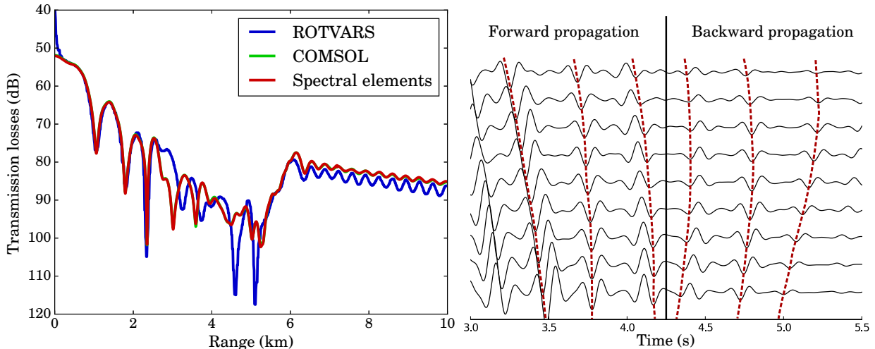
Figure 3.7 – Left: Transmission losses in dB as a function of range in km. The first curve has been calculated with ROTVARS, the second with COMSOL (both taken and adapted from Jensen et al. [2007], Fig. 7), and the third with the spectral-element method. Note that the COMSOL and spectral-element results are almost perfectly superimposed. Right: Pressure time series recorded by the receivers of the horizontal antenna ( z = -250 m) shown in Figure 3.5. The upper trace is the pressure recorded by the receiver located at r = 2 km, the lower trace is the pressure recorded by the receiver located at r = 3 km. In the left part of the picture ( t < 4.25 s) the noticeable arrivals are recorded first at the leftmost receivers, thus corresponding to forward energy propagation. In the right part of the picture ( t > 4.25 s) the noticeable arrivals are recorded first at the rightmost receivers, thus corresponding to significant backward energy propagation (which cannot be computed by parabolic equation techniques for instance).
