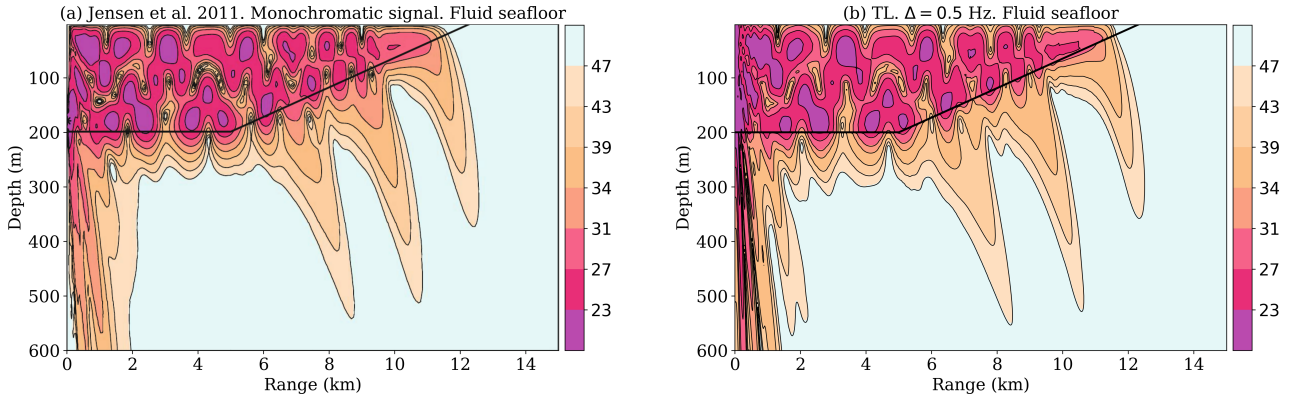
Figure 5.1 – (a) Original TL map, in dB, from reference Jensen et al. [2011] page 514. (b) TL map from a full-wave time-domain simulation using an quasi-monochromatic source ( f_0 = 25 Hz, \Delta = 0.5 Hz). Figure (a) is reproduced (slightly modified) from Figure 6.11 of Jensen et al. [2011] with permission from publisher Springer. The black line indicates the seabed interface.
