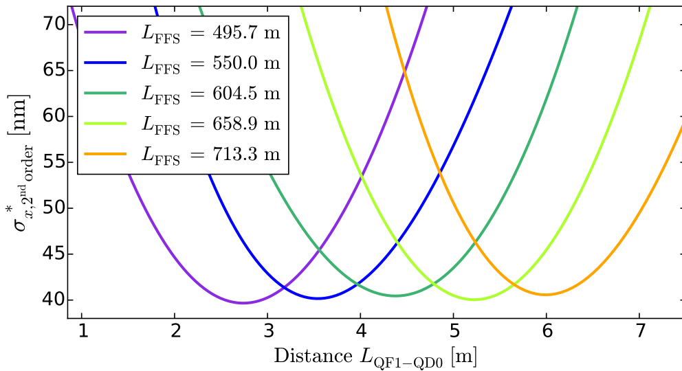
Figure 4.4: Parabolic fits of the L_{\text{QF1-QD0}} scan for different FFS lengths.
