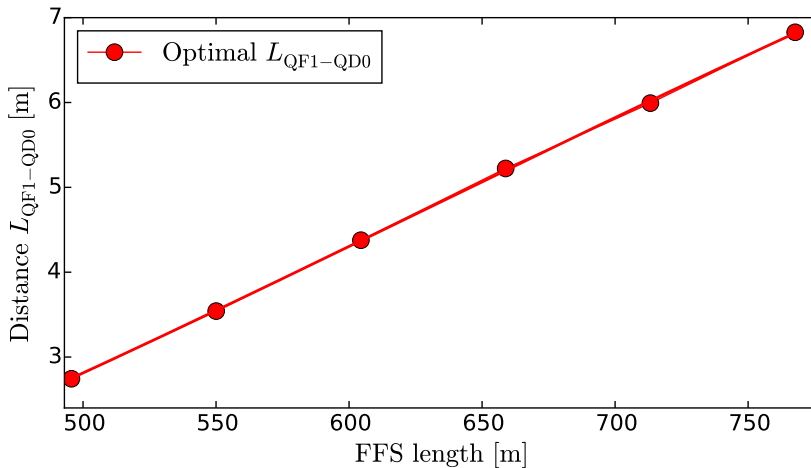
Figure 4.5: Optimal distance L_{\text{QF1-QD0}} for \sigma_{x,2^{\text{nd}}\text{order}}^* minimization as function of the FFS length.
