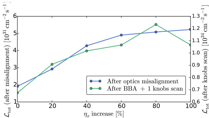
Figure 5.22: Average luminosity, over 100 randomly misaligned machines (see Table 5.5), after applying errors and after one tuning iteration, as function of FFS dispersion increase.
