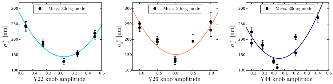
Figure 6.26: Examples of 2 nd order knob scans (using the 4 skew sextupoles) where Y 22 corresponds to T_{yx'x'} , Y 26 corresponds to T_{yx'\delta} and Y 44 corresponds to T_{yy'y'}
