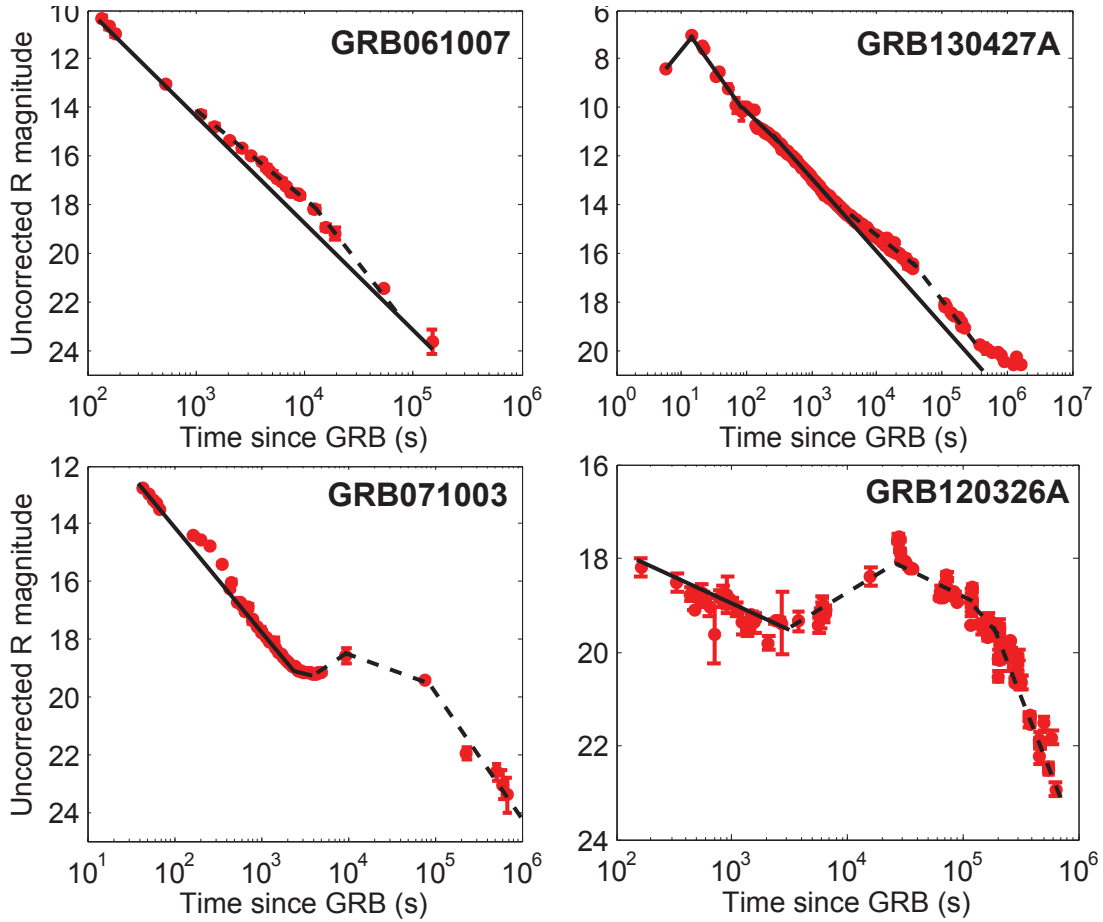
Figure 5.20.: Examples of the two types of late rebrightening (LR) observed in the optical light curves of GRB afterglows (dashed lines). Top: The LRs appear as a smooth bump superimposed to the standard fading optical emission of GRB 061007 and GRB 130427A. For this kind of LR a late-time energy injection process is often invoked as an explanation. Bottom: A dramatic increase of optical flux is observed in the afterglow light curve of GRB 071003 and GRB 120326A. For this kind of LR the refreshed shock scenario or geometrical effects (jet with multiple components, jet seen off-axis) are used to explain these features.
