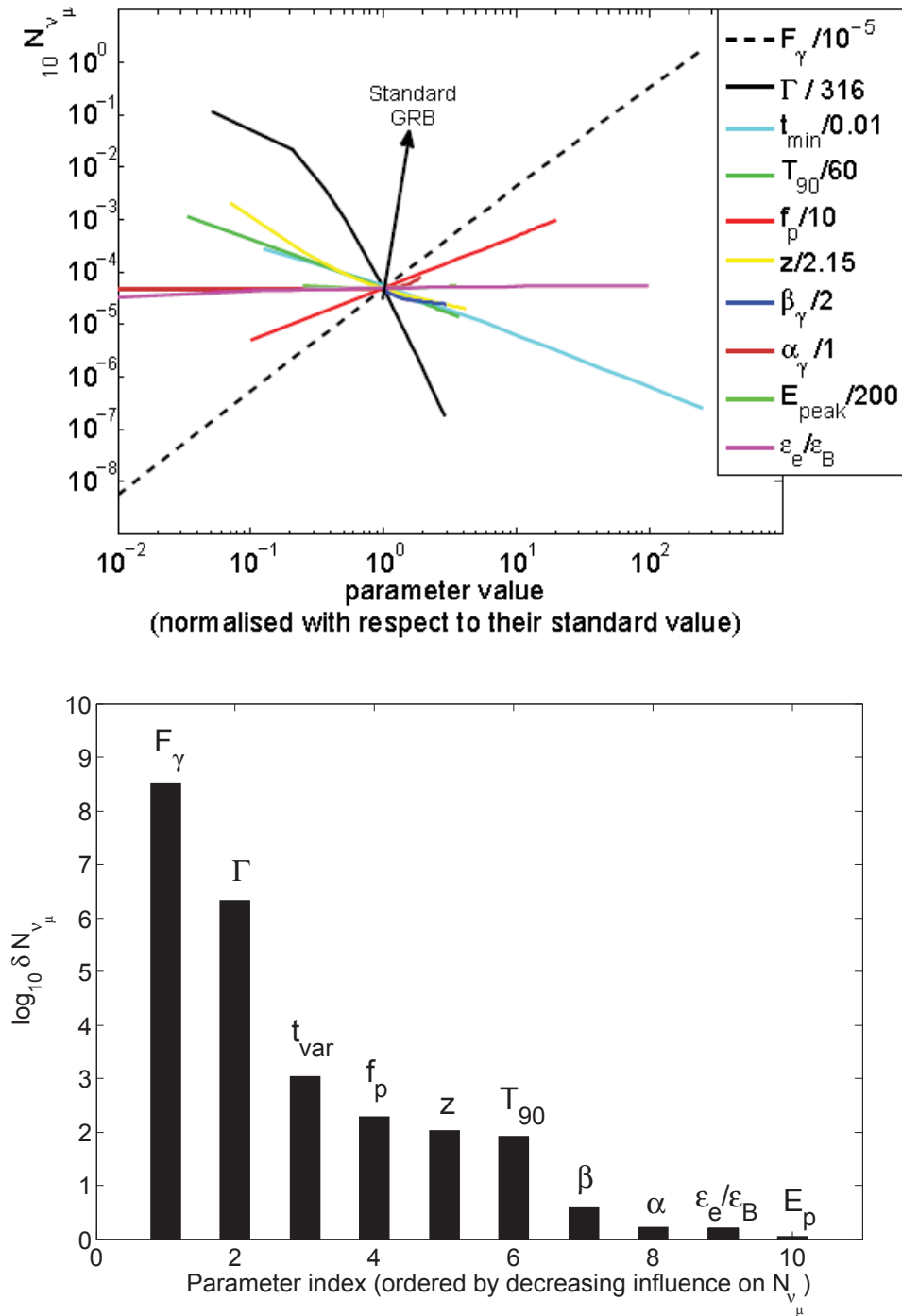
Figure 8.17.: ( Top ) Evolution of the expected number of neutrinos as a function of the normalized parameter values. ( Bottom ) Histogram of the relative amplitude \delta N_\mu with respect to each input parameter. The parameters are ordered according to their impact on the neutrino predictions.
