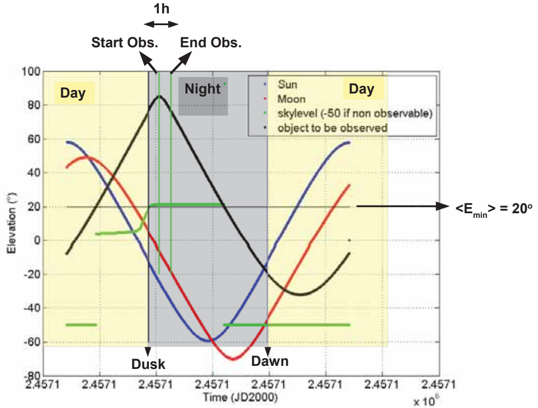
Figure 9.10.: Illustration of the observational strategy applied to the follow-up of the TAToO alerts with the TAROT/Zadko telescopes. The simulation is running for 24 hrs centered on the full night time (black area) at the Zadko site. The TAToO alert is received during the daytime before the night (dusk). The black, blue, red lines represent the elevation the neutrino candidate, the Sun and the Moon as function of time. The skylight level is shown in green. We are in the case where the object is rising when the night starts and setting few hours after ( Type III ). The observations start as soon as possible avoiding the first 30 minutes after the dusk to maximise the sky level and hence to have the best image quality. The alert field is followed-up during one hour.
