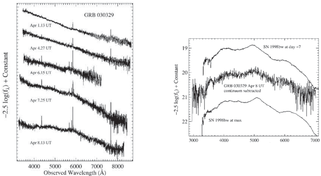
Figure 4.11.: (Left) Evolution of the optical spectrum of GRB 030329-SN 2003dh. Later spectra show broad peaks characteristics of a supernovae (Right) Spectra of SN 2003dh taken on 2003 April, 8, with continuum subtraction. (Both) Figure extracted from (Stanek et al. 2003).
