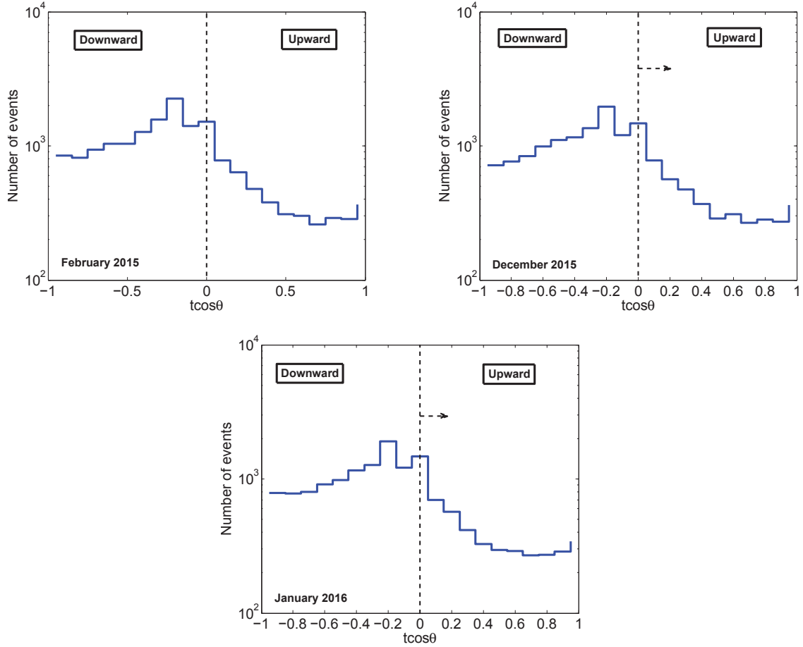
Figure 11.2.: Distribution of the zenith angle ( t \cos \theta ) for the events that passed the on-line quality cuts during the months where the four FRBs were detected. No track-fit quality cut ( \Lambda ) has been applied on the data set shown here. The arrow shows the selection criteria t \cos \theta > 0 .
