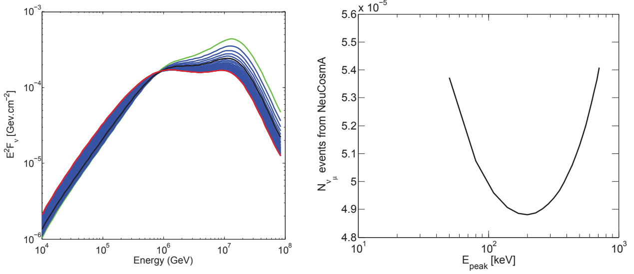
Figure 8.10.: (Left) NeuCosmA spectra ( \nu_\mu + \bar{\nu}_\mu ) for a standard GRB with E_{peak} \in [10 (green) \rightarrow 200 (black) \rightarrow 1000 (red)] keV. Spectra in red, black and green corresponds to the best, the worst and the standard neutrino prediction, respectively. (Right) Evolution of the expected number of neutrinos as a function of E_{peak} for a standard GRB.
