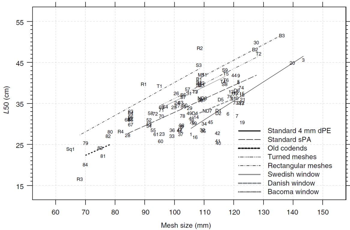
Figure S5.2. Relationship between selectivity parameters and mesh size for cod, estimated from linear regression in the Baltic cod fishery. (source; Madsen, 2007).
