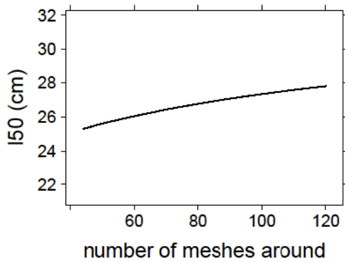
Figure S5.1. The dependence of plaice L50 on codend mesh size, twine diameter and number of meshes around the circumference, estimated from a statistical model based on meta-analysis data. (source; O'Neill and Noble, 2017).
