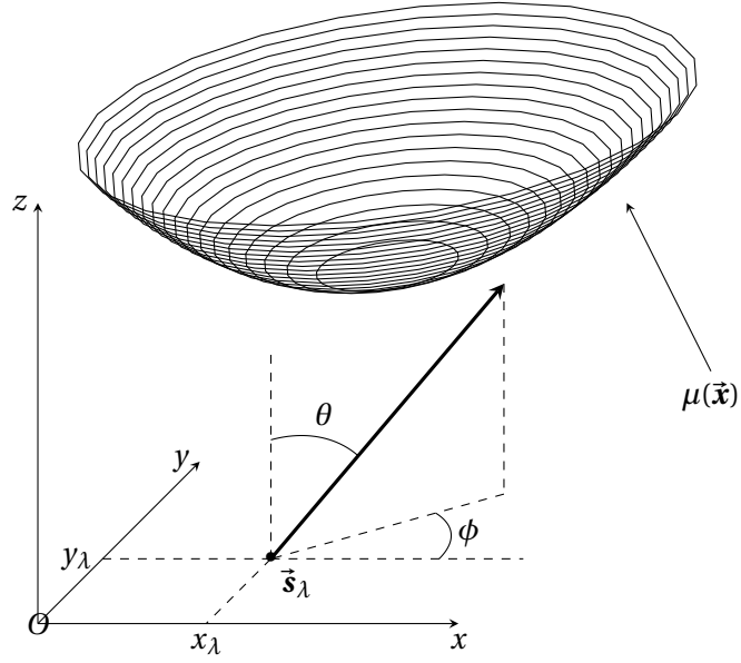
Figure 18: Cone-beam projections acquired from a source in a plane. The source is displaced in the plane z = 0 . One ray is identified with the unit vector \tilde{\mathbf{a}} with spherical coordinates (\theta, \phi) such that \tilde{\mathbf{a}} = (\cos \phi \sin \theta, \sin \phi \sin \theta, \cos \theta) .
