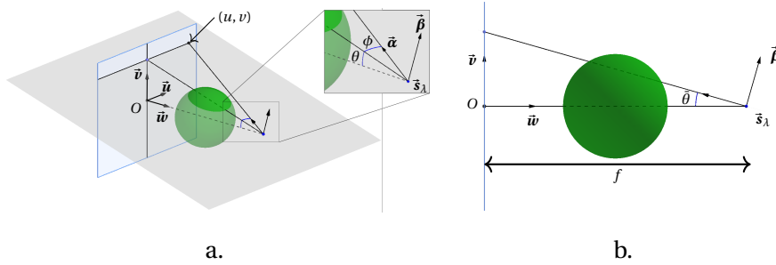
Figure 21: a. Left: The 3D Detector coordinate system. a. Right: the spherical coordinates of the vector \vec{\alpha} . Note the unusual orientation: the polar axis is horizontal. The vector \vec{\beta} has spherical coordinates (\bar{\beta}, 0) . b. View of the u = 0 plane.
