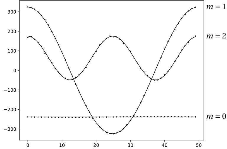
Figure 28: The function \tilde{G}_m(\lambda) for m = 0, 1, 2 for 50 projections, equally-spaced over a 360^\circ scan. The black solid line is a trigonometric polynomial, which best fits the data in a least-squares sense.
