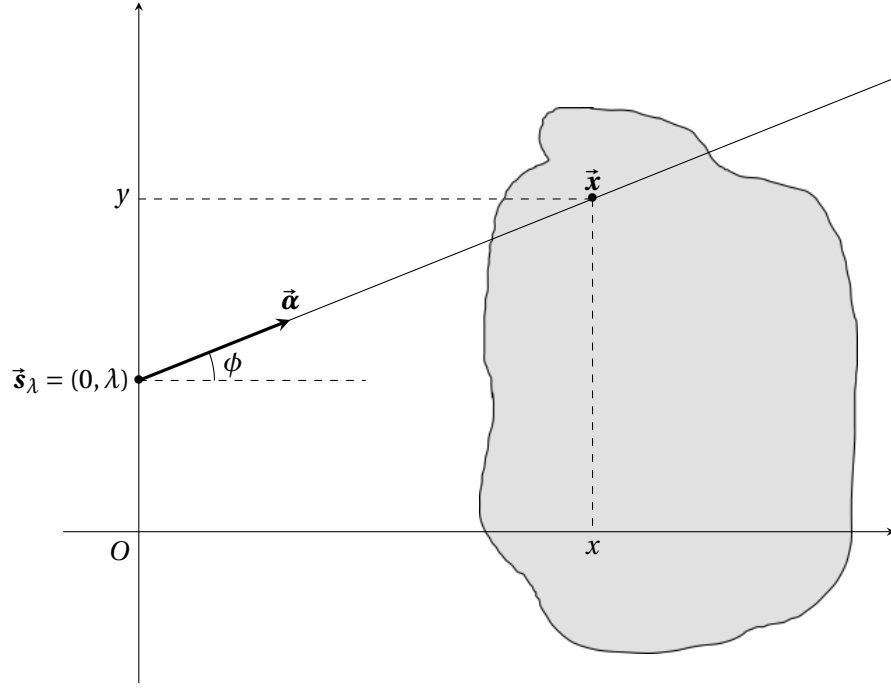
Figure 17: Fan-beam projections acquired along a line. The source is displaced on the vertical line x = 0 . One ray is identified with the unit vector \vec{a} or equivalently by the angle \phi it makes with the horizontal axis ( Ox ).
