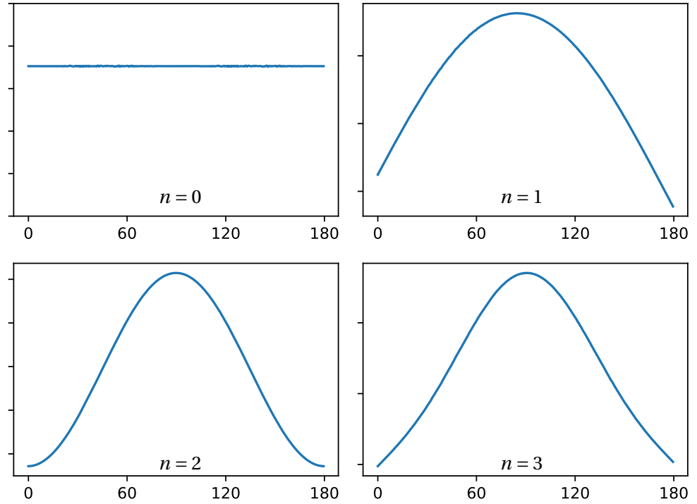
Figure 14: The Helgason-Ludwig consistency conditions. For each m = 0, 1, 2, 3 , the corresponding figure plots the moments J_m(\phi) . The trigonometric nature of J_m appears for each m . Note though that for the case m = 0 , whether J_0 is a constant or not very much depends on the y -scale of the graphic.
