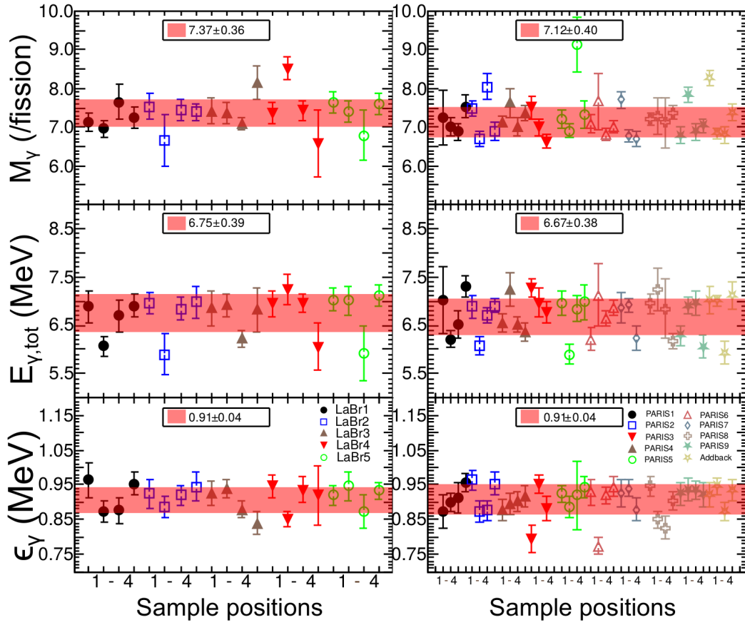
Figure B.3 – Spectral characteristics for each individual \gamma detector for LaBr 3 (left) and PARIS phoswich (right), respectively, in case of ^{239}\text{Pu}(n,f) at E_n 1.8 MeV.
