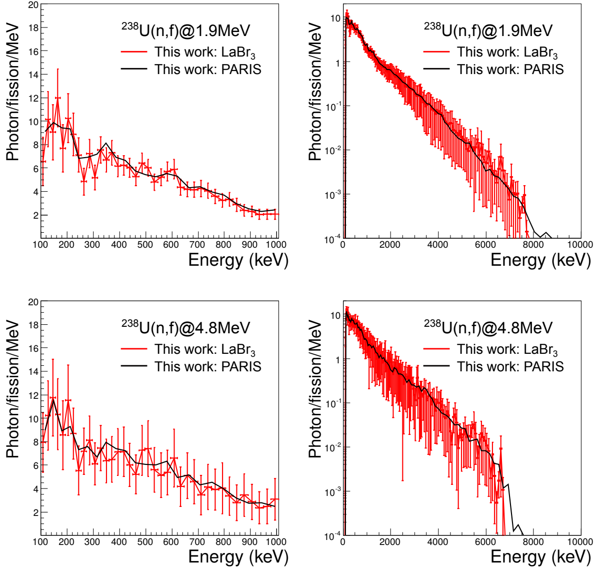
Figure 4.22 – Summed unfolded PFGS of ^{238}\text{U}(n,f) for LaBr 3 and PARIS phoswich, respectively, at E_n=1.9 and 4.8 MeV.
