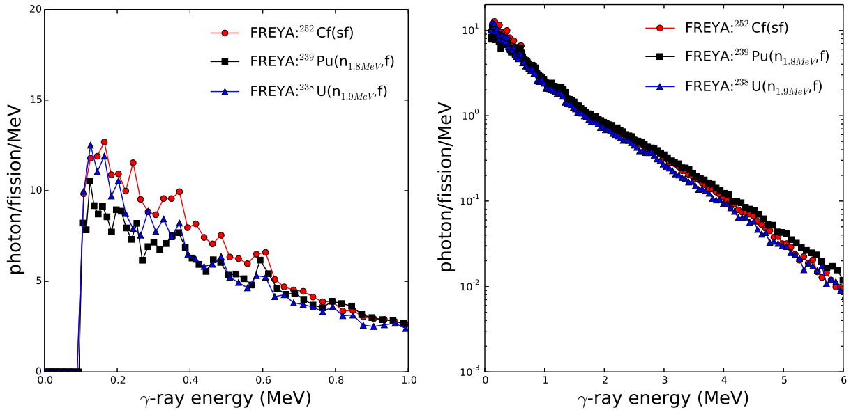
Figure 5.4 – Calculated prompt fission \gamma -ray spectra in FREYA code for different fission reactions: ^{252}\text{Cf}(\text{sf}) , ^{239}\text{Pu}(n_{1.8\text{MeV}},f) and ^{238}\text{U}(n_{1.9\text{MeV}},f) , respectively.
