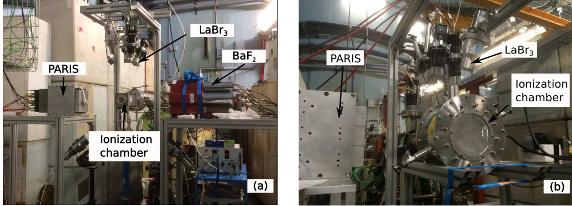
Figure 3.1 – Picture of the two experimental setups, dedicated to measure the PFG of the (a) ^{238}\text{U}(\text{n}_{\text{fast}},\text{f}) and (b) ^{239}\text{Pu}(\text{n}_{\text{fast}},\text{f}) reactions, respectively.
