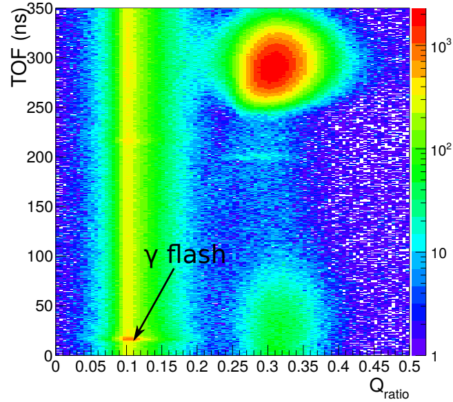
Figure 3.16 – Correlation between TOF and charge ratio in the n/γ discrimination. The γ flash originates from neutron inelastic scattering in coincidence with the beam pulse, which is perfectly known (16.67 ns for a detector placed at 5 m for example) and provides opportunity for the correction of the constant time offset.
