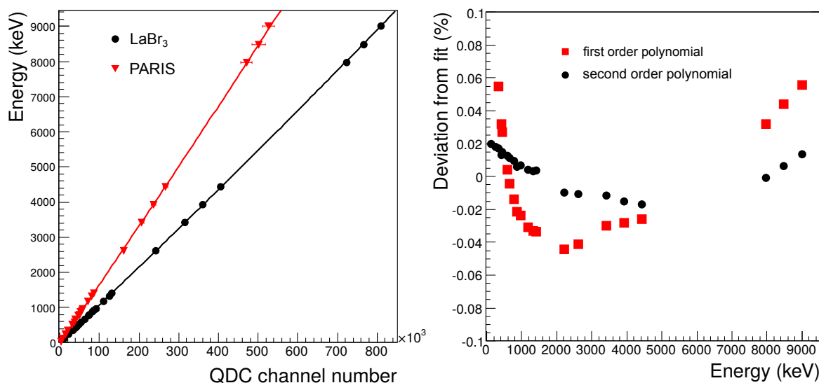
Figure 4.5 – (a) Energy response of the scintillation detector LaBr 3 and phoswich detector PARIS, respectively, i.e. correlation between \gamma -ray energy and QDC channel number; (b) Relative residuals of the linear fit to the experimental data of one LaBr 3 detector in the energy range from 0.1 MeV to 9.0 MeV.
