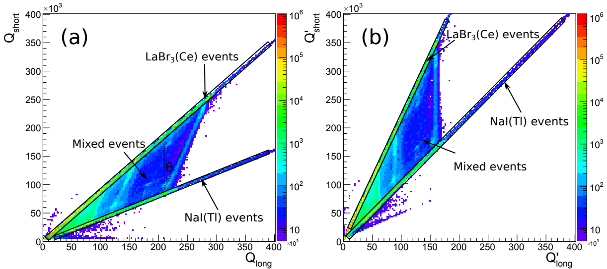
Figure 4.1 – Correlation between Q_{\text{short}} and Q_{\text{long}} before and after rotation. Q_{\text{short}} and Q_{\text{long}} represent the integrated charge over the short and long time gates, respectively. A clear discrimination of different events in a PARIS phoswich crystal can be achieved.
