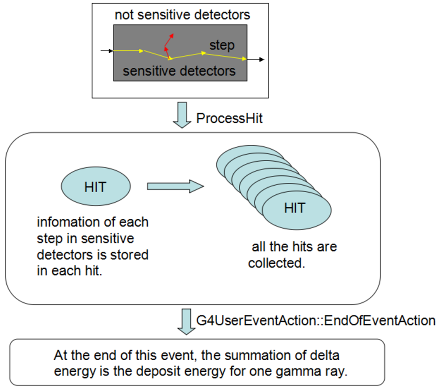
Figure 4.15 – Schematic view of the simulation process in G4VSensitiveDetector of GEANT4.
