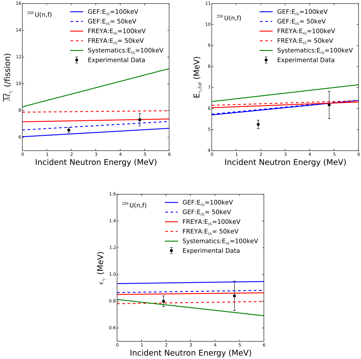
Figure 5.21 – Summary of the PFGS characteristics including average multiplicity \overline{M}_\gamma , average total energy E_{\gamma,tot} and average \gamma -ray energy \epsilon_\gamma , as a function of incident neutron energy, for fast-neutron induced fission of ^{238}\text{U} .
