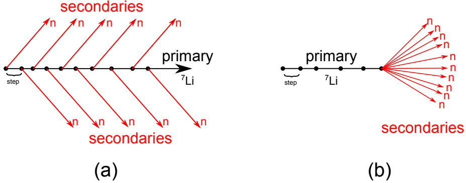
Figure 2.6 – Schematic view of the principle of multi-level splitting techniques applied in GEANT4: (a) force collision; (b) secondaries splitting.
