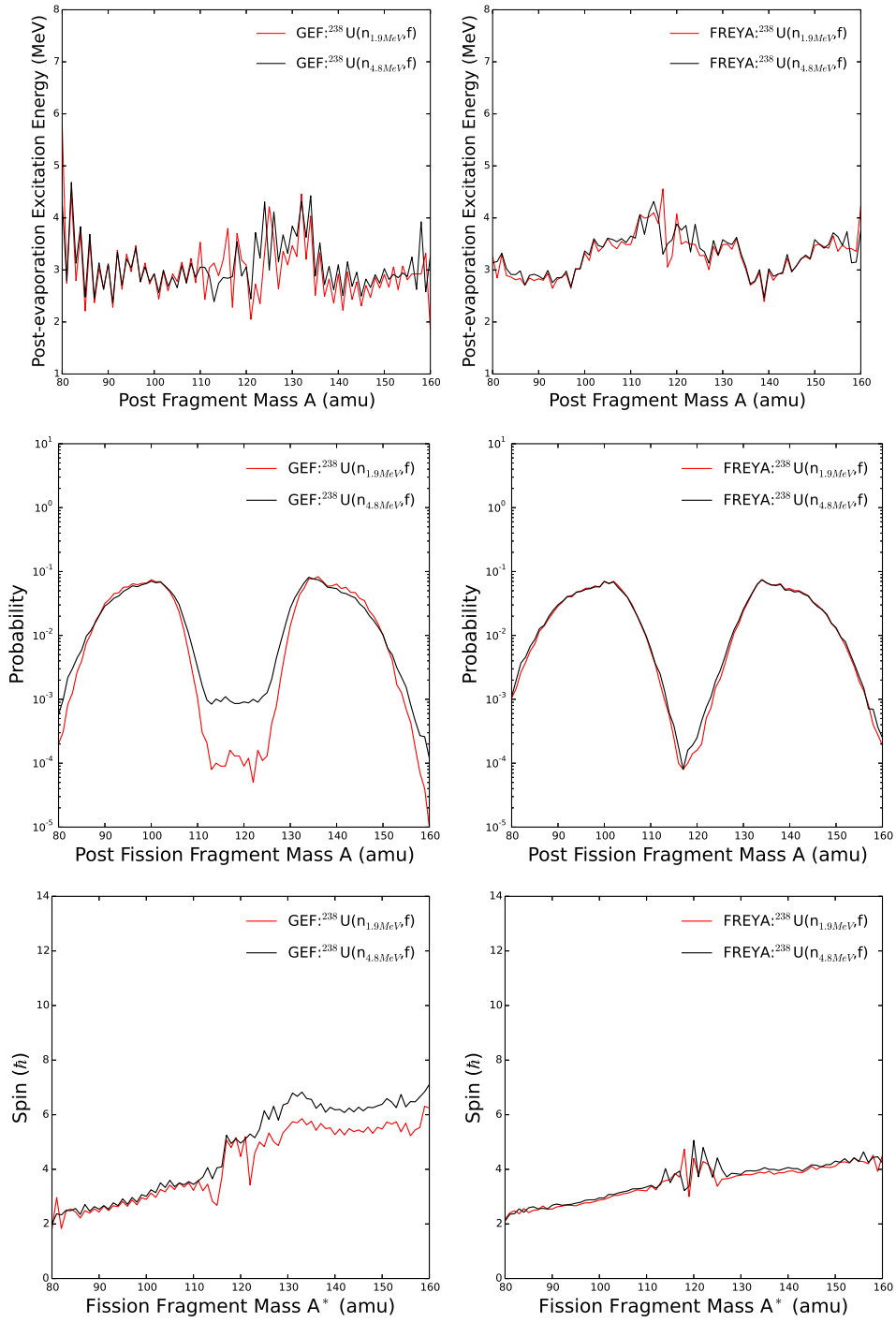
Figure 5.20 – Post-evaporation excitation energy, post-evaporation mass distribution and initial angular momentum distribution at neutron incident energy E_n = 1.9\text{ MeV} and E_n = 4.8\text{ MeV} , respectively, for the GEF (left) and FREYA (right) calculations.
