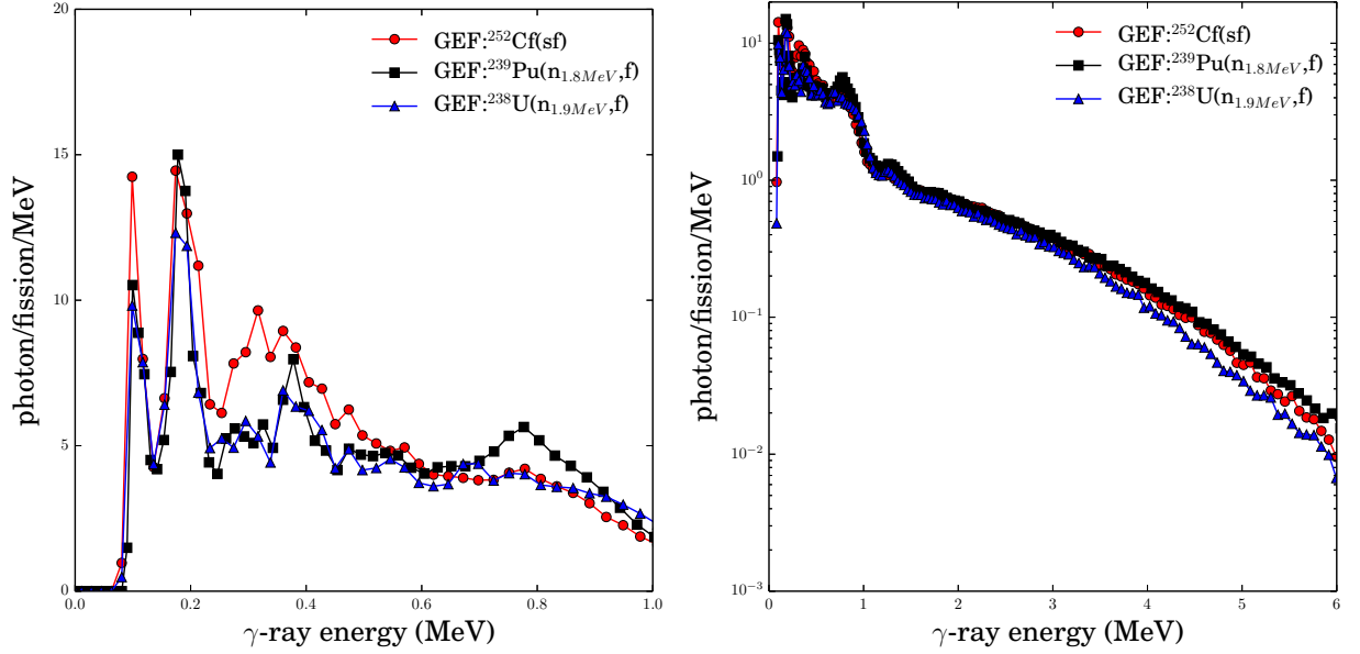
Figure 5.3 – Calculated prompt fission \gamma -ray spectra in GEF code for different fission reactions: ^{252}\text{Cf}(\text{sf}) , ^{239}\text{Pu}(n_{1.8\text{MeV}},f) and ^{238}\text{U}(n_{1.9\text{MeV}},f) , respectively.
