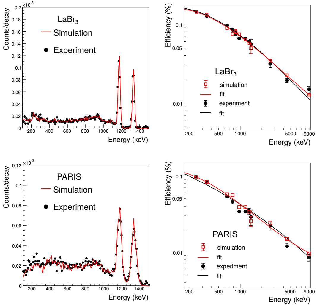
Figure 4.17 – Comparisons of the simulated and experimental \gamma -ray spectrum in the presence of ^{60}\text{Co} radioactive source for one \text{LaBr}_3 detector and one single PARIS phoswich, respectively (left); Comparisons of full-energy detection efficiency for simulation and experiments respectively, in energy range from 0.1 MeV to 9.0 MeV (right).
