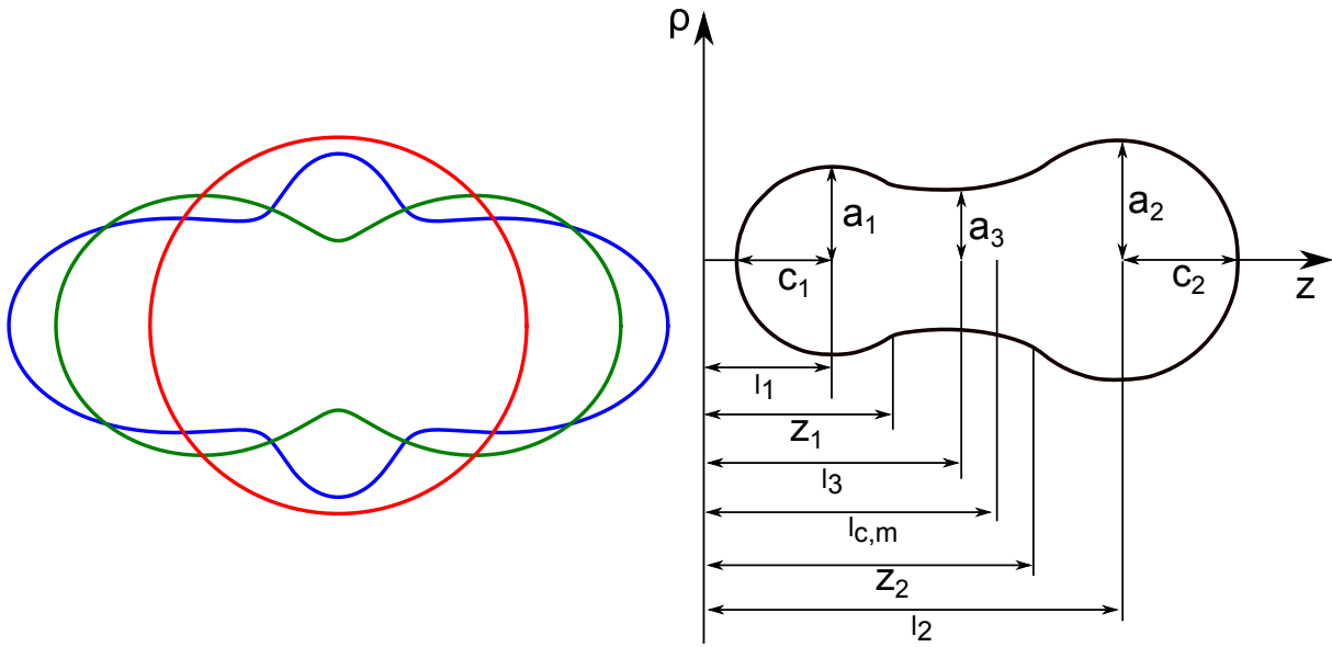
Figure 1.2 – (a) Contour plots of spheres with different kinds of deformation: no (red), quadrupolar (green) and octupolar (blue) deformation, with an expansion over the Legendre polynomials R(\mu) = \lambda R_0(1 + a_2 P_2(\mu) + a_4 P_4(\mu)) . (b) The three-quadratic-surface parameterization in representing the nuclear shape for the tabulation of macroscopic-microscopic potential energy surface (PES) [36].
