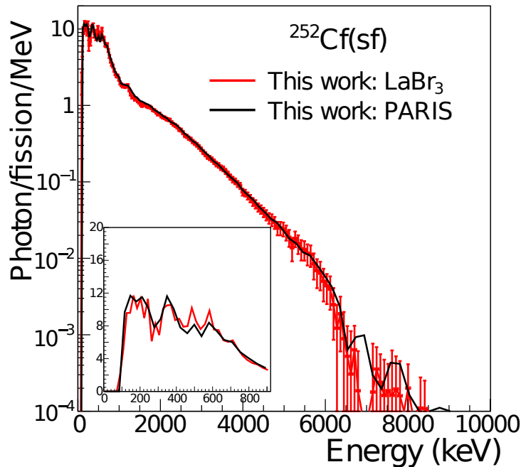
Figure 4.14 – Unfolded spectra with the time window \pm 2.5 ns from ^{252}\text{Cf(sf)} in logarithmic scale as obtained for two different types of gamma detectors (see text for details). The inset shows the region below 900 keV in linear scale.
