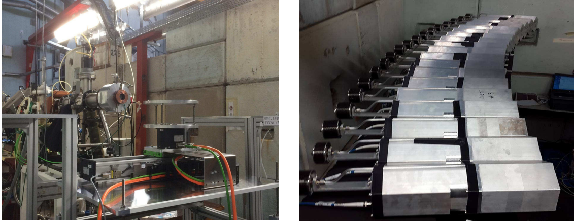
Figure 2.15 – Experimental setup of fast neutron tomography by using LICORNE neutron source, including a scanning table (left) and a neutron detection array NEDA (right).
