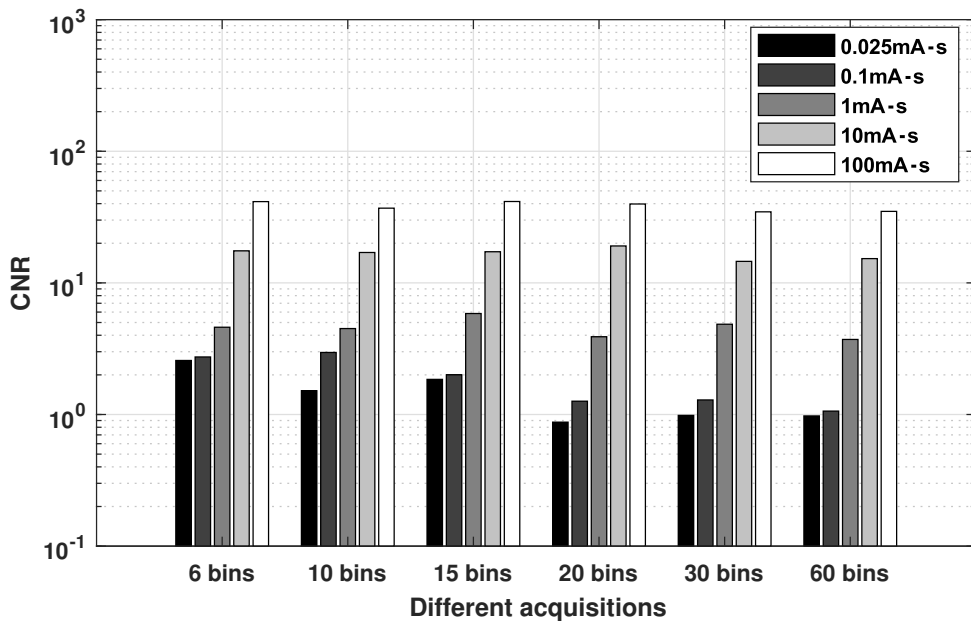
Figure 5.9: CNRs of decomposed iron images for 100 mg/cc of iron with different acquisitions using proj-PR-LLS method. Each group of acquisitions has the same number of energy bins but different exposure factors.
