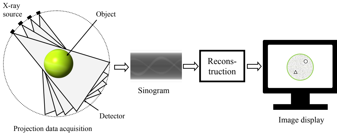
Figure 2.8: The mechanics of CT imaging: cross sectional image is reconstructed from projection data measured from multiple angles.
