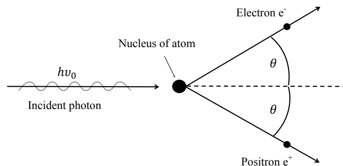
Figure 2.5: The mechanism of pair production: incident photon is annihilated, an electron-positron pair is generated. Figure is inspired by [Barrett and Swindell, 1996].
