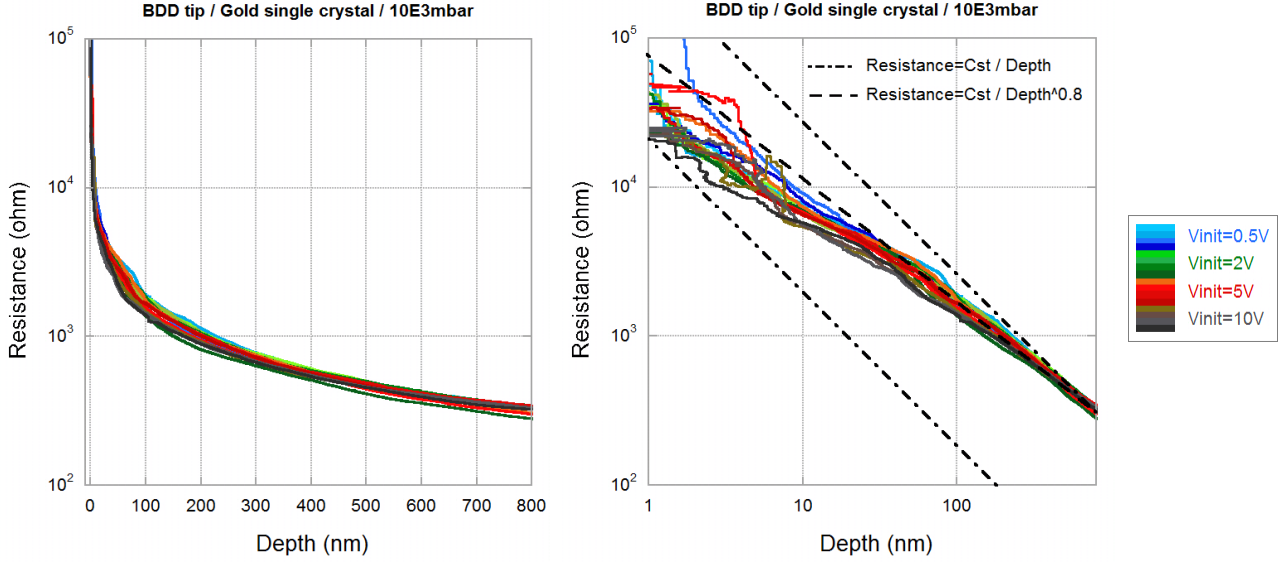
Figure 6.2: Resistance-versus-depth curve for BDD tip and bulk Au single crystal, with decimal scale (left) and logarithm scale (right).
