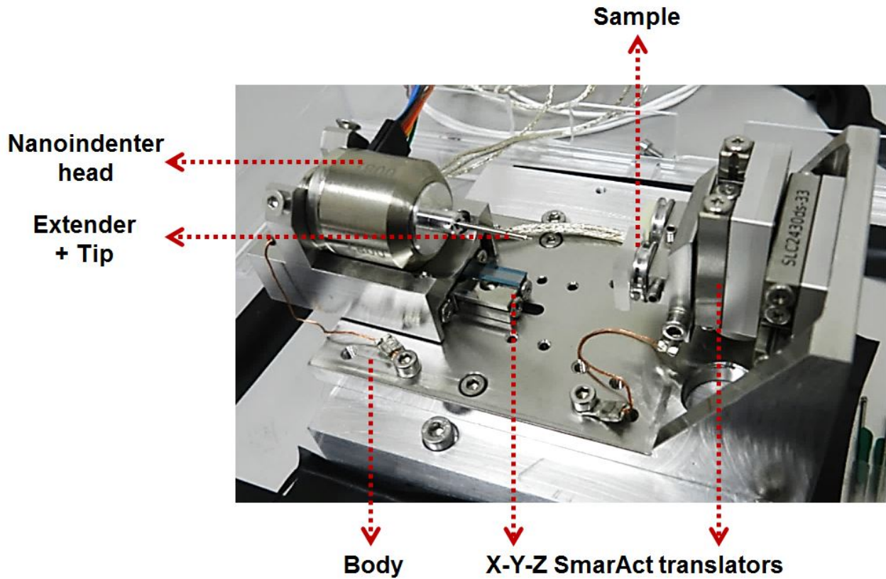
Figure 3.4: 3-axes set-up.
