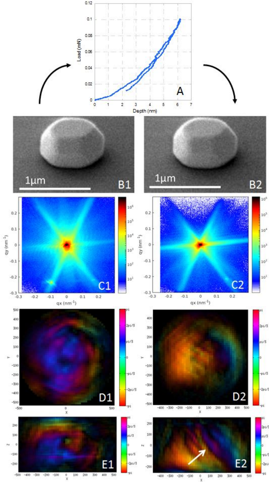
Figure 5.27: Force-versus-displacement curve during nanocompression of a gold single crystal (A), SEM image of the crystal (B), reciprocal space projection (C) and real space reconstruction parallel to the substrate (D) and normal to the substrate (E), before (left) and after (right) mechanical loading.
