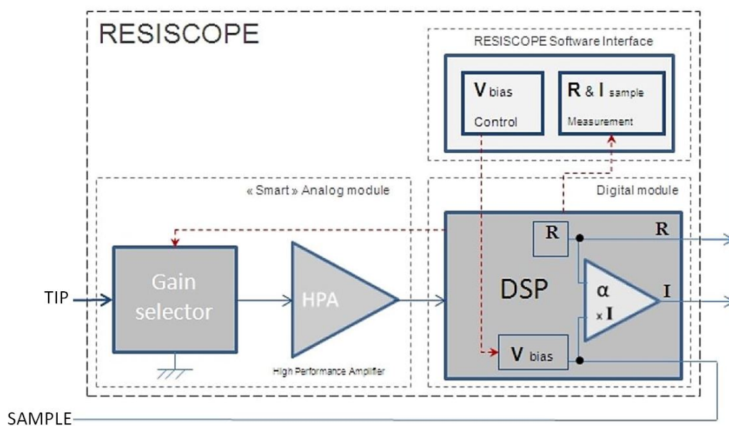
Figure 3.29: Digital module and analgo module of the ResiScope.
