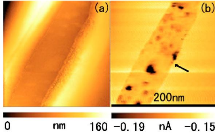
Figure 2.17: Conductive AFM topography map (a) and corresponding current map, showing the presence of "Dark spots" on a 4 nm SiO 2 area. From Sun et al. [119]
