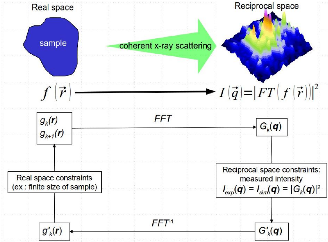
Figure C.3: Schematic of phase-retrieval algorithms, from Dupraz [189].
