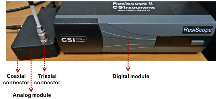
Figure 3.29: Digital module and analgo module of the ResiScope.
