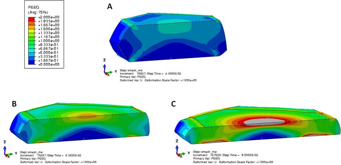
Figure D.3: Deformed shape of the island at increasing levels of compression \epsilon = \frac{\Delta h}{h_0} , in the case of a a island pinned at the bottom surface. A mapping of the equivalent plastic strain has been superimposed: (A) \epsilon = 26.5 %, (B) \epsilon = 52.3 % and (C) \epsilon = 67.3 %.
