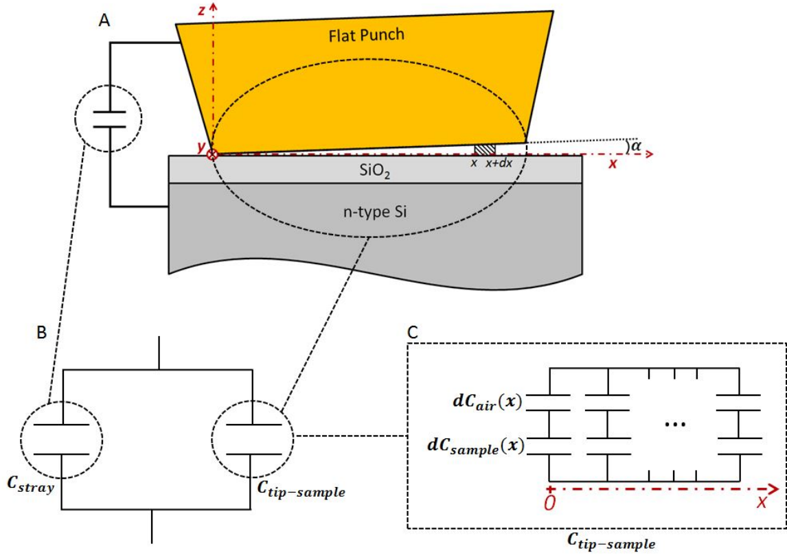
Figure 7.18: Schematic of the misalignment between the flat punch and the sample surface (A) and electrical diagram corresponding to the measured capacitance C_{\text{measured}} (B) and the tip-to-sample capacitance C_{\text{tip-sample}} (C).
