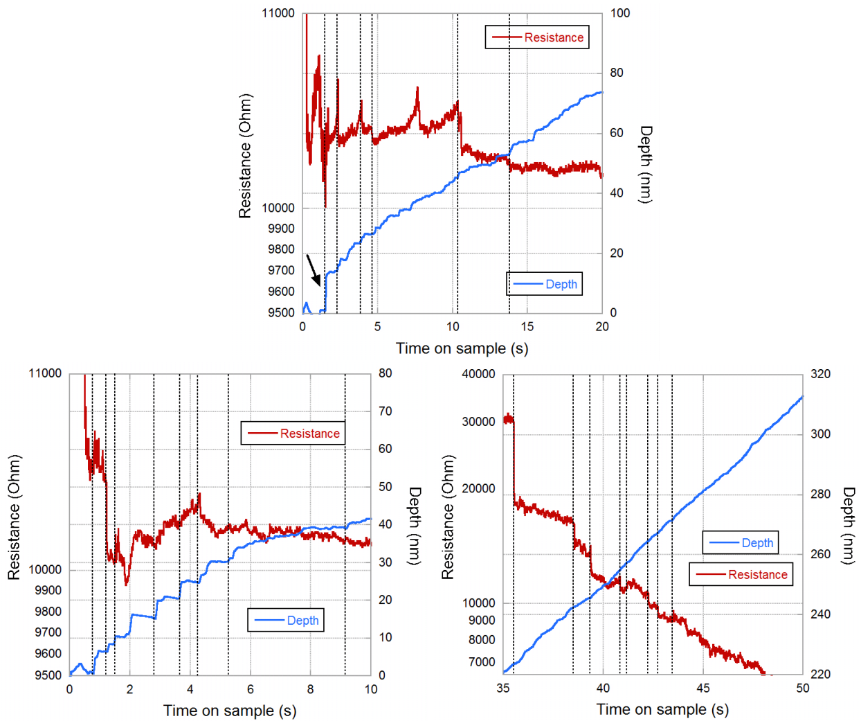
Figure 6.30: Correlation between mechanical events and electrical events (dotted lines).
