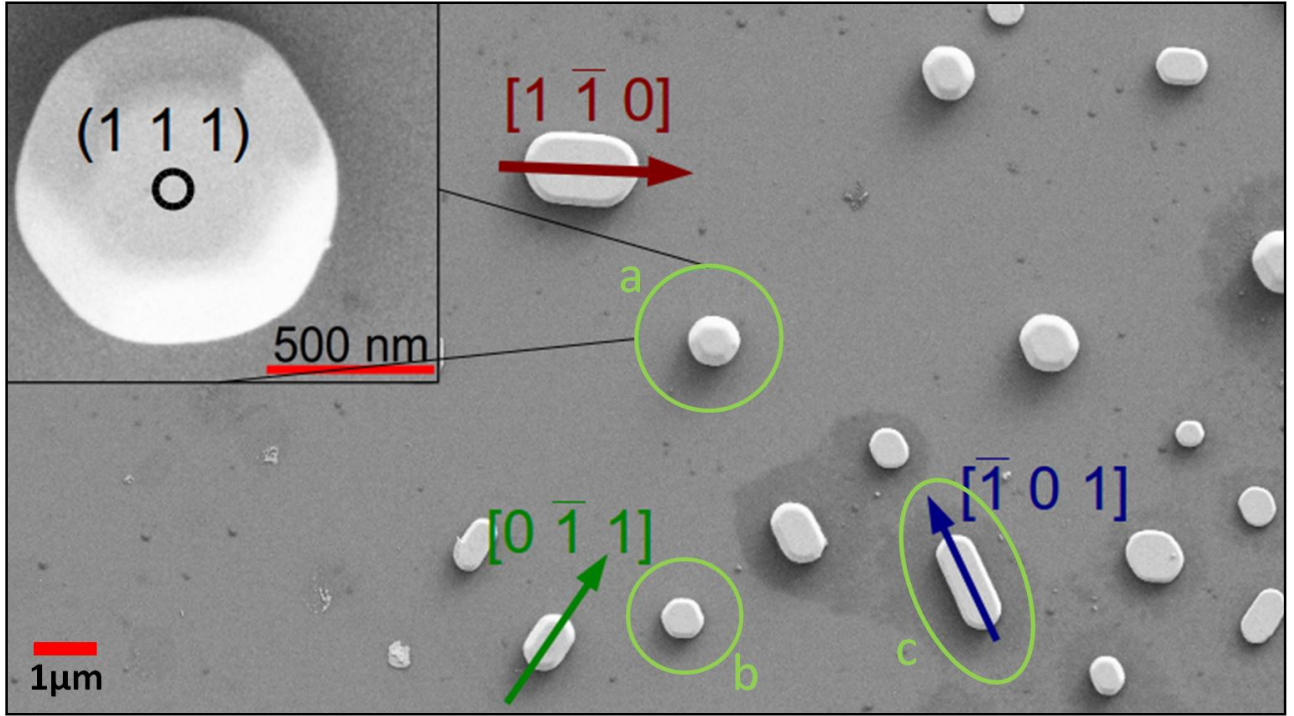
Figure 5.7: SEM image of an assembly of islands.
