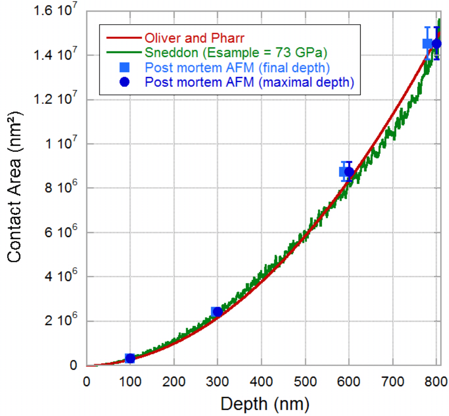
Figure 6.11: Contact area on bulk Au sample estimated from Oliver and Pharr model and Sneddon's equation and compared to post mortem AFM measurements. Post mortem AFM are given versus the maximal indentation depth (circle) and versus the final depth after unloading (square), in order to account for the elastic spring back.
