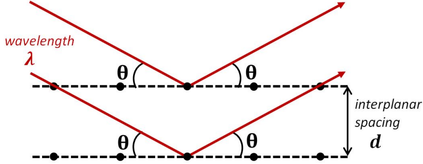
Figure C.1: Diffraction of a wavefront in Bragg condition.
