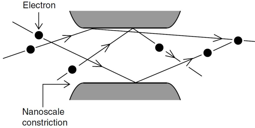
Figure 2.4: Ballistic motion of the electrons through a small constriction, from Brauvonic et al. [76]
