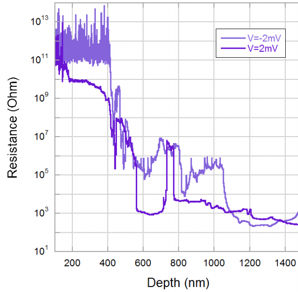
Figure 6.33: Example of resistance variations obtained while indenting bulk Al single crystal with a WC tip, measured with a Keihtley 6430 (SMU). Current density varies from 8 \cdot 10^5 A.cm -2 to 3 \cdot 10^3 A.cm -2 and indentation time is 80s.
