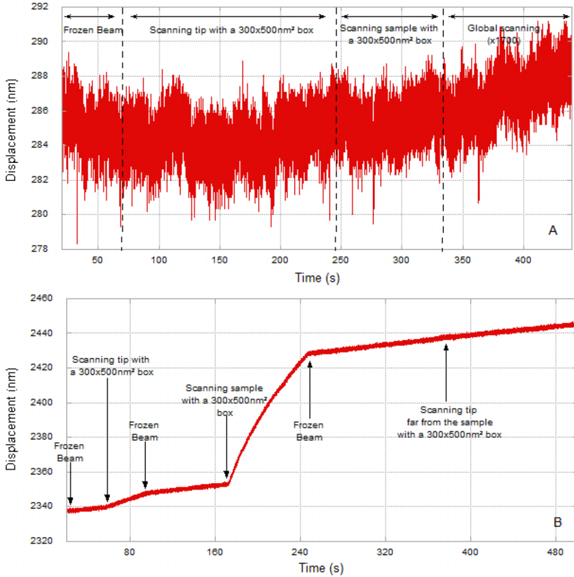
Figure 3.25: Effect of the beam on the nanoindenter column displacement at 2\text{ }\mu\text{m} from the contact (A) and at 150\text{ nm} of indentation depth (B) (metallized fused silica, 60\text{ }\mu\text{m} diameter diaphragm, \text{EHT} = 10\text{ kV} ).
