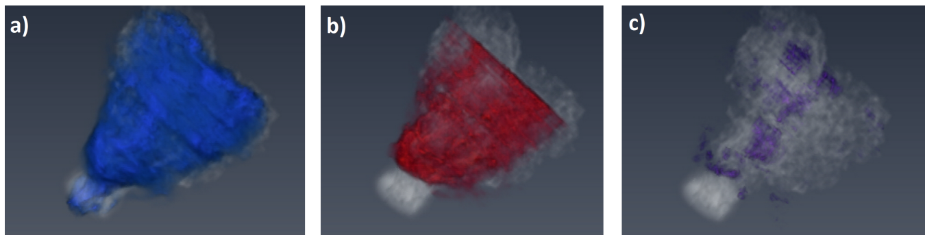
Figure 7.5: Superimposed X-ray and FTIR 3D reconstructions of (a) OH stretching, (b) CH aliphatic vibrations and (c) carbonates for the Paris 5 fragment.
