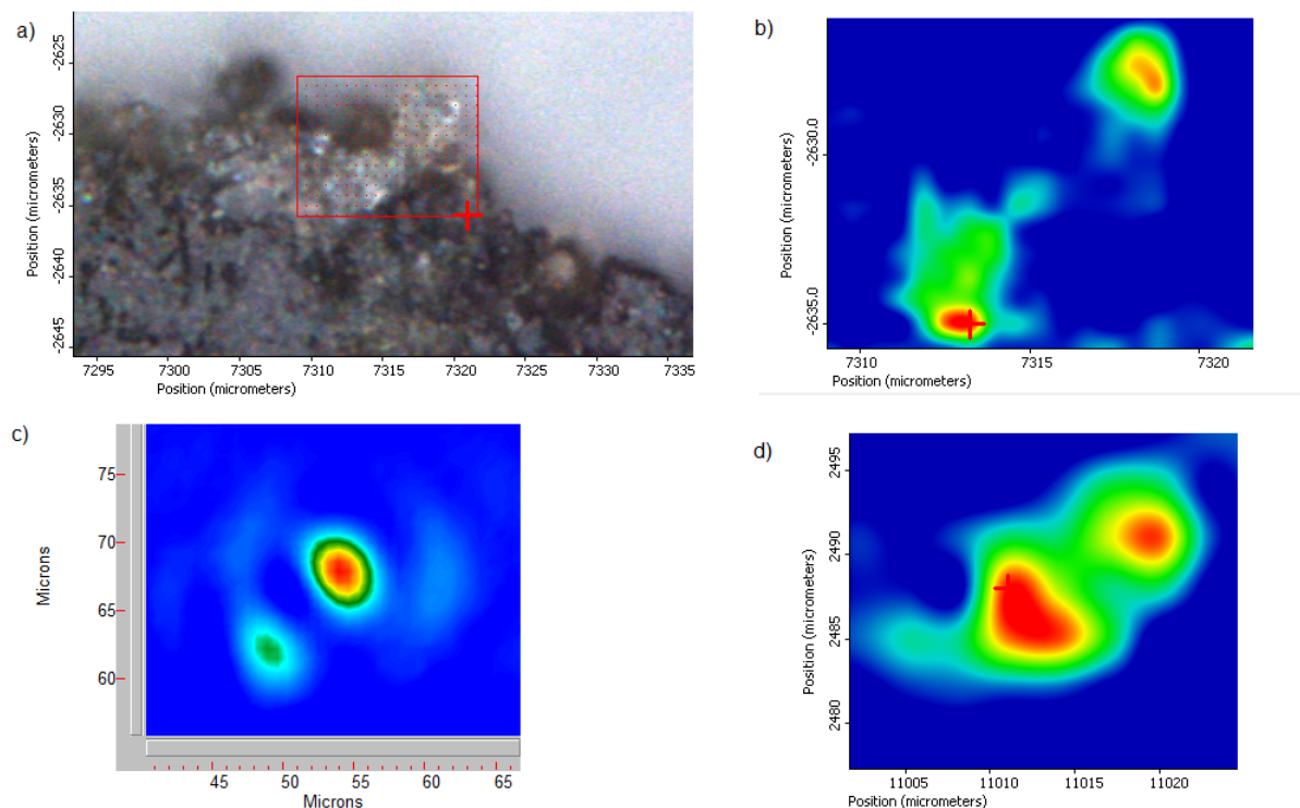
Figure 2.12: Comparison of two grains of carbonates observed with different setups: optical image (a) and maps of the same area obtained with (b) the Raman spectrometer, (c) the FPA, Globar source and (d) the single point MCT, SR source.
