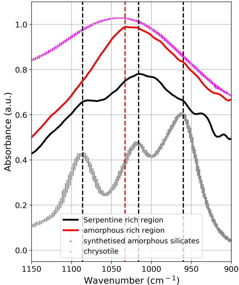
Figure 3.3: Spectrum from the amorphous region in red compared to amorphous spectrum from Demyk et al., 2017 in dashed pink and spectra from the serpentine region in black compared to the one from a pur serpentine in gray (Beck et al., 2014).
