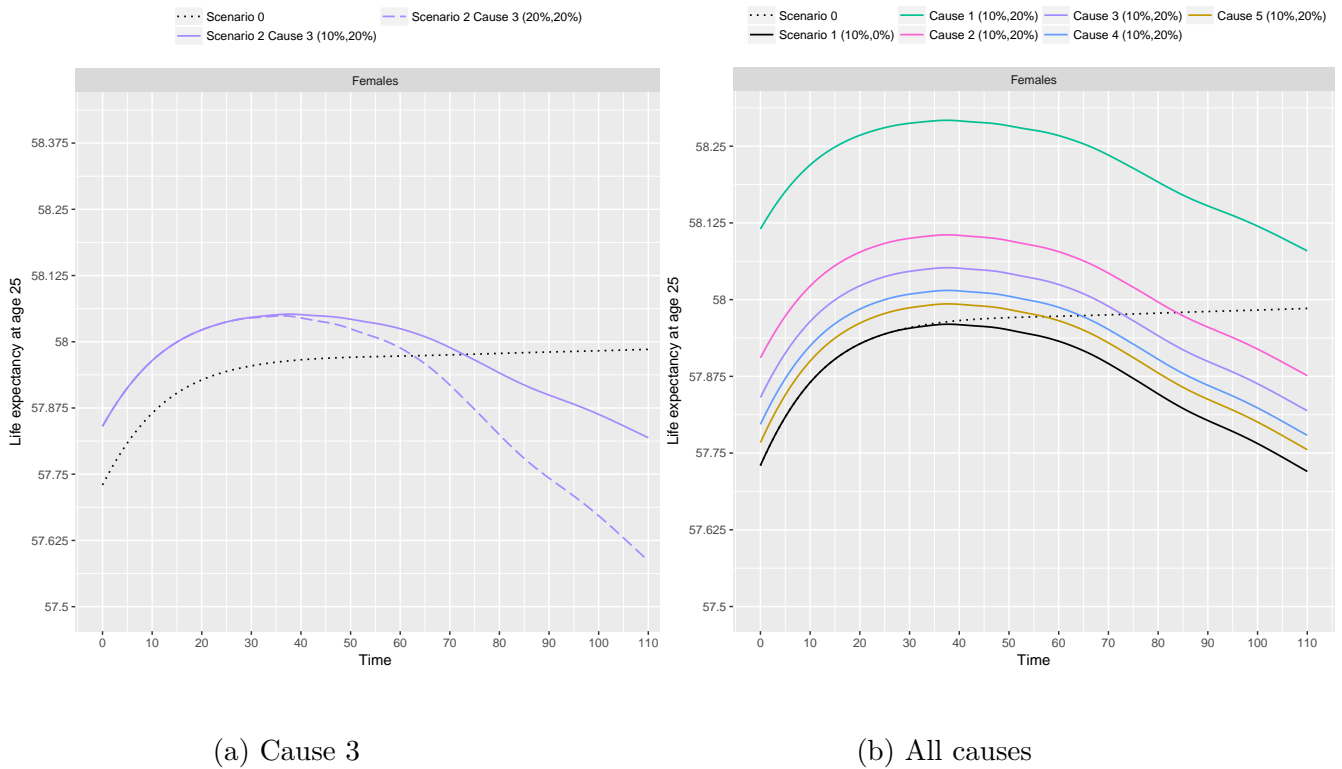
Fig. D.5 Aggregated period life expectancy over time with birth and mortality changes
