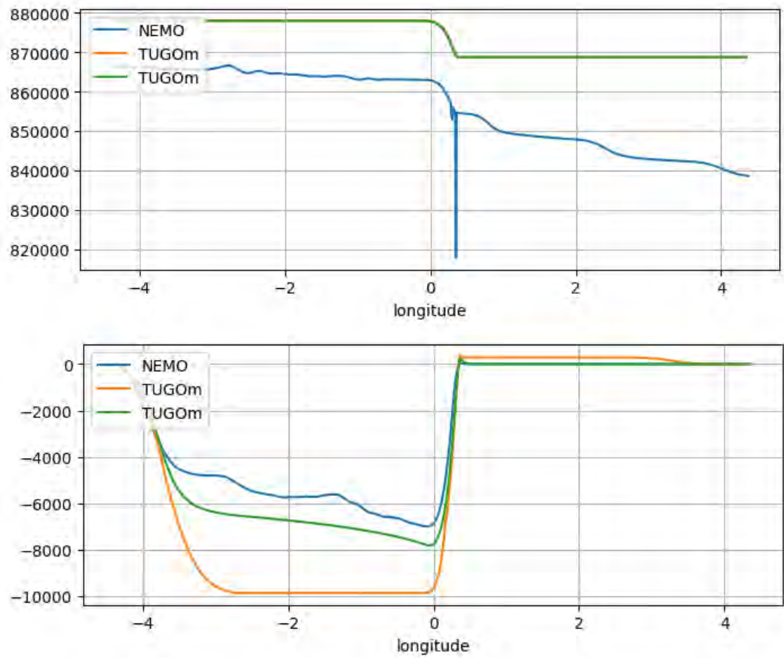
Figure 6.12: Comparison of barotropic flux (top) and baroclinic flux(bottom) for NEMO (blue lines), TUGO without diffusion(red lines) and TUGO with ( k_v = 5e^{-2} ) diffusion(green lines). Units are Wm^{-1}
