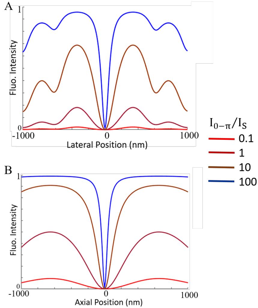
Figure 4.5: Simulated cross-sectional profiles of the fluorescence signal for different excitation intensities: A) along x, B) along z.
