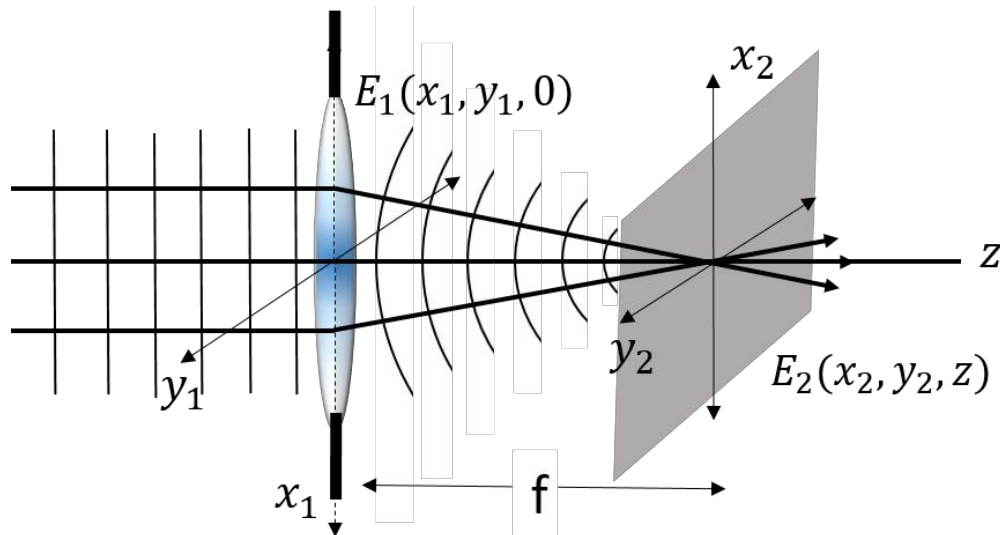
Figure 1.2: Focusing of a plane wave propagating through a converging lens. E_1(x_1, y_1, 0) is the aperture plane and E_2(x_2, y_2, z) is the focal plane.
