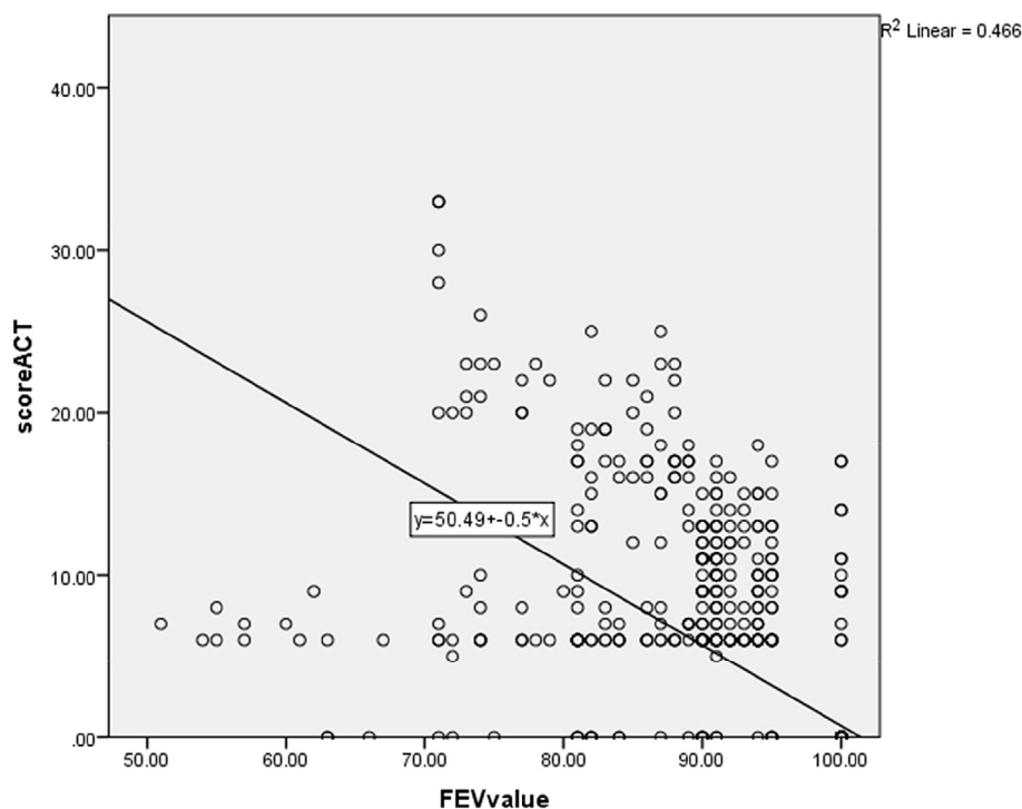
Fig. 1. Scatter plot of FEV value versus ACT score. R = -0.682 ( R^2 = 0.466 ); p < 0.001 ; ACT score = 50.49 - [(0.5 * FEV)] .
