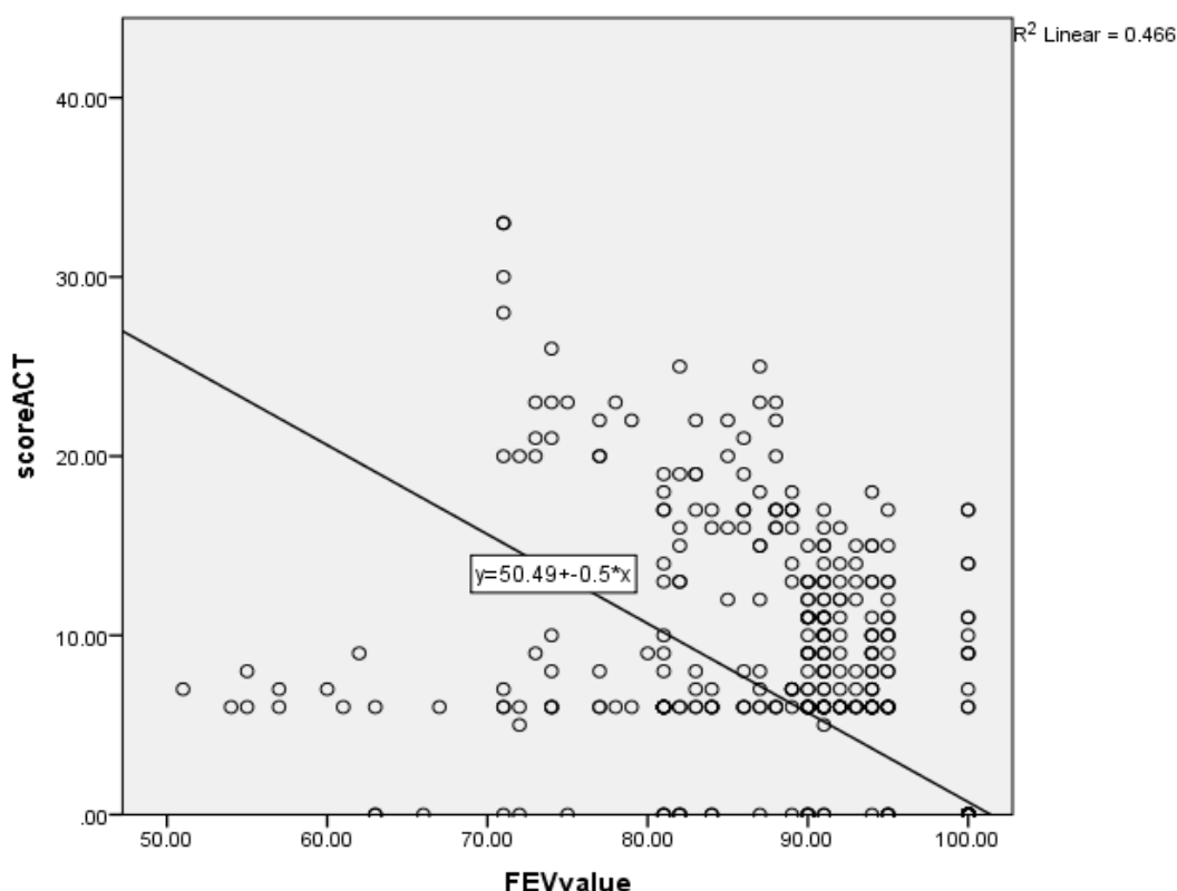
Figure 6: Scatter plot of FEV value versus ACT score. R = -0.682 ( R^2 = 0.466 ); p < 0.001 ; ACT score = 50.49 - [(0.5 * FEV)]
