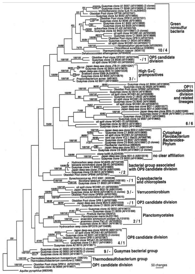
Figure 3: Bacterial diversity of hydrothermal active sediments of the Guaymas Basin
