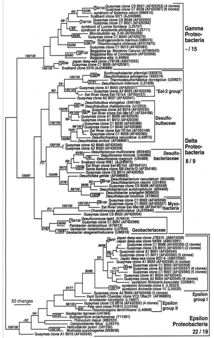
Figure 3: Bacterial diversity of hydrothermal active sediments of the Guaymas Basin
