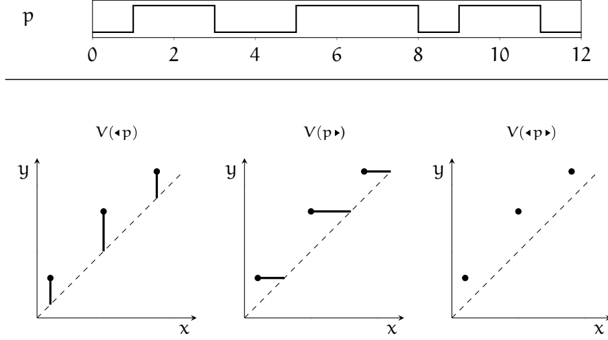
Figure 17: Valuations of anchored expressions.
