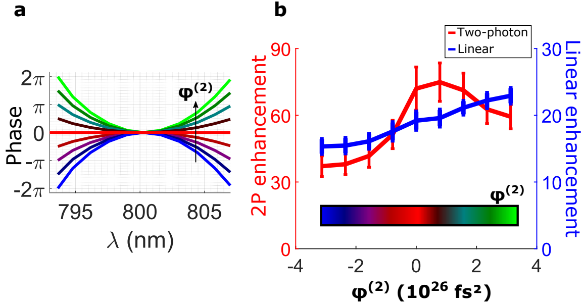
Figure 6.6 – Two photon signal upon an adjustable chirped pulse, via a quadratic spectral phase distribution with the full MSTM. Two-photon signal is emitted from fluorescent beads after propagation through a thick scattering sample. (a) Quadratic spectral phase relation applied on the output pulse via the MSTM. (b) Measured linear (blue) and two-photon (red) enhancements (SBR) as a function of the added group delay dispersion. Color-bar indicates the correspondence between the curvatures (color lines) in (a) and the x-axis in (b). Error bars are the corresponding standard deviation over 9 different focus positions.
