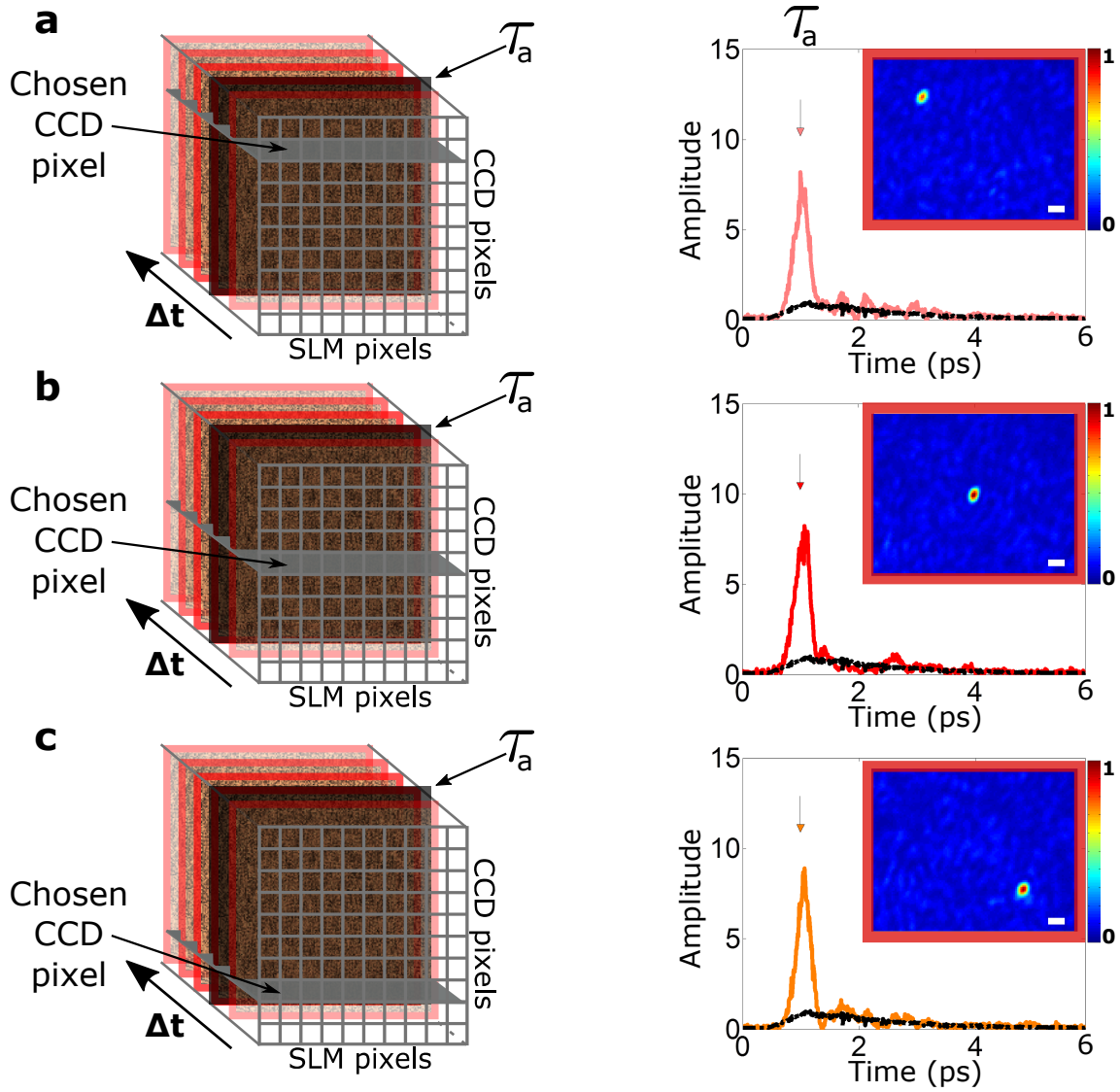
Figure 4.2 – Spatio-temporal focusing with a single time-gated Transmission Matrix. A single time-gated Transmission Matrix \mathbf{H}(\tau_a) (black vertical plan), corresponding to \tau_a = 1 ps, is extracted from the TRTM, that was measured with N_{\text{SLM}} = 256 SLM pixels. TRTM is illustrated on the left side. Spatial targeted position is represented by the gray horizontal cross-section on the TRTM. Temporal profile of the achieved spatio-temporal focusing is retrieved with ICC measurement. Focusing is achieved by phase-conjugating \mathbf{H}(\tau_a) . (a) A chosen targeted spatial position is selected on top left corner of the CCD image. The target position is visible on the CCD image in inset. Temporal profile at this spatial position shows a peak at time \tau_a , whose duration \sim 150 fs is close to the duration of the input pulse. The time-of-flight distribution (black line) is obtained by averaging temporal profiles over 100 different speckle grains at the output. The confinement time of photons inside the medium is evaluated from this averaged profile to be about \tau_m \simeq 2 ps. (b - c) Temporal profiles and the corresponding CCD camera images for spatio-temporal focusing processes performed at two different spatial positions, using the same transmission matrix \mathbf{H}(\tau_a) . Averaged temporal profiles are drawn in black. Intensity of CCD images are normalized by maximum of CCD image of (b). Scale bar: 5 \mu\text{m} .
