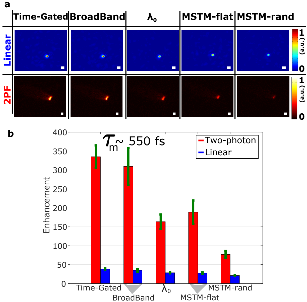
Figure 6.7 – Comparison of two-photon signals between the different transmission matrices, for a “thin” multiple scattering medium. (a) Linear (top line) and two-photon (bottom line) signals, upon focusing on a single fluorescent microbead, for different transmission matrices of a “thin” scattering medium ( \tau_m \sim 550 fs): Time-Gated, Broadband, monochromatic at \lambda_0 the central wavelength of the output pulse, and Multi-Spectral for either a flat spectral phase (MSTM-flat) or a random spectral phase (MSTM-rand). Color bar are normalized by maximum value of the Time-Gated images. Scale bars: 2 \mu\text{m} . (b) Linear (blue) and two-photon (red) enhancements averaged over 9 different focus positions. Error bars are the corresponding standard deviation.
