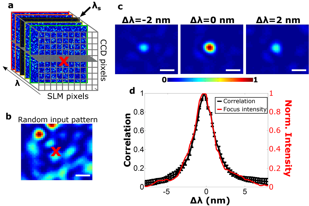
Figure 3.2 – Focusing a single wavelength of an ultrashort pulse via the MSTM through a scattering medium - spectral properties. (a) A single monochromatic TM( \lambda_s ) (black vertical cross-section) is extracted from the measured MSTM. The scattering medium is characterized by N_\lambda \sim 5 . Focusing light at wavelength \lambda_s is achieved via phase-conjugating a chosen line, which corresponds to the targeted spatial position (grey horizontal cross-section). Phase of the solution is displayed on the SLM. (b) Typical speckle pattern observed with CW light, with a random phase pattern on the SLM. Red cross corresponds to the targeted position for focusing. Its position is represented by the gray cross-section in the MSTM in (a). (c) Phase pattern to focus light at wavelength \lambda_s is displayed on the SLM. Monochromatic intensity images are recorded on the CCD camera as function of spectral detuning \Delta\lambda from \lambda_s . 3 monochromatic speckle patterns are represented, for respectively \Delta\lambda = -2 nm, \Delta\lambda = 0 nm, and \Delta\lambda = 2 nm with the same colorbar. At central wavelength (i.e. \Delta\lambda = 0 nm), in CW \text{SBR}_{\text{mono}} \sim 100 using N_{\text{SLM}} = 256 SLM pixels. (d) Normalized intensity of the focus, as well as spectral correlation, are plotted as function of spectral detuning \Delta\lambda . Scale bar: 4 \mu\text{m}
