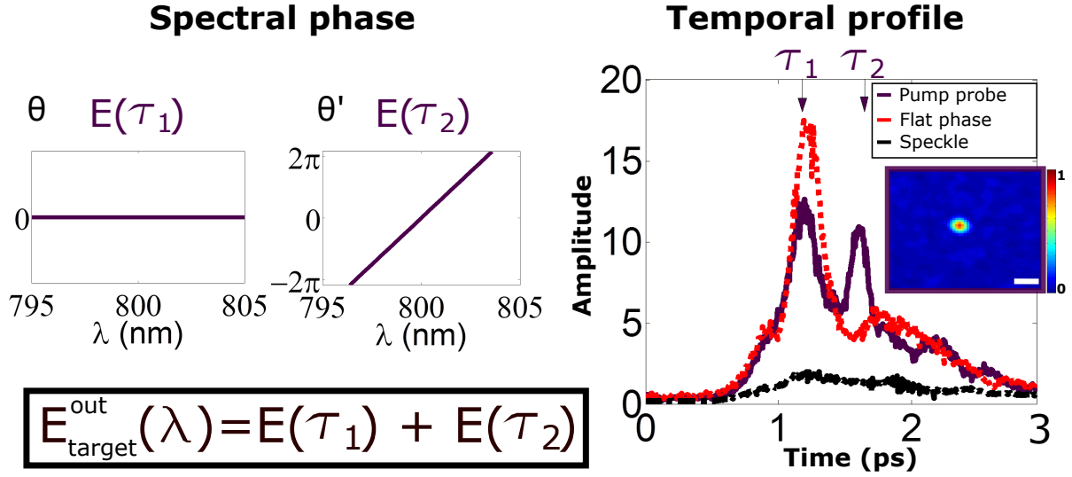
Figure 3.11 – Pump probe pulse profile with the full MSTM. A double pulse can be achieved with E_{target}^{out}(\lambda) that is the sum of two spatio-temporal focus, in the same spatial position but at different delays. (left) The global E_{target}^{out}(\lambda) corresponds to the sum of two spatio-temporal focusing whose spectral phase ( \theta_l ) and ( \theta'_l ) are shown. (right) Temporal profile of the achieved pulse, retrieved with ICC and averaged over 9 different focus positions. In the same spatial position, two pulses at delay time \tau_1 and \tau_2 are focused. Expected arrival times are shown with top arrows, whose delay times are calculated according to ( \theta_l ) and ( \theta'_l ). Inset: CCD image of a pump-probe focusing experiment. Light is focused in a single spatial position. Intensity is normalized by maximum of CCD image corresponding to a flat spectral phase pulse.
