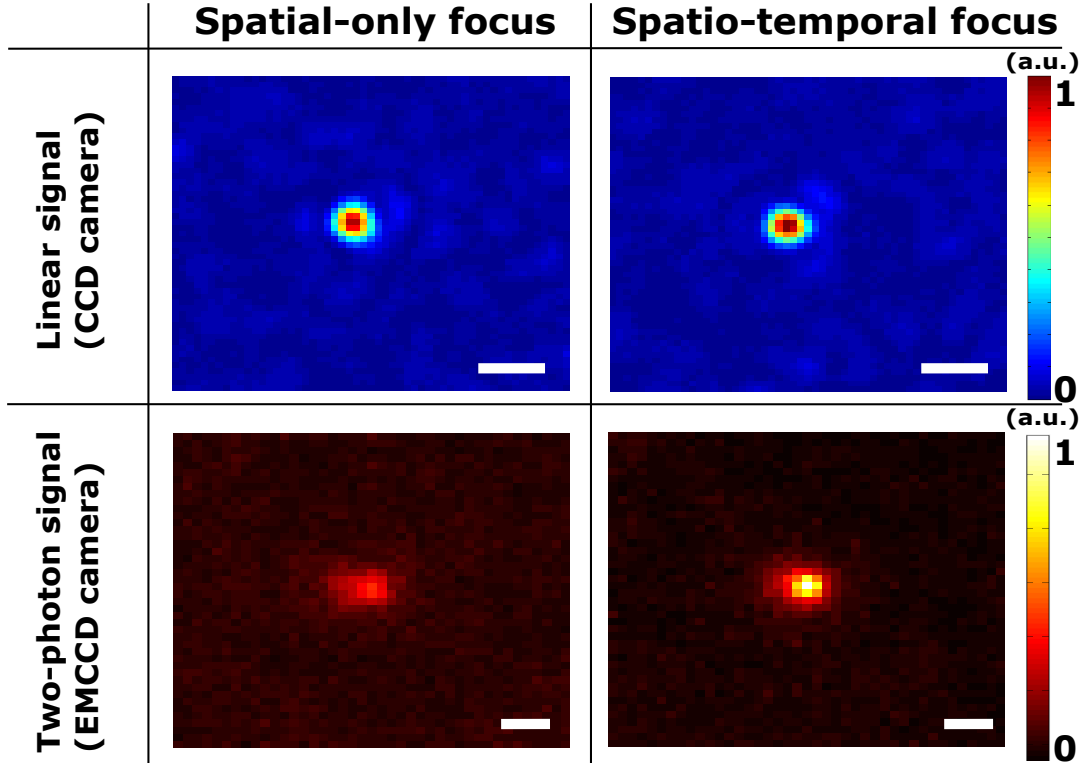
Figure 6.3 – Comparison of both linear and two-photon excitations for spatial-only focusing, and spatio-temporal focusing, with the MSTM. A two-photon screen is used to excite 2PF. The scattering medium is characterized by its spectral correlation bandwidth \delta\lambda_m \sim 2 nm. Spatial-only focusing is achieved by focusing only the central wavelength of the output pulse. Top line: Linear signal measured with the CCD camera. Bottom line: Corresponding two-photon signal, measured with the EMCCD camera. Color-bars are normalized to the maximum intensity of spatio-temporal focusing. Scale bar: 5 \mu\text{m} .
