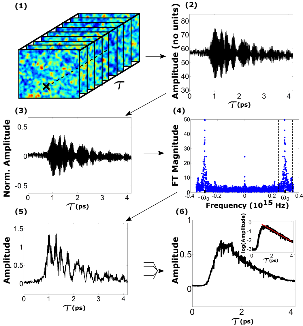
Figure 2.8 – Interferometric Cross-Correlation characterizes temporal fluctuation of spatio-temporal speckle. Interferometric Cross-Correlation (ICC) is performed using experimental setup presented in Figure 2.1. An ultrashort reference pulse, whose arrival time is controllable with a delay line, is overlapped spatially and temporally with spatio-temporal speckle. The two beams are coherent. (1) Interference images are recorded as function of delay \tau , by scanning the delay line. (2) Interferogram at a given spatial position, defined by the black cross in (1). Intensity of the cross-term between reference pulse and stretched pulse is linearly related to the amplitude of spatio-temporal speckle field at this specific position. (3) Normalized interferogram by subtracting baseline, and by dividing over both amplitude of reference and signal beams. (4) Fourier transform of the normalized interferogram. Peak at \omega_0 , the central frequency of the ultrashort pulse, is filtered with a band-pass filter, and shifted down to DC. (5) Inverse Fourier transform of the filtered signal. Only envelope of interferogram is remaining: we directly access temporal speckle at a given spatial position. Approximately N_\lambda temporal speckle grains are present. (6) Averaging over N=1000 spatial speckle positions leads to time-of-flight distribution. Its tail has an exponential decay, of characteristic time \tau_m \propto 1/\delta\lambda_m is the averaged confinement time of photons in the scattering medium. Inset: time-of-flight distribution in semilog diagram. Linear fit of the tail (red line) gives access to \tau_m , via the inverse of its slope.
