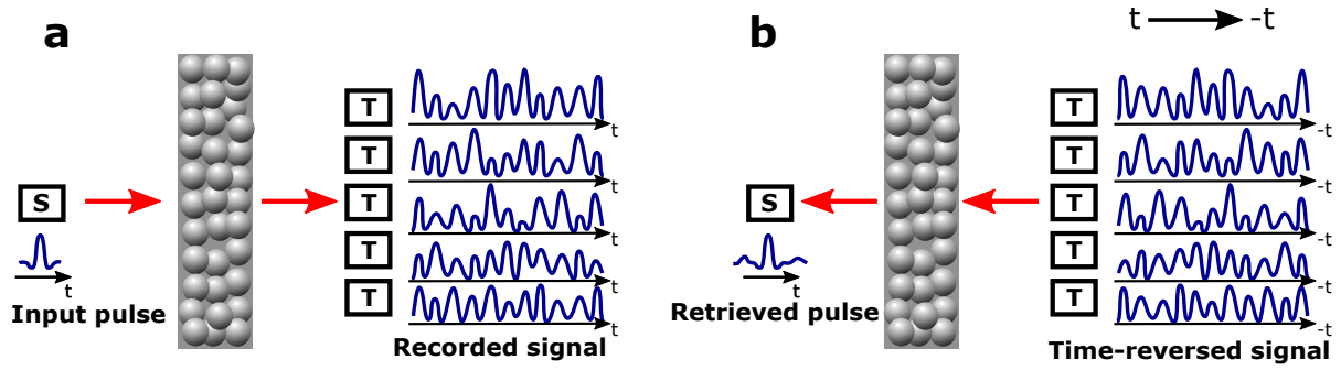
Figure 1.19 – Time-reversal of acoustic waves. Temporal reciprocity of the wave equation is at the origin of time-reversal experiments. (a) In a first step, an ultrasound pulse is propagating through a multiple scattering sample, and detected with few transducers on the other side of the medium. Temporal signals are digitally recorded. (b) In a second step, temporal signal measured previously are reversed. Transducers are emitting these time-reversed signals back to the sample. At the source location, a short pulse is detected at a given delay time, with similar duration as the input pulse. S: source; T: transducer
