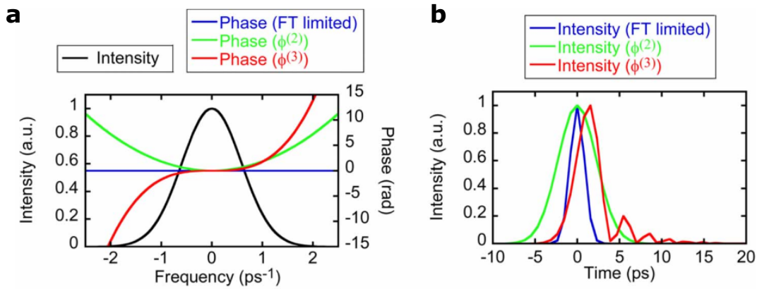
Figure 1.14 – Impact of dispersion terms on the ultrashort pulse duration and shape. (a) Spectral intensity of the considered pulse, associated with three different spectral phases: flat (in blue), quadratic ( \varphi^{(2)} term, in green) and cubic ( \varphi^{(3)} term, in red). (b) Corresponding temporal profiles of pulses. The flat spectral phase leads to a Fourier-limited pulse. The quadratic term increases the temporal duration of the pulse. The cubic term creates post-pulses. Image adapted from [Walmsley and Dorrer, 2009]
