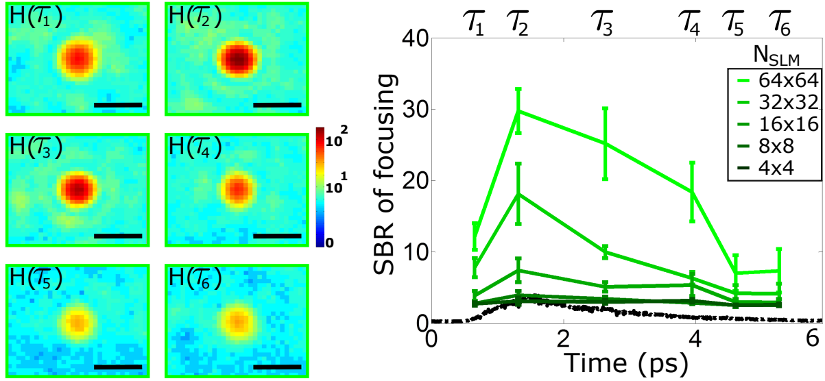
Figure 4.5 – Signal-to-background ratio upon focusing with a single time-gated transmission matrix. Signal-to-background ratio (SBR) measured on the CCD camera for different targeted arrival times, and different number of modes controlled at the input N_{\text{SLM}} . The SBR is the ratio of the intensity at the targeted pixel of the CCD camera and the mean intensity value of the full speckle image. (left) CCD images of focusing using a 6 different time-gated transmission matrices (TGTMs) at 6 arrival times \mathbf{H}(\tau_k) . The corresponding TGTMs were measured with N_{\text{SLM}} = 64 \times 64 SLM segments. Intensity is represented in log scale. Scale bar: 5 \mu\text{m} . (right) SBR of focusing measured on the CCD camera at 6 different arrival times \tau_k , and different N_{\text{SLM}} . Error bars are standard deviation for SBR over 9 different focus positions.
