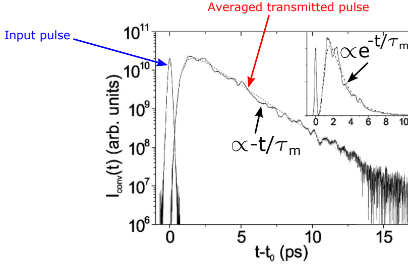
Figure 1.16 – Time-of-flight distribution of photons after propagation through a strong disordered medium. Time-of-flight distribution of photon passing through a thick GaP sample, plotted in log scale. Tail of time-of-flight distribution has an exponential decay (see inset), from which the average confinement time of photons in the scattering medium \tau_m can be extracted. Image adapted from [Johnson et al., 2003]
