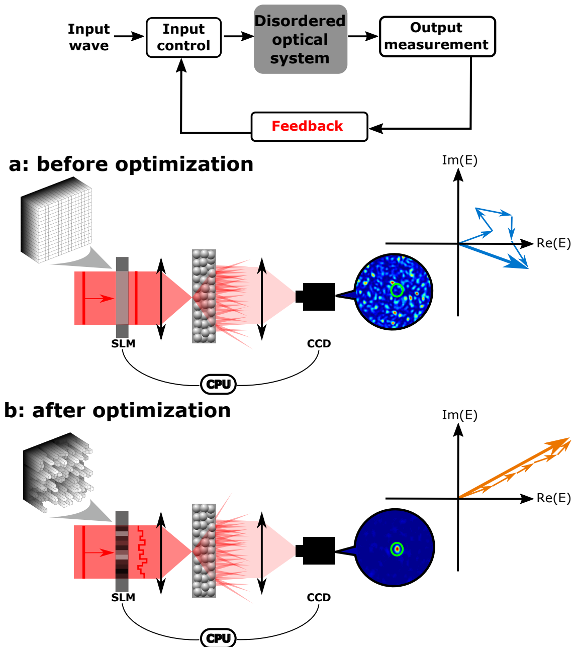
Figure 1.7 – Iterative optimization algorithm to focus light through a scattering medium. (Top) Typical sketch of wavefront shaping setup via an iterative optimization algorithm. (a) Coherent light is propagating through a disordered sample. Transmitted light is imaged on a CCD camera. The input wavefront of light can be controlled before propagation in the medium with a SLM. Each pixel of the SLM contributes as a phasor in the output field, with a uniform phase distribution because of scattering. Before starting the optimization algorithm, the SLM pattern is flat: the output field results in a speckle. Field distribution in the target position (center of the green circle) is schematically represented in the complex plane, as in Figure 1.5. (b) Iterative optimization algorithm is strongly enhancing the intensity at the target position, by launching a closed loop between SLM pattern and intensity in the target as feedback signal, both connected via a CPU. In the complex plane at the position of the target, the phasors are now aligned in phase, driving a constructive interference which leads to a brighter intensity spot. The final input wavefront is no longer a plane wave, but a distorted wavefront controlled by the SLM. More details about iterative optimization algorithms available in [Vellekoop, 2015]
