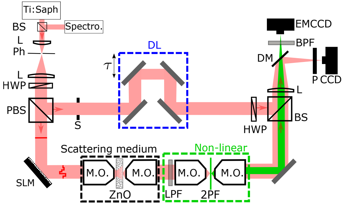
Figure 2.1 – Experimental setup for spatio-temporal control of an ultrashort pulse through a scattering medium. The laser source, emitted from a Ti:Saph oscillator, has two operating modes: either tunable cw, or mode-locking that generates an ultrashort pulse of duration 100 fs at FWHM. Laser beam is expanded and it illuminates a phase-only Spatial Light Modulator (SLM), which is conjugated with the back focal plane of a microscope objective. The scattering medium is a thick (around 100 \mu\text{m} ) sample of ZnO nanoparticles, placed between two microscope objectives. The output facet is imaged on a two-photon fluorescence (2PF) sample. A long-pass filter (LPF) allows one to eliminate the autofluorescence of ZnO. A dichroic mirror (DM) separates the two-photon fluorescence signal (imaged with an EMCCD camera) from the linear signal (imaged with a CCD camera). A delay line (DL) is adjusting delay between reference beam and scattered light. A shutter (S) may block the delay line, for instance when performing spectral correlation measurements. Lens (L), pinhole (Ph), half plate wave (HPW), polarized beam-splitter (PBS), delay line (DL), beam splitter (BS), polarizer (P), band pass filter (BPF), spectrometer (Spectro.).
