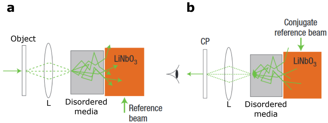
Figure 1.9 – Typical sketch of an optical phase conjugation setup with a photorefractive crystal. (a) In the first step, scattered light is recorded. (b) Secondly, the optical phase conjugated field is sent back. L: Lens, CP: compensation plate; Image adapted from [Yaqoob et al., 2008].
