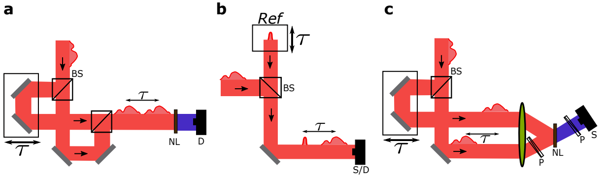
Figure 1.15 – Typical methods to characterize an ultrashort pulse (a) Intensity autocorrelation. (b) Spectral or temporal interferometry. (c) Polarization-Gated Frequency-Resolved Optical Gating. (BS): beam splitter, (NL): non-linear crystal, (D): photo-detector or camera, (S): spectrometer, (P): polarizer.
