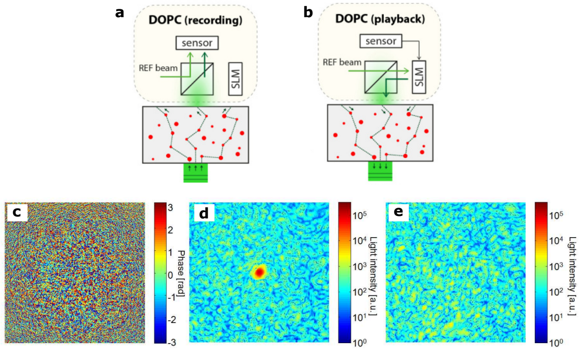
Figure 1.10 – Typical sketch of a digital optical phase conjugation setup. A sensor (usually a CCD camera) and a SLM are located in conjugated planes with respect to a beam splitter. Their respective pixels are matched pixels by pixels. (a) In the first step, the scattered field is measured on the sensor via an interference with a reference beam. (b) Secondly, the phase map measured on the sensor is displayed on the SLM. The same reference beam is now reflected on the SLM: phase-conjugation operation is digital. The reference beam is propagating in the scattering medium following the same channels used in the first step, but backwards. (c) Example of a phase map measured on the sensor. Scattering effects in the disordered material (random polystyrene microspheres here) make the phase map looking very complex, nonetheless measurable. (d) Reconstructed focus obtained by phase conjugating the field measured in (c), in log scale. (e) Reconstructed image with a flat pattern displayed on the SLM. Image (a-b) adapted from [Jang et al., 2015], Image (c-e) adapted from [Cui and Yang, 2010].
