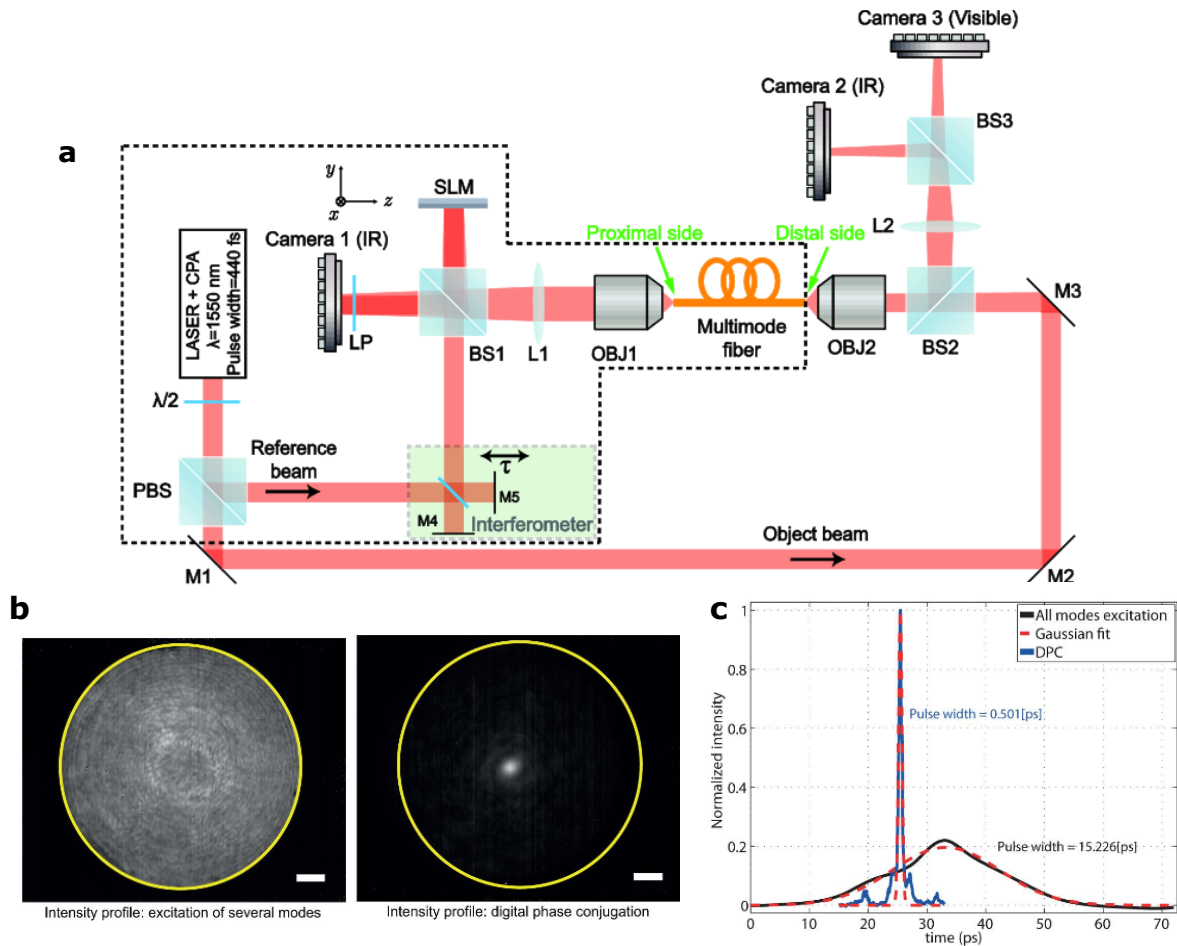
Figure 1.21 – Digital optical phase conjugation of a short pulse. (a) Typical experimental set-up. A 440 fs pulse centered at \lambda_0 = 1550 nm is injected into a step-index multimode fiber via a microscope objective OBJ2. The output pulse is interfering with a tilted reference beam. A delay-line in the reference beam enables to filter photons arriving at a given time. An off-axis hologram is recorded at a given time on Camera 1. Its phase conjugate is displayed on the SLM. The reference beam is back propagating into the fiber. The output facet is imaged on camera 2 and an autocorrelator (camera 3). (b) Image of the output facet of the fiber without (left) and with (right) DOPC. DOPC is building up a focus among the background speckle. (c) Temporal profile without DOPC (in black) and at the focus obtained with DOPC (in blue). The output pulse recovers almost its initial duration with DOPC. Images adapted from [Morales-Delgado et al., 2015]
