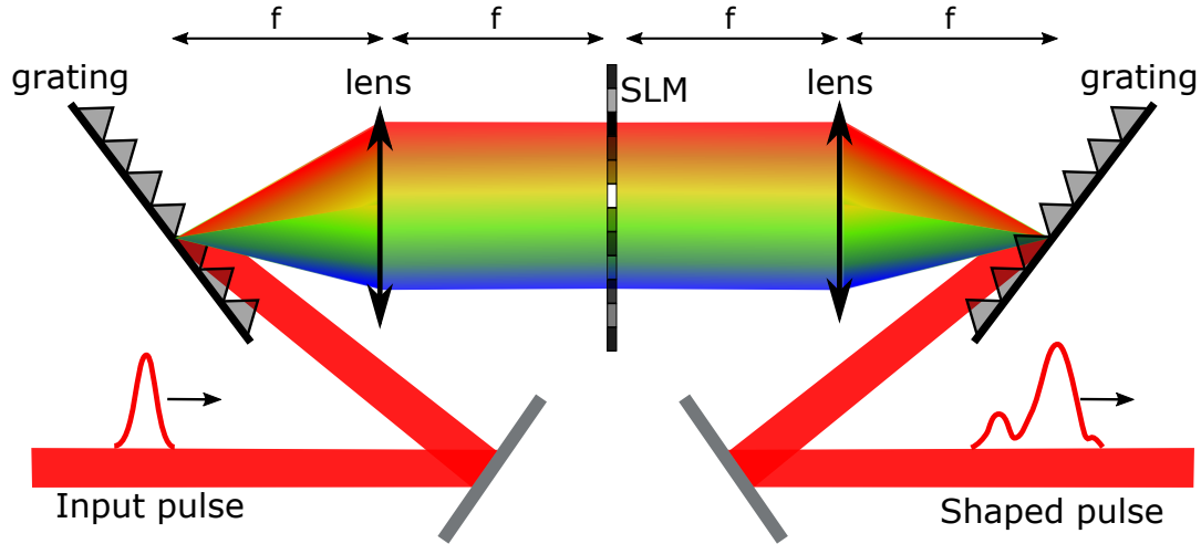
Figure 1.20 – Pulse shaping of an ultrashort pulse. Spectral amplitude and spectral phase of an ultrashort pulse are shaped directly in the spectral domain with a 4f imaging system. The input pulse is focused on a grating, that is imaged with a lens on a spatial light modulator: every spectral components can be addressed independently on the SLM. The SLM is conjugated with another grating via another lens. The obtained pulse can be temporally shaped at will via spectral shaping.
