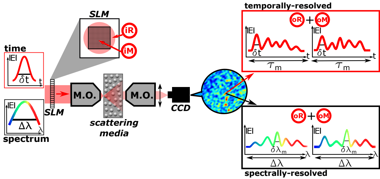
Figure 5.1 – Principle of the measurement of the Broadband transmission matrix. An input pulse of duration \delta t \sim 100 fs (spectral width \Delta \lambda \sim 10 nm) illuminates a spatial light modulator (SLM) before propagation through a thick scattering medium via a microscope objective (MO). The active part of the SLM will modulate a subpart of the input beam iM with respect to a static reference part iR. The transmitted light results in an intensity speckle with low contrast C_0 \simeq 1/\sqrt{N_\lambda} , with N_\lambda the number of spectral degrees of freedom, on a CCD camera. Every single grain is the resulting broadband interference of the transmitted speckle from the input reference part oR and from the input modulated part oM. The BBTM is the linear relationship connecting iM to oM. In the temporal domain, the speckle grain is characterized by its temporal feature \delta t , and by the averaged traversal time of photons through the medium \tau_m . In the spectral domain, the speckle has a characteristic width \delta \lambda_m , which is the spectral speckle correlation bandwidth of the medium.
