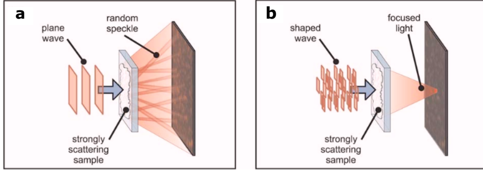
Figure 1 – First wavefront shaping experiment with CW light. (a) Upon a plane wave illumination, transmitted light through a thick layer of white paint takes the form of a random speckle. (b) Wavefront shaping the incident beam enables light focusing after propagation through the scattering medium. Image adapted from [Vellekoop and Mosk, 2007]
