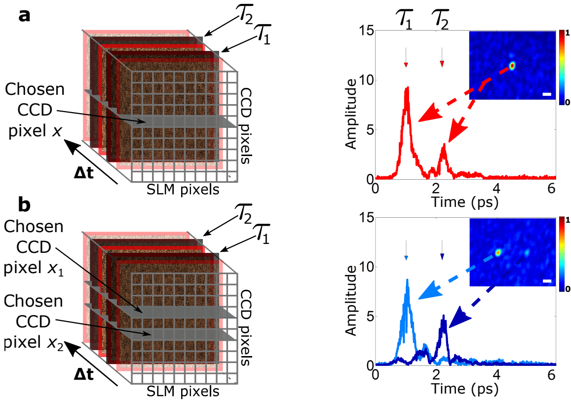
Figure 4.6 – Complex spatio-temporal shaping by exploiting the full TRTM. Two time-gated transmission matrices at delay times \tau_1 and \tau_2 are extracted from TRTM. (a) Temporal profile recorded using a spatio-temporal focusing process at one spatial position x (gray horizontal plane on the TRTM) and at two different arrival times \tau_1 = 1 ps and \tau_2 = 2.2 ps. CCD image in inset shows the position of the spatial target. (b) Temporal profiles recorded using a spatio-temporal focusing process at the same two different arrival times, \tau_1 = 1 ps and \tau_2 = 2.2 ps, and at two different spatial positions, x_1 and x_2 (gray horizontal planes the TRTM), visible on the CCD image in inset. CCD is normalized by maximum intensity of (a) . Scale bar is 5 \mu\text{m} .
