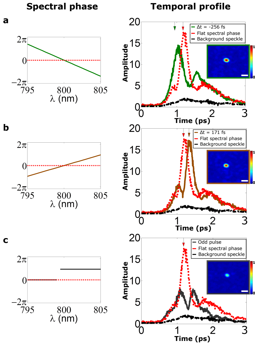
Figure 3.10 – Controllable pulse shaping with the full MSTM. A set of different spectral phase distributions ( \theta_l ) is applied on E_{\text{target}}^{\text{out}}(\lambda) with similar spectral amplitude ( r_l ), that is fitting a similar Gaussian shape as the input pulse spectrum. Spectral phase distribution is shown on left, and the corresponding measured temporal profile of focus, retrieved with ICC technique and averaged over 9 different focus positions, is shown on right. Red top arrow indicated delay line position where MSTM has been measured. (a-b) A spectral phase ramp is applied. Slope of the ramp is tuning the pulse arrival delay time related to flat spectral phase pulse, while its sign indicates if the output pulse is being advanced or retarded. Colored top arrows indicate expected arrival time according to applied spectral phase slope. (c) An odd pulse is obtained by imposing a \pi -phase step in the spectrum. A dip appears in the temporal profile instead of a peak. Insets: CCD image of focusing for each spectral phase relation, normalized by CCD intensity of flat spectral phase pulse. Scale bar: 5 \mu\text{m} .
