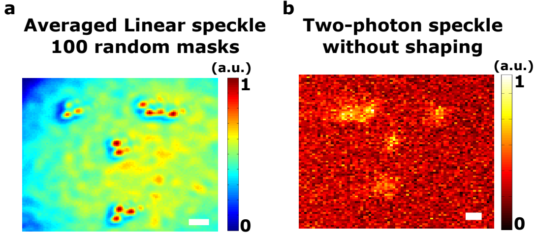
Figure 6.2 – Two-photon signal from fluorescent microbeads. The scattering medium is characterized by \tau_m \sim 1 ps. Fluorescent microbeads (diameter 1 \mu\text{m} ) are spread over a microscope slide, and inserted in the experimental setup. Transmitted light is collected with an oil immersion microscope objective ( \times 60 , \text{NA}=1.4 ). (a) Mean linear speckle image, obtained by averaging over 100 different speckles (from different random patterns on the SLM) measured with the CCD camera. We thus mimic homogeneous illumination with the setup: N_b = 12 beads are identified in the imaging zone. (b) Two-photon signal measured on the EMCCD camera with a random pattern on the SLM. Gain=1000 and exposure time T_e = 1000 s. Scale bars: 2 \mu\text{m} .
