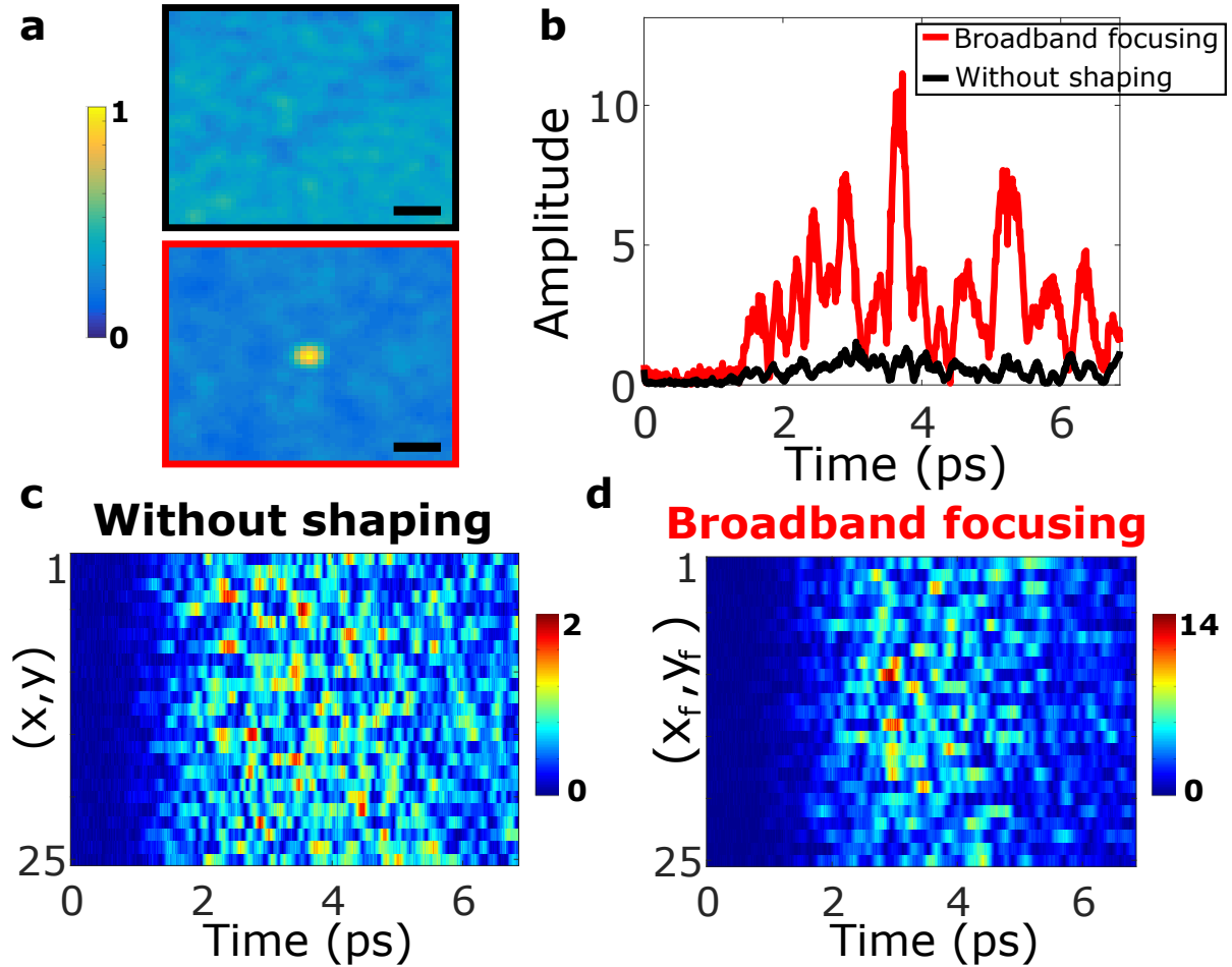
Figure 5.3 – Temporal profile when focusing with the Broadband transmission matrix. The scattering medium is characterized by its confinement time \tau_m \sim 6 ps. (a) CCD images measured with the shutter of the external arm S closed. Top: Without wavefront shaping, or equivalently with a random input phase pattern on the SLM, a low-contrasted speckle is measured. Bottom: The output pulse is focused on the central spatial speckle grain. Scale bar: 5 \mu\text{m} . (b) Time-of-flight distributions retrieved with ICC, in a single speckle grain in the case of (red) focusing with the BBTM and (black) without shaping. (c-d) Temporal profiles over 25 different spatial positions (x, y) either without shaping (in (c) ) or in different focus in positions (x_f, y_f) (in (d) ) with the same scattering sample. Colormap stands for the amplitude of the temporal profile at chosen spatial position and arrival time.
