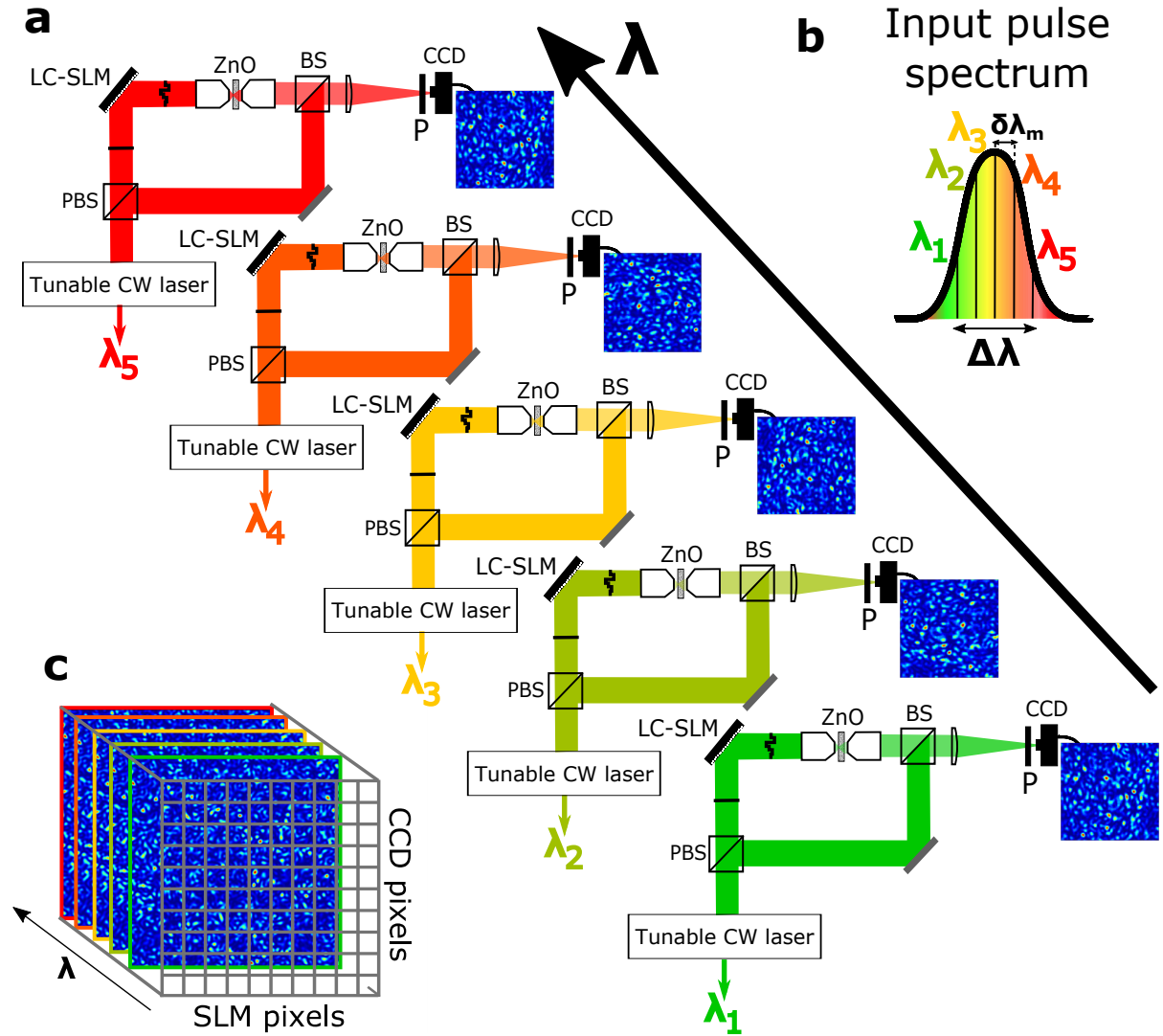
Figure 3.1 – Multi-Spectral Transmission Matrix measurement. Scheme of the Multi-Spectral Transmission Matrix of a scattering medium. N_\lambda stands for the number of spectral degrees of freedom. (a) Measurement of the MSTM is discretized: N_\lambda monochromatic TMs are measured, at wavelengths separated to each other by \delta\lambda_m that corresponds to the spectral correlation bandwidth of the medium. The experimental setup is simplified from the real one that is presented in Figure 2.1. For clarity, we chose N_\lambda = 5 in this representation. (LC-SLM) : Liquid-Crystal Spatial Light Modulator; (PBS): Polarized Beam Splitter; (BS): Beam Splitter; (P): Polarizer; (CCD): Charged Coupled Device; (ZnO): Zinc Oxide scattering medium. (b) The N_\lambda wavelengths are represented with black lines over the spectrum of the input pulse. \Delta\lambda stands for the spectral bandwidth of the ultrashort pulse. (c) Typical schematic representation of the Multi-Spectral Transmission Matrix, of dimension N_{\text{out}} \times N_\lambda \times N_{\text{SLM}} , where N_{\text{out}} stands for number of CCD pixels, and N_{\text{SLM}} the number of SLM pixels exploited in the measurement of TMs. Each monochromatic TM has been measured at a different wavelength, that is represented with a chosen color. In practice N_{\text{out}} \sim 10^4 pixels, N_{\text{SLM}} \sim 1024 pixels and N_\lambda \sim 20 spectral degrees of freedom.
