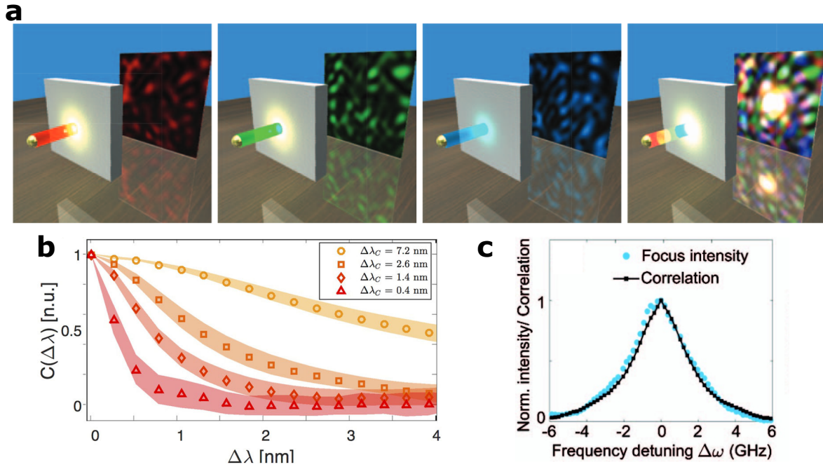
Figure 1.17 – Wavelength-dependent monochromatic speckle. Monochromatic light passing through a scattering medium leads to a speckle that depends on the incident wavelength. (a) Three individual different spectral components (on the left) give rise to three uncorrelated speckle patterns. Combination of the three incident colors (last on the right side) generates a complex spatio-spectral speckle, that is the incoherent sum of the previous monochromatic speckle patterns. (b) Correlation between monochromatic speckles as a function of spectral detuning, for four samples of different thicknesses with the same l^* . Spectral correlation bandwidth of the scattering medium \delta\lambda_m can be extracted. (c) A monochromatic focus has the same spectral bandwidth as the medium: light is controlled only for a single spectral channel. Images adapted from (a) : [Mosk et al., 2012], (b) : [Andreoli et al., 2015], (c) : [van Beijnum et al., 2011]
