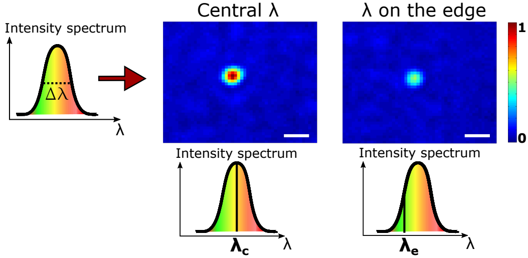
Figure 3.3 – Monochromatic focusing of different individual wavelength of the ultrashort pulse spectrum. Phase pattern is displayed on the SLM to focus either central wavelength of the pulse \lambda_c , or wavelength on the edge \lambda_e , where spectral amplitude of the pulse is half of the maximum. Laser is now emitting an ultrashort pulse of light. SBR of focusing at \lambda_c \sim 13 , while SBR at \lambda_e \sim 7.5 . MSTM has been measured with N_{\text{SLM}} = 1024 SLM pixels, for a scattering medium that is characterized by N_\lambda \sim 20 . Scale bar: 4 \mu\text{m}
