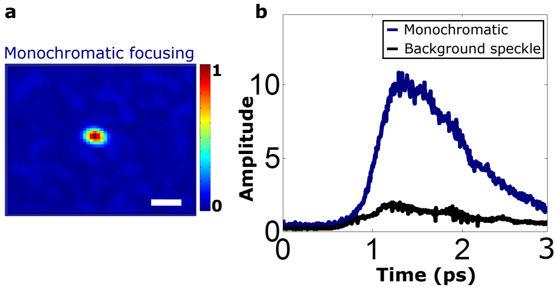
Figure 3.4 – Focusing a single wavelength of an ultrashort pulse via the MSTM - temporal properties. (a) CCD image of monochromatic focusing (central wavelength of the pulse) in a given output spatial position, while the laser is mode-locked. Intensity is normalized. (b) Temporal profile of monochromatic focusing is recorded with Interferometric Cross-Correlation (ICC) technique. In blue: averaged temporal profiles of monochromatic focusing over 9 spatial positions. In black: averaged temporal profiles of spatial speckle grains with a random input phase mask on the SLM, over 200 positions: the scattering medium is characterized by its confinement time of photon \tau_m \sim 1.8 ps. Amplitude of monochromatic focusing is higher, but temporal compression is missing, as only a single spectral degree of freedom over N_\lambda is controlled.
