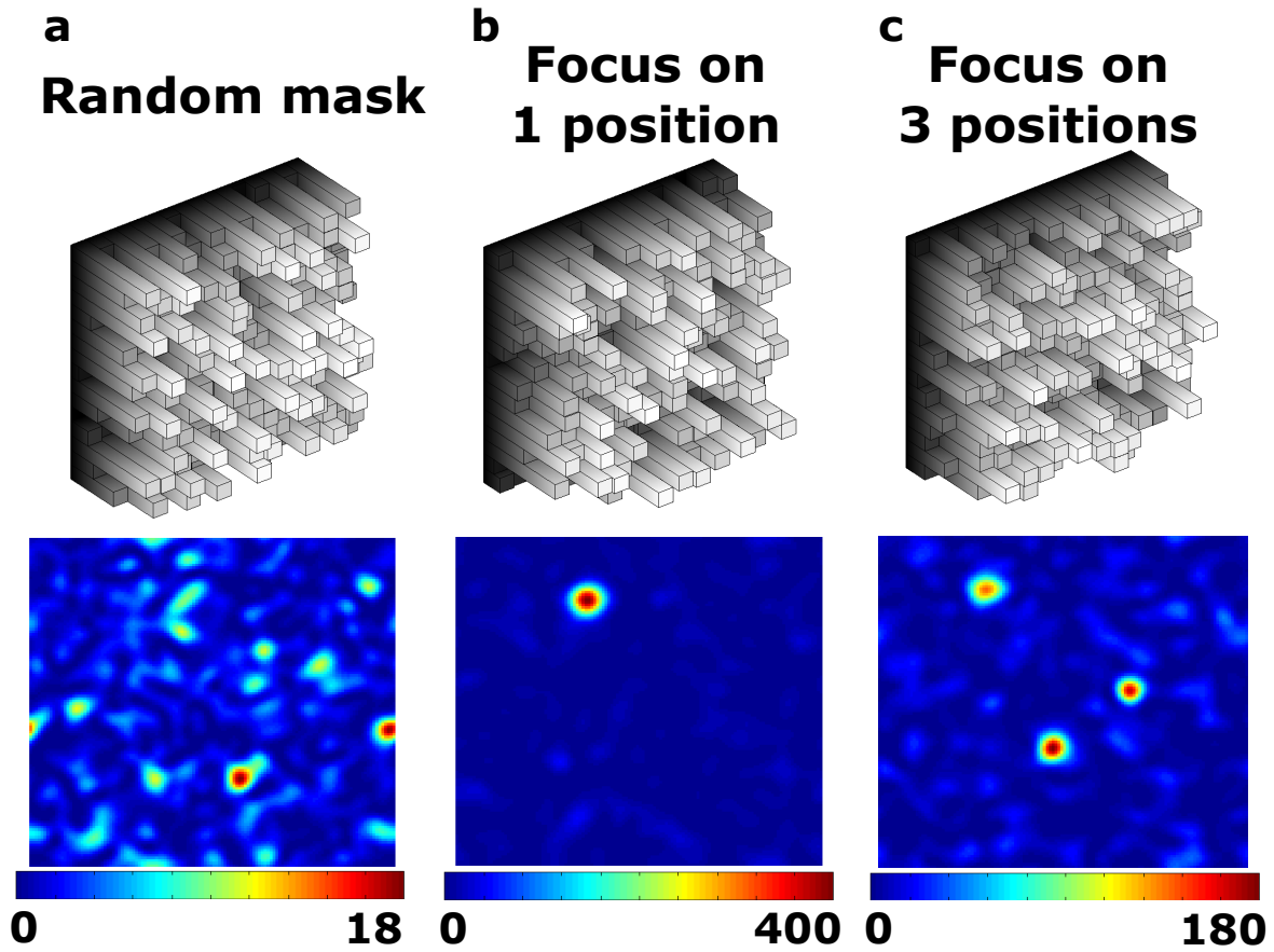
Figure 1.12 – Focusing monochromatic light through a scattering medium via the monochromatic transmission matrix. The monochromatic TM has been measured following the previous protocol developed in Figure 1.11. Phase patterns displayed on the SLM ( N_{\text{SLM}} = 256 ) are represented on top. The corresponding output intensity patterns, measured on a CCD camera, are shown on bottom. (a) A random input phase pattern is displayed on the SLM. After propagation through the sample, transmitted light takes the form of a speckle pattern, whose mean value intensity is \langle I \rangle = 2.2 (arbitrary units). (b) Phase conjugation of TM line, corresponding to the target pixel where we want to focus light on, is displayed on the SLM. It results in a focus at the target position I_{\text{focus}} = 400 , with signal-to-background ratio \eta = I_{\text{focus}}/\langle I \rangle = 180 , which is proportional to the number of SLM segments controlled. (c) The target is now composed of 3 different pixel positions. Signal-to-background ratio in each obtained foci is smaller than in (b) . Nonetheless focus intensity at each focus \propto N_{\text{SLM}}/3 : it remains much higher than averaged intensity in the background.
