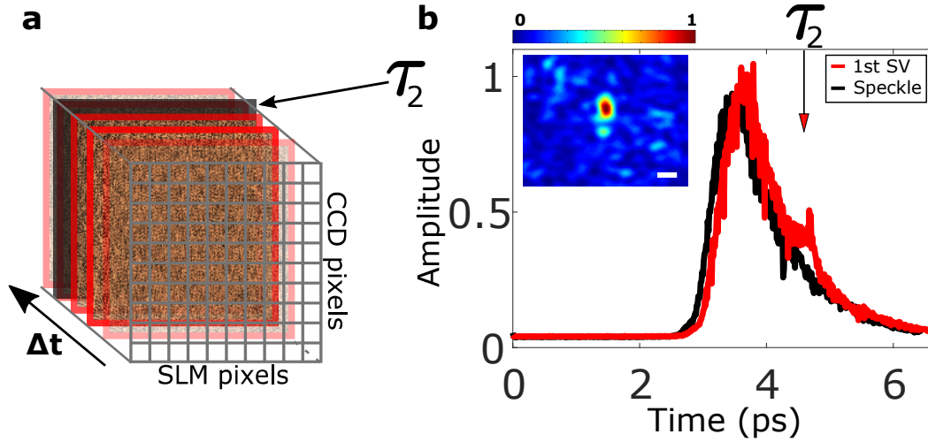
Figure 4.10 – Propagation of the first singular vector, that is associated to the highest singular value of \mathbf{H}(\tau_2) . The scattering medium is characterized by \tau_m \sim 1.1 ps. (a) The TGTm \mathbf{H}(\tau_2) is extracted from the TRTM. Singular vectors are extracted via SVD. (b) Spatially averaged temporal profile of the first singular vector (red), associated to the largest singular value of \mathbf{H}(\tau_2) . As a comparison, the time-of-flight distribution is plotted in black. Top red arrow corresponds to arrival time \tau_2 . Inset: Normalized CCD image of transmitted first singular vector. Scale bar: 2 \mu\text{m} .
