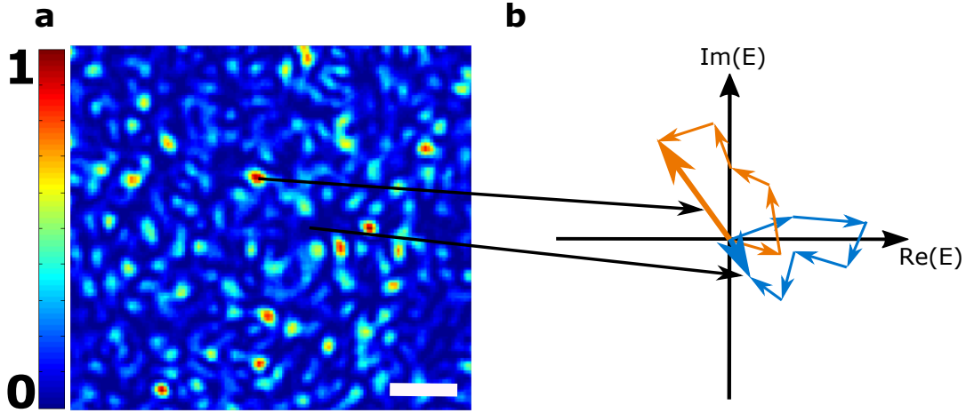
Figure 1.5 – Monochromatic speckle pattern. (a) When monochromatic coherent light is propagating through a scattering medium, interferences between different optical paths give rise to a so-called speckle pattern. In the image: intensity speckle measured with a CCD camera after propagation of continuous wave light through a layer of white paint. Scale bar: 5 \mu\text{m} . (b) Simplified representation in the complex plane of the electric field resulting from light scattering in a dark grain (blue) and in a bright grain (orange). Magnitude of the resulting electric field is amplitude of the sum of random phasors.
