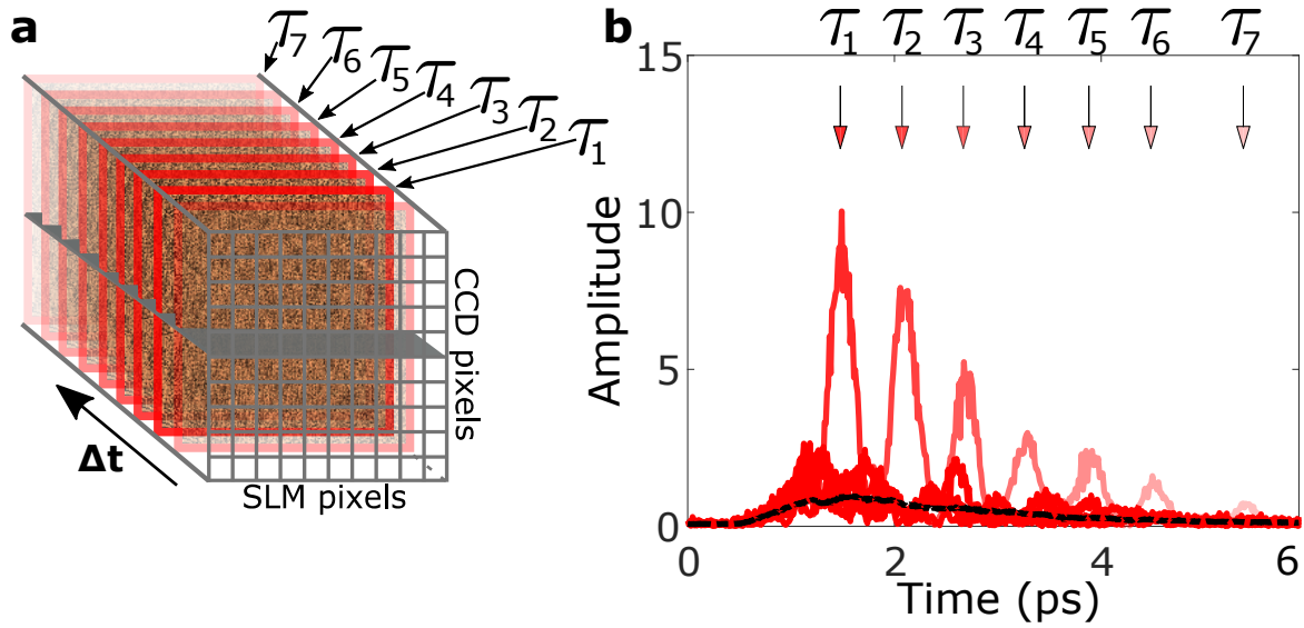
Figure 4.4 – Spatio-temporal focusing with different single time-gated Transmission Matrices, at different delay times. Spatio-temporal control of light with the Time-Resolved Transmission Matrix, that was measured with N_{\text{SLM}} = 256 SLM pixels. (a) Simplified scheme of the TRTM. 7 individual time-gated transmission matrices are selected, whose arrival times are distributed between \tau_1 = 1.5 ps and \tau_7 = 5.4 ps. (b) Superposition of temporal profiles acquired with ICC measurement, using spatio-temporal focusing processes at the same output position and different arrival times (colored arrows). The time-of-flight distribution is used as a reference temporal profile (black curve).
