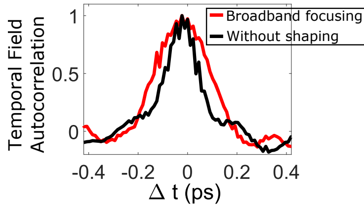
Figure 5.5 – Temporal field autocorrelation when focusing with the Broadband transmission matrix. Temporal field autocorrelation of both (red) focus averaged over 25 different foci and (black) without shaping averaged over 200 speckle grains. We arbitrarily chose the reference arrival time \tau = 3 ps from the set of data presented in Figure 5.3c and Figure 5.3d, which corresponds then to \Delta t = 0 . The temporal width of the autocorrelation peak for the focus is broader than without shaping: \delta t_f > \delta t_m .
