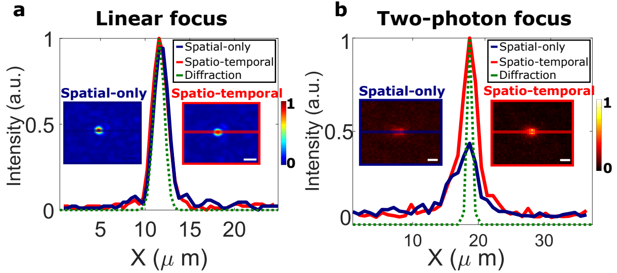
Figure 6.4 – Intensity profiles of both linear and two-photon focus positions, for both spatial-only focusing and spatio-temporal focusing, with the MSTM. Intensity profile of the images from Figure 6.3 are analyzed. (a) Intensity profiles of the linear ( \lambda_L = 800 nm) focus for spatial-only (blue line) focusing and spatio-temporal (red line) focusing. Expected diffraction limit (green line) is fitted with a Gaussian function, with \lambda_L/(2NA) = 1\mu\text{m} at FWHM, with NA=0.4 . Inset: corresponding CCD images. (b) Intensity profiles of the 2-photon ( \lambda_{NL} \simeq 500 nm) focus for spatial-only (blue line) focusing and spatio-temporal (red line) focusing. Expected diffraction limit (green line) is fitted with a Gaussian function, with \lambda_{NL}/(2NA) \simeq 600 nm at FWHM, with NA=0.4 . Inset: corresponding EMCCD images. Scale bar: 5\mu\text{m} .
