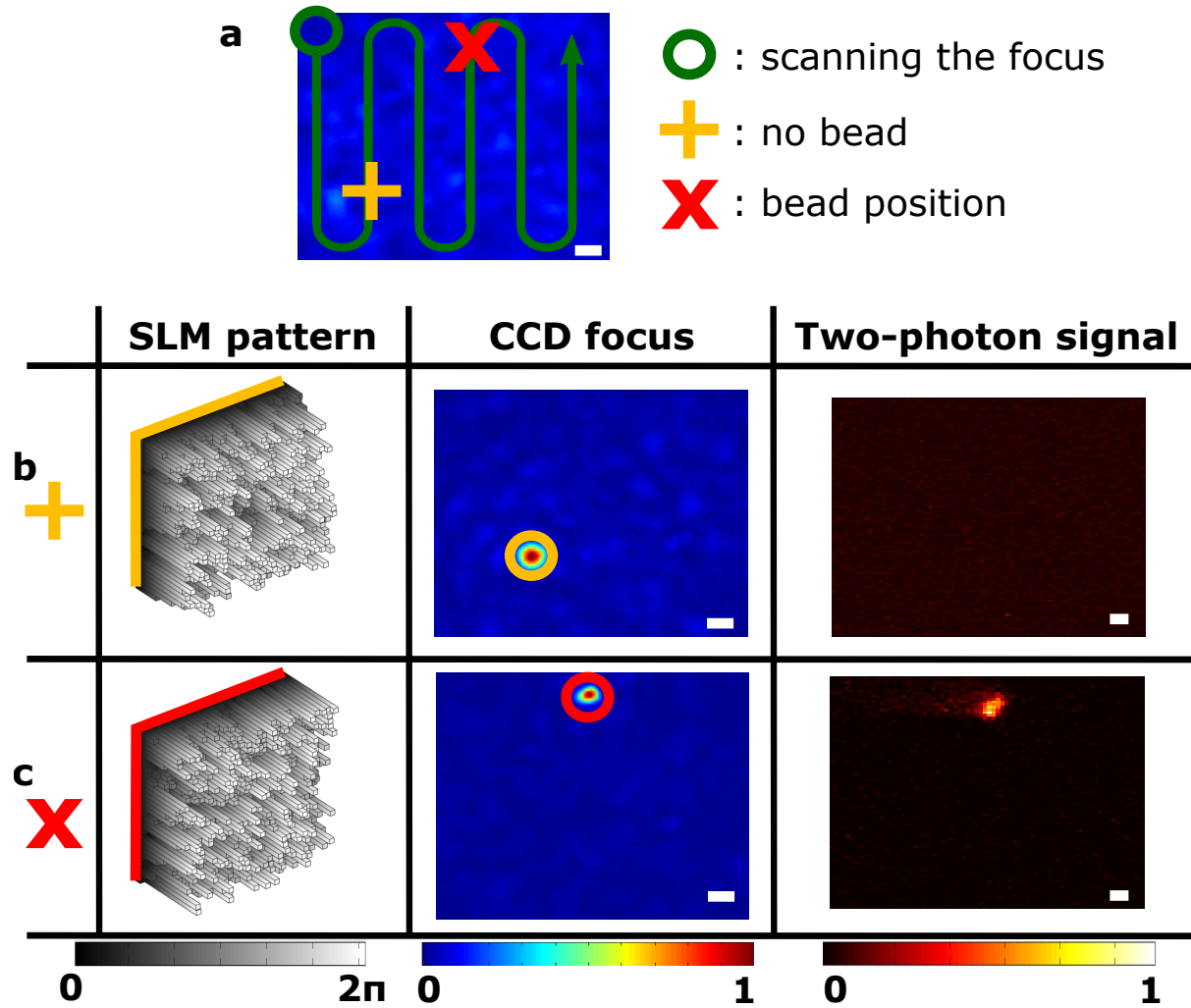
Figure 6.9 – Protocol for point-scanning imaging of fluorescent beads, using a single time-gated transmission matrix. A single time-gated matrix \mathbf{H}(\tau) , of a thick scattering medium, is measured. \tau corresponds to the delay time where the time-of-flight distribution reaches its maximum. First column: SLM input pattern. Second column: CCD image when focusing with \mathbf{H}(\tau) . Third column: corresponding two-photon signal measured on the EMCCD camera. (a) (Green line) The achieved focused is scanned, using the phase-conjugation of \mathbf{H}(\tau) in all the output spatial positions. The corresponding spatially-integrated two-photon signal is recorded on the EMCCD camera. (b) (Yellow + of (a)) No microbead is detected for this focus position. (c) (Red x in (a)) Example of focusing on a microbead: two-photon signal is detected on the EMCCD camera. Scale bars: 2\ \mu\text{m} .
