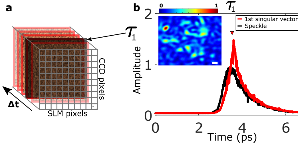
Figure 4.8 – Propagation of the first singular vector, associated to the highest singular value of \mathbf{H}(\tau_1) . The scattering medium is characterized by \tau_m \sim 1.1 ps. (a) The TGTm \mathbf{H}(\tau_1) is extracted from the TRTM, which was measured with N_{\text{SLM}} = 1024 SLM pixels and N_{\text{CCD}} \sim 100 speckle grains. Its SVD is being computed to extract singular vectors. (b) Spatially averaged temporal profile of the first singular vector (red), associated to the largest singular value of \mathbf{H}(\tau_1) . As a comparison, the time-of-flight distribution is plotted in black. Top red arrow corresponds to arrival time \tau_1 . Inset: Normalized CCD image of transmitted first singular vector. Scale bar: 2 \mu\text{m} .
