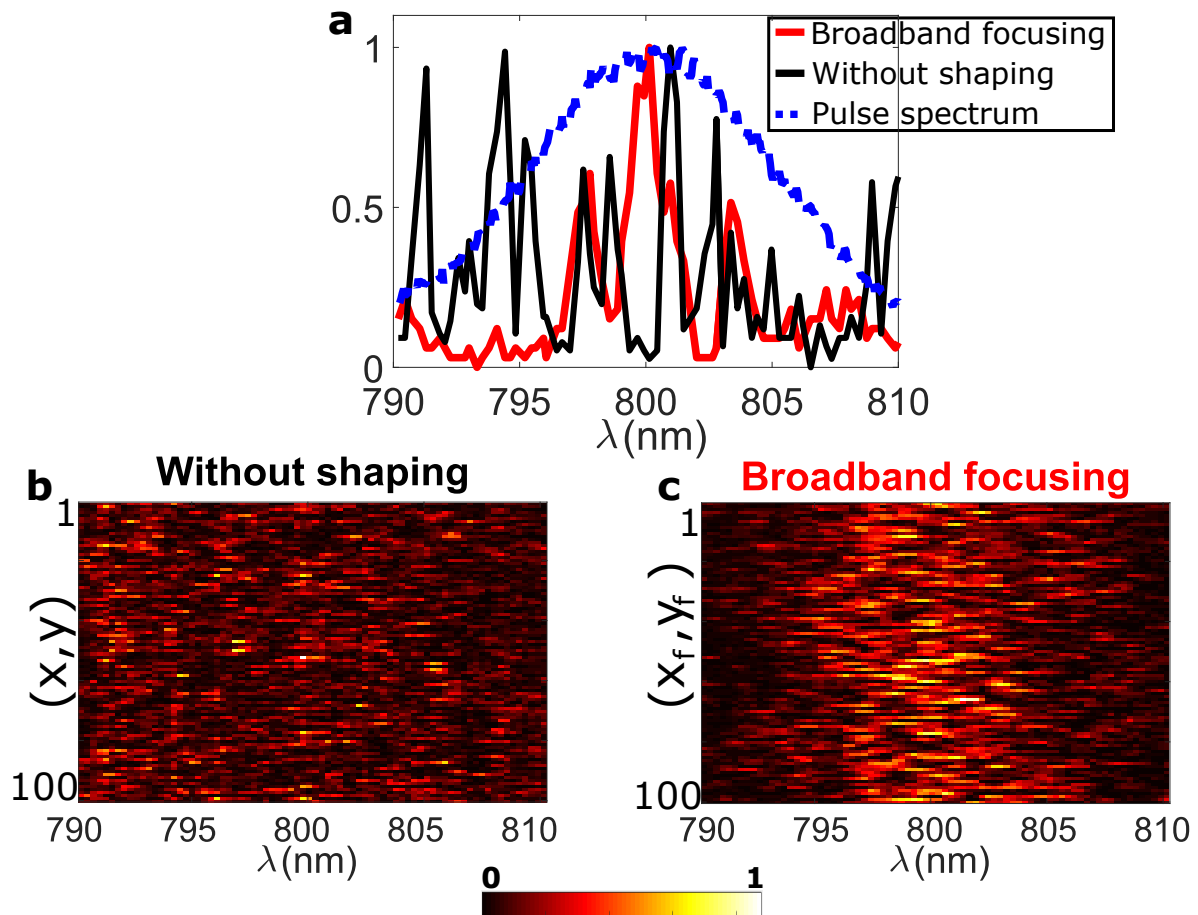
Figure 5.6 – Spectral intensity measurement when focusing with the Broadband transmission matrix. (a) Spectral intensity measurement. Monochromatic intensity in a single grain (with or without shaping) is recorded on a CCD camera as function of \lambda with a tunable cw laser. Plots are spectral intensities (black) without wavefront shaping, and (red) at the focus. (blue) Intensity spectrum of the input pulse is recorded with a spectrometer at the output of the laser. (b-c) Monochromatic intensity over 100 different spatial positions (x, y) either without shaping (in (b)) or in different focus positions (x_f, y_f) (in (c)) with the same scattering sample. Color-map stands for the spectral intensity at a chosen spatial position and incident wavelength.
