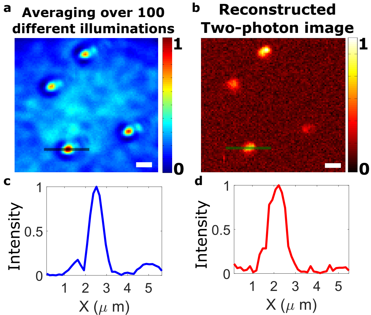
Figure 6.10 – Experimental results of point-scanning imaging of fluorescent beads, using a single time-gated transmission matrix. (a) Mean linear speckle image, obtained by averaging over 100 different random illumination patterns on the SLM, measured with the CCD camera. 4 microbeads are observed in the field of view. Scale bar: 2\ \mu\text{m} . (b) Reconstructed two-photon image with the point-scanning imaging technique. Scale bar: 2\ \mu\text{m} . (c) Intensity profile along the black line of (a). (d) Intensity profile along the green line of (b).
