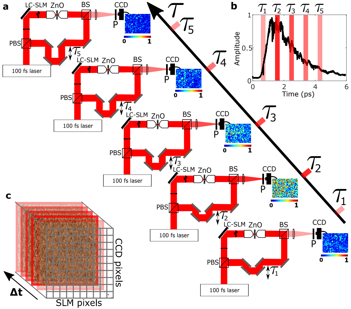
Figure 4.1 – Time-Resolved Transmission Matrix measurement. N_\lambda stands for the number of temporal degrees of freedom. Only 5 time-gated transmission matrices (TGTMs), measured at delay time ( \tau_a ) are represented for clarity. (a) Measurement of the Time-Resolved Transmission Matrix (TRTM) is discretized: N_\lambda TGTMs are measured, at different arrival times ( \tau_a ) that are separated to each other by \delta t the duration of the input ultrashort pulse. \tau_a is set by adjusting the delay line position, in the external reference arm. Cross-product between the transmitted output pulse and the delayed reference pulse, that is proportional to TGTMs coefficients, is represented on the CCD camera for a flat pattern on the SLM. Color-bar and amplitude are normalized to maximum of cross-product at time \tau_2 . For each fixed delay line position at time ( \tau_a ), the matrix is measured by setting a series of N_{\text{SLM}} pattern on the SLM, and measuring the corresponding output field with phase-stepping holography. (LC-SLM) : Liquid-Crystal Spatial Light Modulator; (PBS): Polarized Beam Splitter; (BS): Beam Splitter; (P): Polarizer; (CCD): Charged Coupled Device; (ZnO): Zinc Oxide scattering medium. (b) Typical time-of-flight distribution of photons in the ZnO scattering medium, measured with Interferometric Cross-Correlation. The five delay time ( \tau_a ) are represented on top of the plot. We estimate from this plot \tau_m \sim 2 ps the confinement time of photons in the medium. (c) Typical schematic representation of the Time-Resolved Transmission Matrix, of dimension N_{\text{out}} \times N_\lambda \times N_{\text{SLM}} , where N_{\text{out}} stands for number of CCD pixels, and N_{\text{SLM}} the number of SLM pixels exploited. In practice N_{\text{out}} \sim 10^4 pixels, N_{\text{SLM}} \sim 1024 pixels and N_\lambda \sim 20 temporal degrees of freedom.
