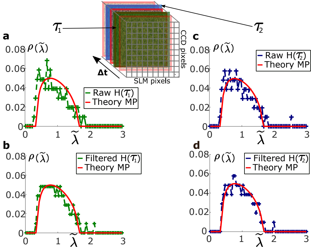
Figure 4.7 – Distribution of normalized singular values of a single time-gated transmission matrix. The full TRTM has been measured with N_{\text{SLM}} = 256 SLM pixels and \gamma = 2.5 , for a thick scattering medium, that is characterized by \tau_m \sim 2 ps. (a) A single TGTM \mathbf{H}(\tau_1) is extracted from the TRTM at arrival time \tau_1 . After binning the output pixel by the typical speckle grain size, leading to a matrix \mathbf{M}(\tau_1) , the distribution of its normalized singular values is plotted (green), in comparison with theoretical prediction from Marcenko-Pastur (MP) law (red). (b) \mathbf{M}(\tau_1) is filtered by normalizing its lines and columns: fidelity with theoretical prediction is improved. c-d The protocol is iterated for an uncorrelated time-gated transmission matrix \mathbf{H}(\tau_2) , that is extracted from the same TRTM, at arrival time \tau_2 .
