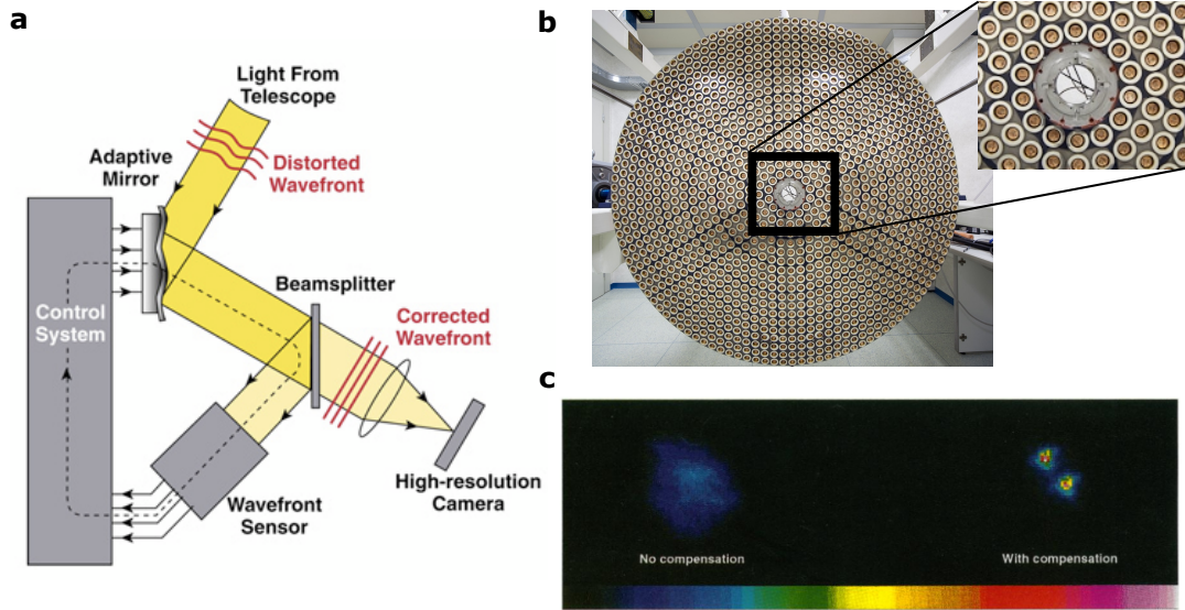
Figure 1.2 – Adaptive optics for astronomy. (a) Principle of adaptive optics in astronomy. The distorted wavefront is measured in real time with a wavefront sensor, connected via a feedback loop to the deformable mirror, blurred by atmospheric turbulence. They adjust correspondingly the wavefront. (Image adapted from Center for Adaptive Optics, UC Santa Cruz) (b) Example of a deformable mirror, diameter 1.1m, used for astronomy in the Very Large Telescope in Chile, composed of around 1000 actuators (Image: European Southern Observatory) (c) Image of a double star with the Come-on-Plus system on the European Southern Observatory. Turning on the adaptive optics algorithm permits to resolve the binary star, that is initially blurred (adapted from [Hubin and Noethe, 1993] )
