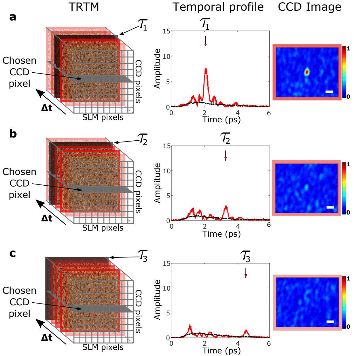
Figure 4.3 – Spatio-temporal focusing with different time-gated transmission matrices. Light is focused in the same spatial position, but at different arrival times. 3 time-gated transmission matrices are extracted from the TRTM, at arrival times \tau_1 = 2.1 ps, \tau_2 = 3.3 ps and \tau_3 = 4.5 ps, that were measured with N_{\text{SLM}} = 256 SLM pixels. Temporal profiles are retrieved with ICC measurement on the focus position. (a) Phase-conjugation of \mathbf{H}(\tau_1) leads to spatio-temporal focusing at arrival time \tau_1 in the selected spatial position. The target position is visible on the CCD image. (b-c) Spatio-temporal focusing in the same spatial position at times \tau_2 and \tau_3 . Intensity of the focus, detected by the CCD camera, decreases as it follows the time-of-flight distribution for a fixed number of N_{\text{SLM}} SLM pixels. Scale bar: 5 \mu\text{m} .
