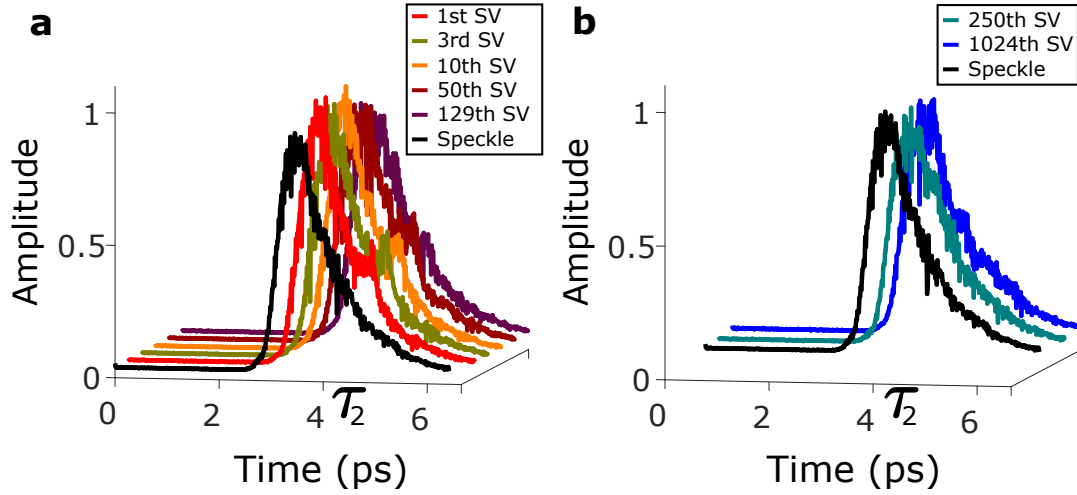
Figure 4.11 – Propagation of singular vectors of \mathbf{H}(\tau_2) . Similarly to \mathbf{H}(\tau_1) , normalized singular values \tilde{\lambda} of \mathbf{H}(\tau_2) are sorted in descending order. In particular for \mathbf{H}(\tau_2) , \tilde{\lambda}_i = 1 for i = 208 . (a) Propagation of singular vectors of \mathbf{H}(\tau_2) , whose associated singular values are larger than unity. (b) Propagation of singular vectors of \mathbf{H}(\tau_1) , whose associated singular values are lower than unity.
