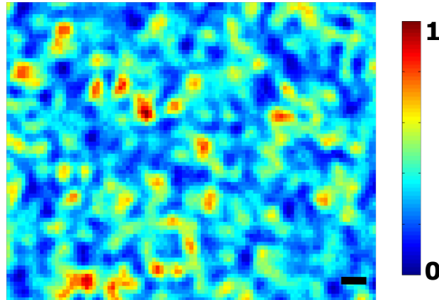
Figure 2.6 – Spatio-temporal speckle spectrally/temporally integrated, measured with an ultrashort short pulse on a CCD camera. Transmitted pulse through ZnO scattering medium is imaged on a CCD camera. The measured intensity pattern corresponds to integration of spatio-temporal speckle over time. This speckle is low contrasted: C=0.22 , corresponding to an incoherent sum of 1/C^2 \sim 20 monochromatic speckles. Scale bar: 2 \mu\text{m} .
