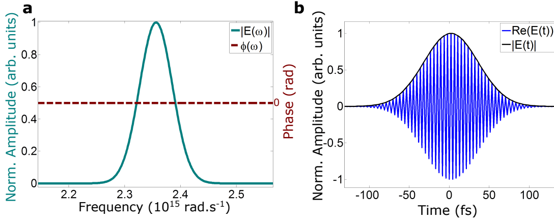
Figure 1.13 – Typical ultrashort pulse of light. Spectral and temporal characteristics of a typical ultrashort pulse. (a) Spectral amplitude and spectral phase of the electric field E(\omega) , with a center wavelength \lambda_0=800 nm and a bandwidth of the intensity spectrum \Delta\omega/\omega_0=0.02 . This ultrashort pulse is Fourier-limited as its spectral phase is flat. (b) Corresponding temporal profile of the pulse, obtained with an inverse Fourier transform. Blue line represents the real part of the electric field, while the black line stands for the Gaussian envelope in the time domain. The intensity pulse duration is \Delta t \simeq 70 fs.
