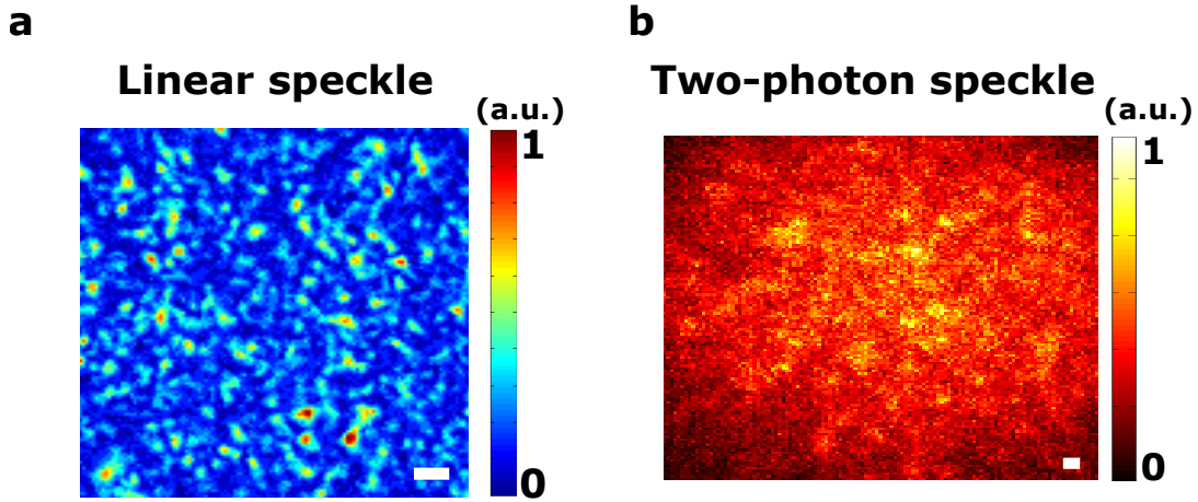
Figure 6.1 – Two-photon speckle pattern from fluorescein within a two-photon screen. A random pattern is displayed on the SLM. The scattering medium is characterized by \tau_m \sim 500 fs. A capillary of thickness 20 \mu\text{m} , filled with fluorescein, is inserted in the experimental setup. Transmitted light is collected with a microscope objective ( \times 20 , \text{NA}=0.4 ). Linear signal (speckle at \lambda = 800 nm) and non-linear signal (fluorescence at \lambda = 400 - 600 nm) are separated with a dichroic mirror. (a) “Linear” speckle pattern recorded with the CCD camera, after propagation through the scattering medium and the two-photon screen. (b) Corresponding fluorescence pattern, revealing a two-photon speckle, measured on the EMCCD camera, with a gain 300 and exposure time T_e = 2 s. Scale bars: 5 \mu\text{m} .
