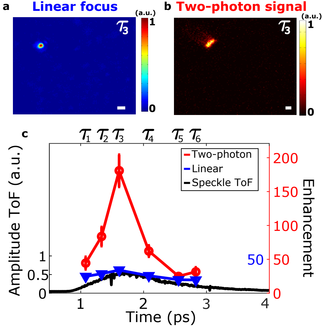
Figure 6.5 – Spatio-temporal focusing with a time-gated transmission matrix H(\tau) : two-photon signal-to-background ratio as a function of arrival time \tau . Two-photon signal is emitted from fluorescent microbeads after propagation through a thick scattering sample. (a) Temporally-integrated linear focus at arrival time \tau_3 (see (c)), measured with the CCD camera, on a microbead. Scale bar: 2\ \mu\text{m} . (b) Corresponding two-photon signal, measured with the EMCCD camera. Scale bar: 2\ \mu\text{m} . (c) Black line represents the time-of-flight distribution of photons in the scattering medium. 6 time-gated transmission matrices (TGTM) are measured at arrival times \tau_i , with i varying from 1 to 6, that are indicated on top. We focus on 9 different beads with each TGTM: the average linear (blue) and two-photon (red) are both shown, at their corresponding \tau_i . Error bars are the corresponding standard deviation.
