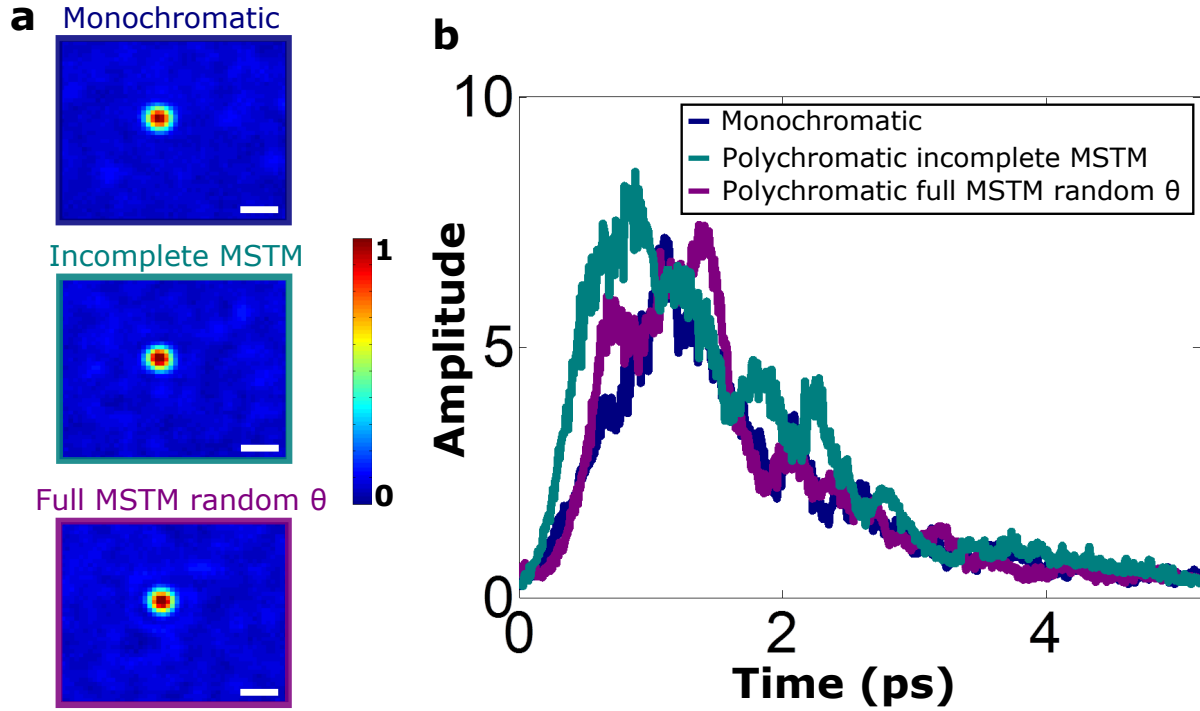
Figure 3.7 – Temporal profiles of spatial-only focusing of an ultrashort pulse via the MSTM.
