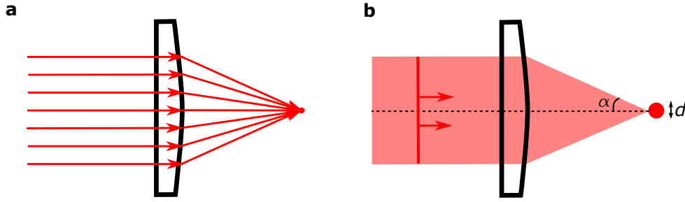
Figure 1.1 – Diffraction-limited spot. Focusing light with a lens. (a) Using ray optics, parallel arrows represent an incoming plane wave. The achieved spot has an infinitely small width. (b) In reality, for a perfect lens, the spot width is diffraction-limited, with a diameter d
