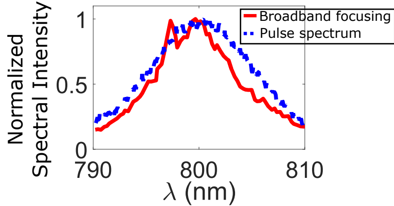
Figure 5.7 – Averaged spectral intensity of the achieved focus with the Broadband transmission matrix. (red) The averaged spectral intensity of focusing, via the BBTM, is obtained by averaging monochromatic intensity as a function of incident wavelength over 100 different focus positions. (blue) It is compared to the intensity spectrum of the input pulse, recorded with the spectrometer. On average, the output pulse has a narrower spectrum than the input pulse
