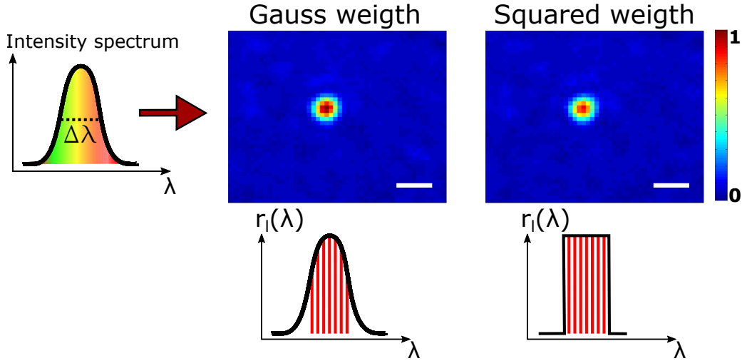
Figure 3.6 – Multi-Spectral focusing of all the spectral components of the ultrashort pulse.
