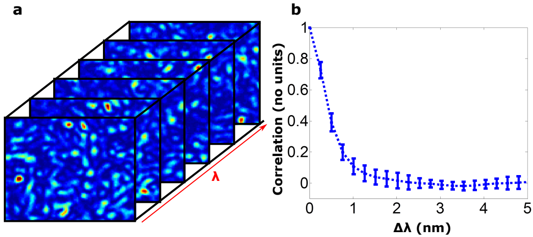
Figure 2.4 – Spectral correlation bandwidth of typical ZnO scattering samples. (a) A stack of monochromatic speckle patterns is recorded as function of illumination wavelength, using tunable cw laser. (b) 2D-correlation between monochromatic images C_\lambda as function of spectral detuning. Spectral correlation bandwidth of the scattering medium \delta\lambda_m is defined as C_\lambda(\delta\lambda_m) = 0.5 by convention.
