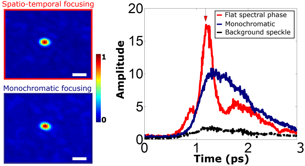
Figure 3.9 – Spatio-temporal focusing is achieved with the MSTM via imposing a flat spectral phase at a given output spatial position. The MSTM was measured with N_{\text{SLM}} = 1024 SLM pixels for N_{\lambda} = 21 wavelengths. (left) CCD images when displaying on the SLM a phase pattern to impose either a flat spectral phase for all the spectral components of the pulse (top, red square) or phase-conjugating the central frequency of the pulse (bottom, blue square). Both images are sharing the same color-map. The two focus have similar signal-to-background ratio of focusing \sim 19 . (right) Temporal profiles of the two focus, retrieved with Interferometric Cross-Correlation. Data are averaged over 9 different spatial positions. Imposing a flat spectral phase leads to spatio-temporal focusing of the output pulse, almost back to its initial duration ( \sim 150 fs at FWHM), at the delay time where the MSTM has been measured (top red arrow). Scale bar: 3 \mu\text{m} .
