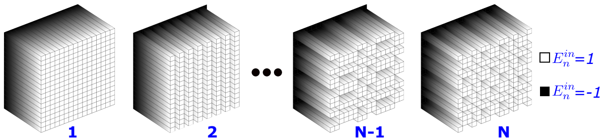
Figure 1.11 – Monochromatic transmission matrix of a scattering medium. (Top) Monochromatic light is transmitted through a spatial light modulator (SLM) before propagating inside a thick scattering medium. Transmitted light is collected with a sensor, usually a CCD camera. While modulating the input field E^{in} on the SLM, the corresponding output field E^{out} is measured using holographic method on the CCD camera. The linear relationship connecting E^{in} and the measured E^{out} is the Transmission Matrix of the scattering medium. (Bottom) The input basis used for the measurement of the Transmission Matrix is the Hadamard basis. Some patterns are represented for N = 256 input SLM pixels. All the pixels have the same intensity distribution, nonetheless half of them are \pi phase-shifted with respect to the other half.
