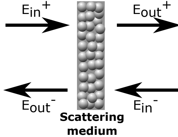
Figure 1.6 – Scattering matrix. Light scattering can be described with the Scattering Matrix \mathbf{S} that gives the relationship between the input field (either on the left side E_{in}^+ or on the right side E_{in}^- ) and the output field (either on the left side E_{out}^- or on the right side E_{out}^+ )
