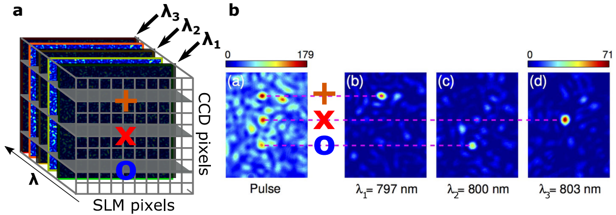
Figure 3.8 – Turning the scattering medium into a controllable grating. Multi-Spectral focusing of 3 different spectral components ( \lambda_1, \lambda_2, \lambda_3 ) within an ultrashort pulse spectral bandwidth, in 3 different spatial positions (+, x, and o). (a) The 3 corresponding monochromatic TMs (black planes) are extracted from the MSTM. The SLM pattern corresponds to the phase of incoherent superposition of three solutions. Each one of them is obtained by phase-conjugating a chosen line (one of the three symbols corresponding to horizontal cross-sections that are represented with gray planes): each wavelength is spatially focused in a different position. (b) When the ultrashort pulse is sent through the scattering medium, 3 spatial focus are observed. While the same pattern is displayed on the SLM, the laser is turned to tunable CW source. The 3 images are measured respectively at \lambda_1, \lambda_2 and \lambda_3 . Each focus corresponds to an individual focus, whose position is represented with dashed line in accordance with selected cross-sections in the MSTM. The medium is thus used as a controllable dispersive element. Image adapted from [Andreoli et al., 2015].
