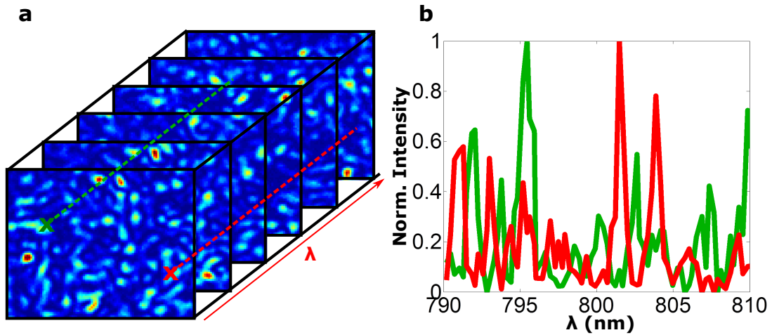
Figure 2.7 – Spectral content of a spatio-temporal speckle, measured with tunable cw light and a CCD camera. A random input pattern is displayed on the SLM. (a) Similarly to Figure 2.4, monochromatic speckle images are recorded for the different spectral components, over a spectral interval corresponding to the input pulse spectrum. (b) Monochromatic intensity in two different spatial positions ( x in (a)) is plotted as function of illumination wavelength. Spectral intensity is fluctuating, with characteristic feature \delta\lambda_m corresponding to the spectral correlation bandwidth of the scattering medium.
