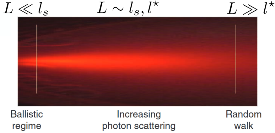
Figure 1.4 – Light propagation in scattering media. Light scattering with increasing thickness of the medium L from left to right at fixed scattering mean free path l_s . In the ballistic regime, light has suffered, in average, less than a scattering event. Increasing L enhances the number of scattering events up to the multiple scattering regime, analogue to a random walk. Image adapted from [Ntziachristos, 2010]
