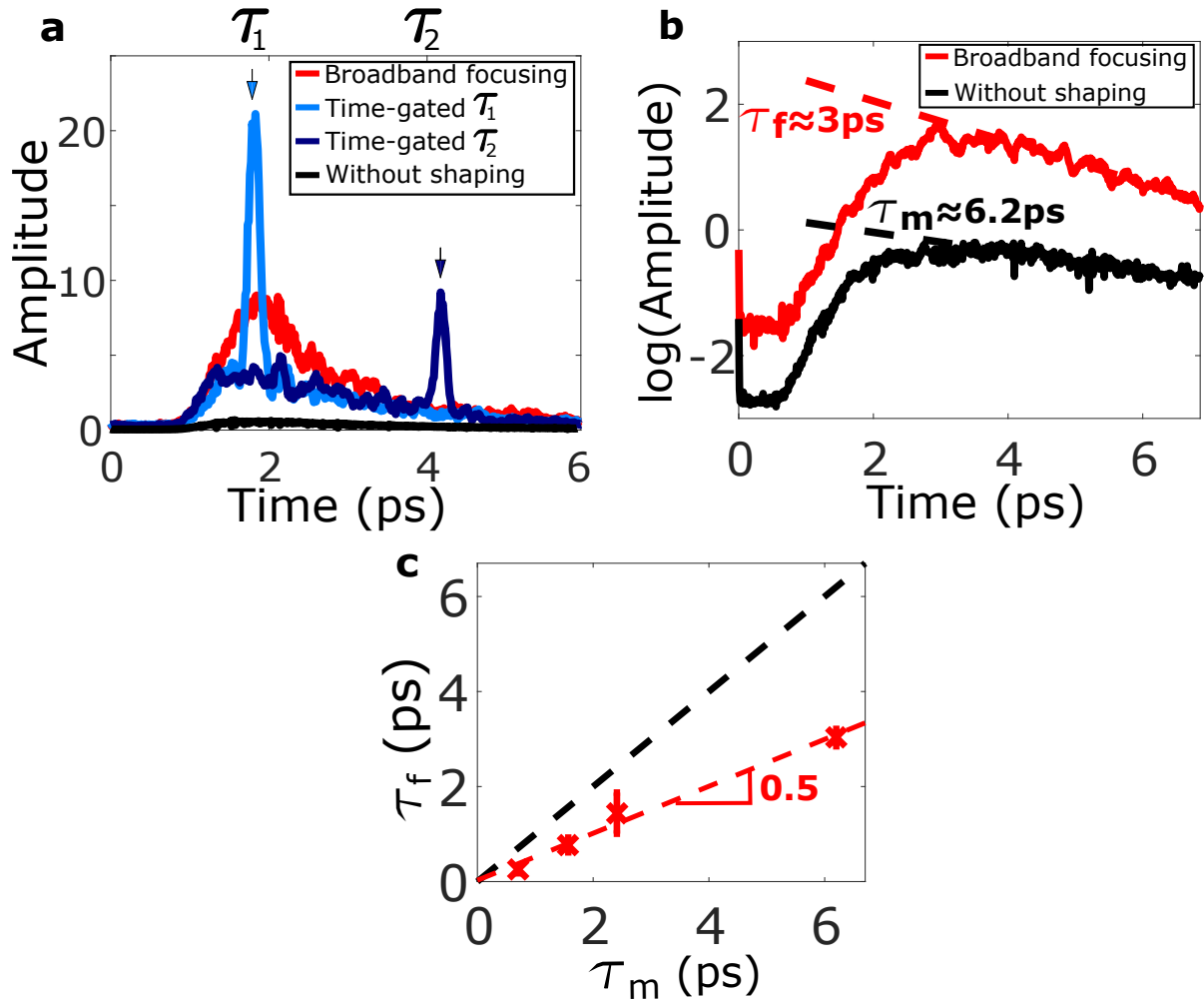
Figure 5.4 – Averaged temporal profiles of focusing with the Broadband transmission matrix. (a) Comparison of averaged temporal profiles when focusing with the Broadband transmission matrix (red) and two single time - gated transmission matrices (blue) measured respectively at delay time \tau_1 and \tau_2 with the external reference arm, with the same number of SLM pixels ( N_{\text{SLM}} = 1024 ). Data are averaged over 9 focus. Time-of-flight distribution of the scattering medium is obtained via averaging over 200 temporal envelop of speckle grains without wavefront shaping (black): we retrieve \tau_m \sim 2.5 ps for this scattering sample. (b) Averaged time-of-flight distributions over 25 different foci plotted in semilog of a thicker scattering sample. \tau_m (without shaping, black line) and \tau_f (broadband focusing, red line) are measured with a linear fit. (c) Comparison between \tau_m and \tau_f for various scattering samples. While dashed black line represents the expected \tau_m = \tau_f , experimental data (red markers) evidences \tau_f is twice smaller than \tau_m . Red dashed line represents a linear fit and error bars indicate the standard deviation for estimation of \tau_f .
