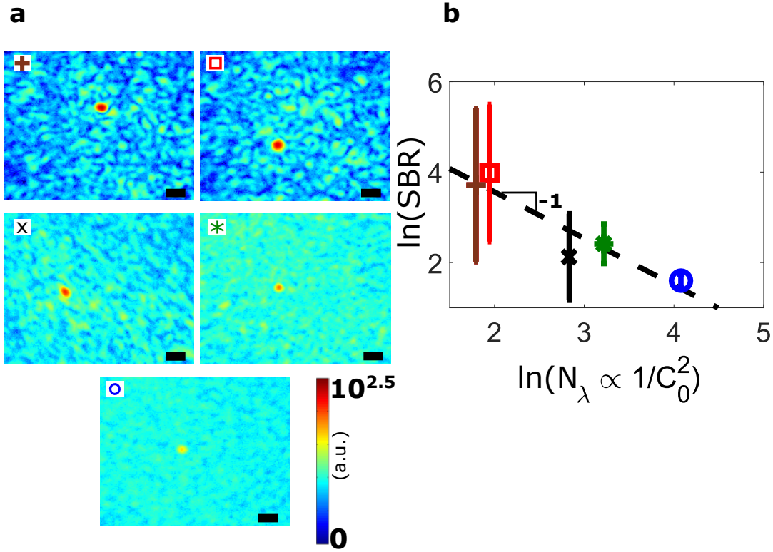
Figure 5.2 – Signal-to-background ratio of focusing with the Broadband transmission matrix. Phase-conjugation of the BBTM enables spatial focusing in a given speckle grain, whose efficiency is inversely related to N_\lambda . (a) The images show the results for 5 different scattering samples whose spectral degrees of freedom N_\lambda \propto 1/C_0^2 , with C_0 the contrast of transmitted speckle without shaping, are indicated with corresponding markers in (b). The color bar is in log scale. Scale bar: 2 \mu\text{m} . (b) Log of signal-to-background-ratio (SBR) is plotted as a function of \log(N_\lambda) . Error bars are standard deviation for SBR over 50 different focus positions. Dashed line: linear fit, with a -1 slope.
