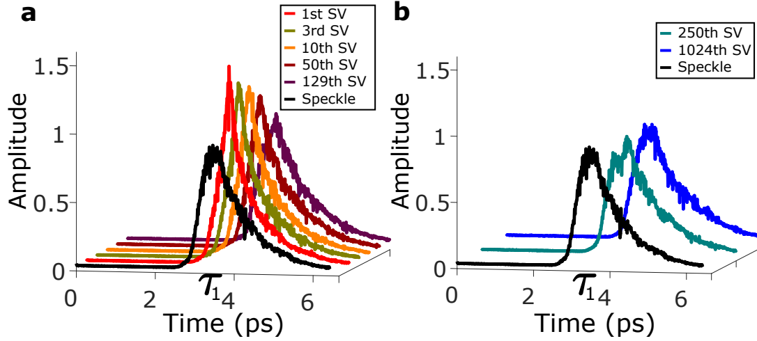
Figure 4.9 – Propagation of singular vectors of \mathbf{H}(\tau_1) . Normalized singular values \tilde{\lambda} of \mathbf{H}(\tau_1) are sorted in descending order. In particular for \mathbf{H}(\tau_1) , \tilde{\lambda}_i = 1 for i = 166 . (a) Propagation of singular vectors of \mathbf{H}(\tau_1) , whose associated singular values are larger than unity. (b) Propagation of singular vectors of \mathbf{H}(\tau_1) , whose associated singular values are lower than unity.
