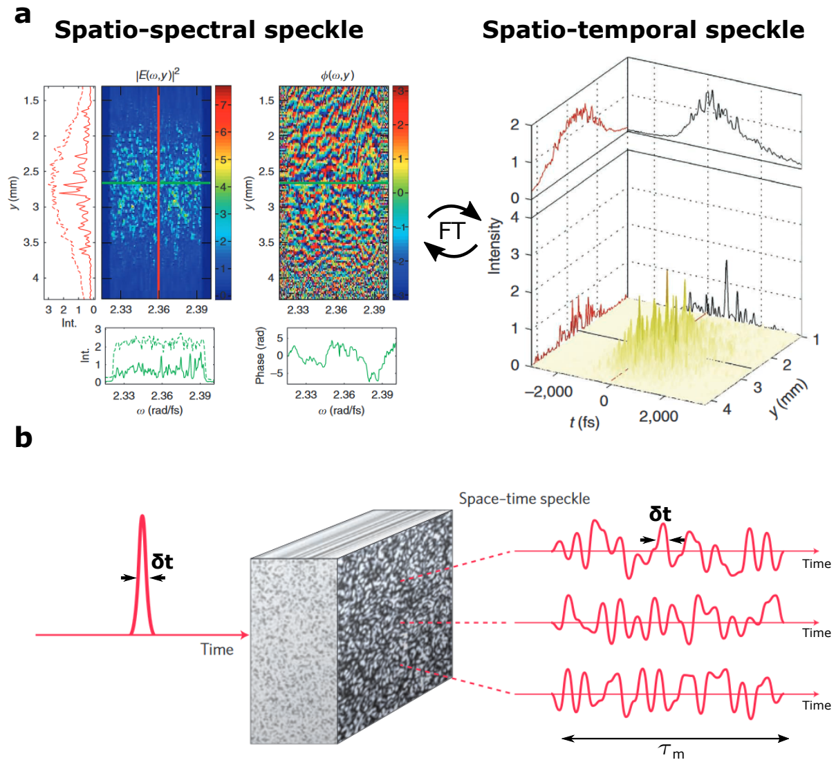
Figure 1.18 – Spatio-temporal/spectral speckle. Propagation of an ultrashort pulse of light through a thick scattering medium leads to both spatial and temporal distortions of light. The corresponding spatio-spectral/temporal speckle pattern results from coupling between spatial and spectral/temporal channels. (a) The associated field of the spatio-spectral speckle can be obtained with spatially and spectrally resolved interferometry techniques. Once amplitude and phase are known, a Fourier transform gives access to the spatio-temporal speckle. (b) In the temporal domain, a short Fourier-transform limited ultrashort pulse of duration \delta t is temporally distorted. The temporal profile is different in every output spatial position. This “temporal speckle” smallest feature has a duration equal to the duration of the input pulse. The transmitted pulse is stretched over a temporal interval \tau_m , which corresponds to the averaged confinement time of photons inside the scattering medium. Averaging this temporal speckle over spatial position leads to the time-of-flight distribution presented in Figure 1.16. Images adapted from (a) : [McCabe et al., 2011]; (b) : [Weiner, 2011].
