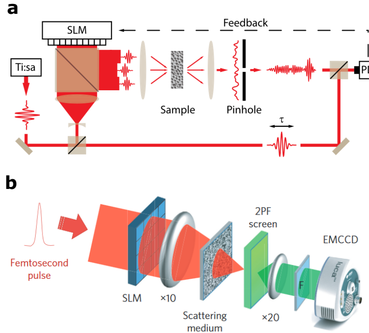
Figure 1.22 – Iterative optimization algorithm with a short pulse for spatio-temporal focusing. Different feedback-based algorithm have been employed. (a) With linear heterodyne feedback (b) With two-photon fluorescence feedback. Images adapted from: (a) : [Aulbach et al., 2011]; (b) : [Katz et al., 2011]
