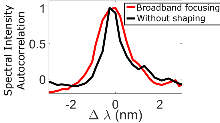
Figure 5.8 – Spectral intensity autocorrelation when focusing with the Broadband transmission matrix. Spectral intensity autocorrelation of both (red) focus averaged over 100 different foci and (black) without shaping averaged over 200 speckle grains. We arbitrarily chose the reference wavelength \lambda_0 = 800 nm the central wavelength of the pulse, from the set of data presented in Figure 5.6b and Figure 5.6c, which corresponds then to \Delta\lambda=0 . The spectral width of the autocorrelation function for the focus is broader than without shaping: \delta\lambda_f > \delta\lambda_m .
