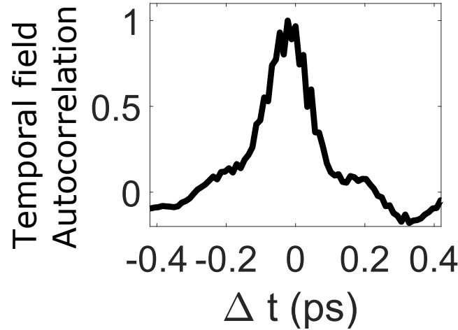
Figure 2.9 – Temporal field autocorrelation of the temporal envelope retrieved via ICC. 100 different temporal envelopes, retrieved via ICC, are stored in lines of a 2D array. Temporal autocorrelation is retrieved by calculating the inner products of columns, with a reference arrival time arbitrary chosen at \tau = 1.2 ps (See Figure 2.8), corresponding to the maximum of the time-of-flight distribution. Time-width of this autocorrelation gives the duration of smallest feature of the temporal speckle, that is \sim the duration of the input pulse \delta t \sim 100 fs.
