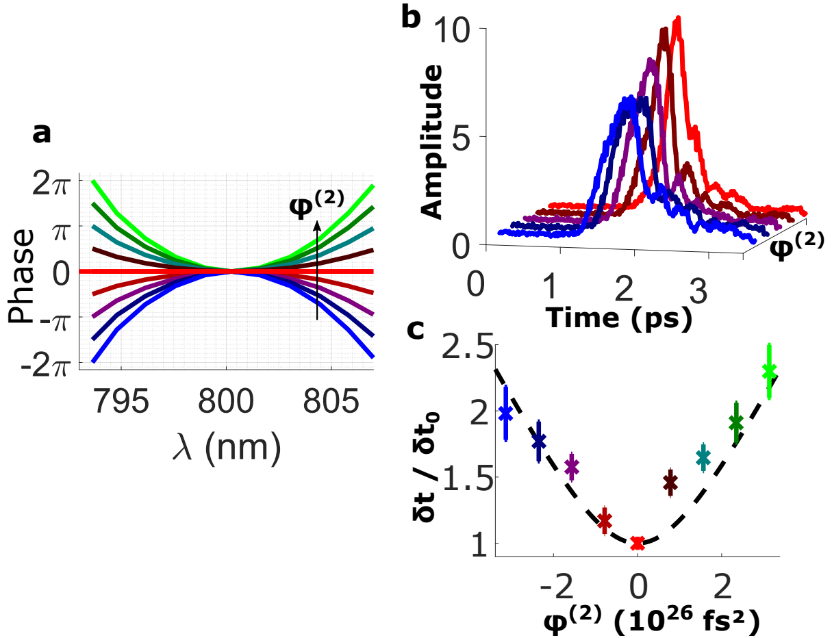
Figure 3.12 – Adjustable chirped pulse via a quadratic spectral phase distribution with the full MSTM. A quadratic spectral phase can be implemented in E_{target}^{out}(\lambda) : we deliberately add group velocity dispersion to the output pulse. The MSTM is measured here on a scattering sample characterized by \tau_m \sim 1 ps: the MSTM contains then N_\lambda = 11 monochromatic TMs, with N_{SLM} = 1024 SLM pixels. (a) 9 different quadratic spectral phase distributions ( \theta_l ) are applied on E_{target}^{out}(\lambda) , for different values of chirp \phi^{(2)} . (b) For each chirp, the temporal profile, measured with ICC technique, is averaged over 9 focus positions. In the plot we only display 4 averaged temporal profiles (for clarity), for negative chirps and (red) the flat spectral phase temporal profile. Duration of the corresponding chirped pulses \delta t are extracted. (c) \delta t is plotted for the different \phi^{(2)} . We note \delta t_0 \sim 200 fs the duration of the measured flat spectral phase pulse. Theoretical prediction of \delta t / \delta t_0 is plotted in black dashed line.
