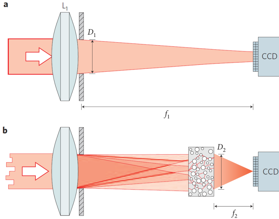
Figure 1.8 – Wavefront shaping turns a disordered material into a scattering lens. (a) Lens L_1 with focal distance f_1 focuses light onto a camera. A pinhole controls the aperture D_1 of the lens. The focus is, at best, as sharp as the diffraction limit of the lens. (b) A disordered medium at distance f_2 from the camera scatters light. After wavefront shaping, light is focused through the sample to a spot that is narrower than the diffraction limit of the lens. D_2 : diameter of the diffuse spot at the back of the sample. Image adapted from [Vellekoop et al., 2010].
