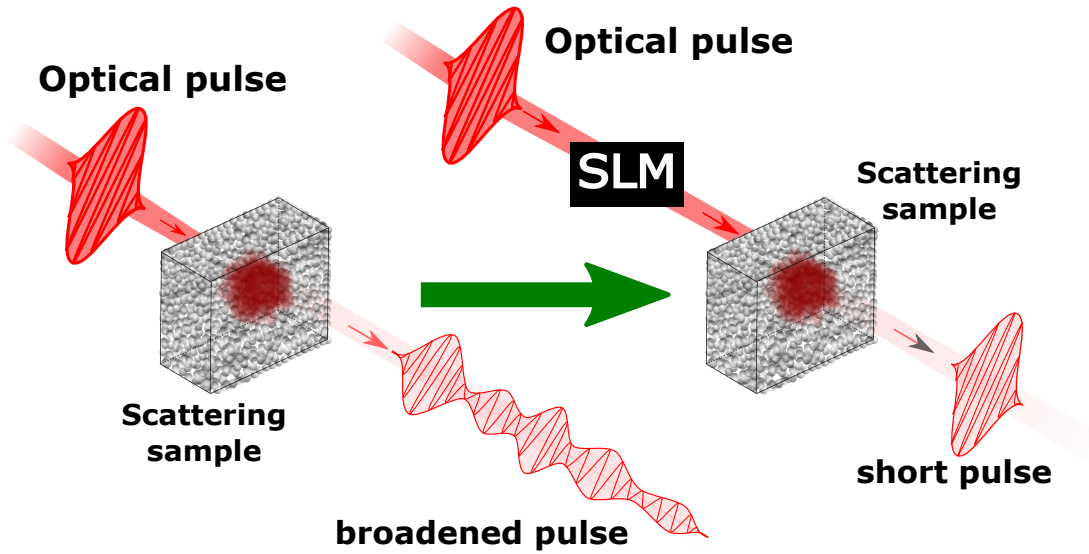
Figure 2 – Extension of wavefront shaping to the temporal control of an ultrashort pulse through scattering media. (Left) An ultrashort pulse is propagating through a thick scattering sample. Temporal profile of the transmitted pulse is significantly broadened because of scattering effects. (Right) A spatial-only control of the input pulse, via a spatial light modulator (SLM) enables temporal recompression of the output pulse almost back to its initial duration. In this thesis , we develop different transmission matrix approaches to compute the corresponding pattern to be displayed on the SLM.
