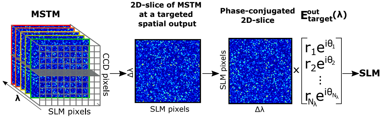
Figure 3.5 – Algorithm for Multi-Spectral focusing in the same spatial position via the MSTM. Scheme of the algorithm used to arbitrary shape the output pulse at a given output position. Both amplitude ( r_k ) and phase ( \theta_k ) relations between the N_\lambda wavelengths are imposed at the output of the scattering medium by the user, and the corresponding input is calculated. Incomplete MSTM allows proper spatio-spectral control only of spectral amplitude, while full MSTM enables spatio-temporal control of the output pulse via spectral phase adjustment.
