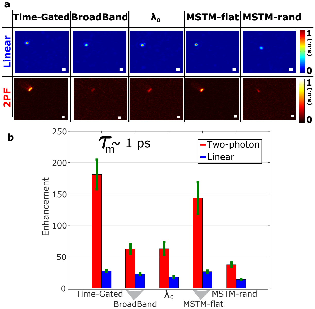
Figure 6.8 – Comparison of two-photon signals between the different transmission matrices, for a “thick” multiple scattering medium. Similar caption than in Figure 6.7, except the scattering medium is now described by \tau_m \sim 1 ps.
