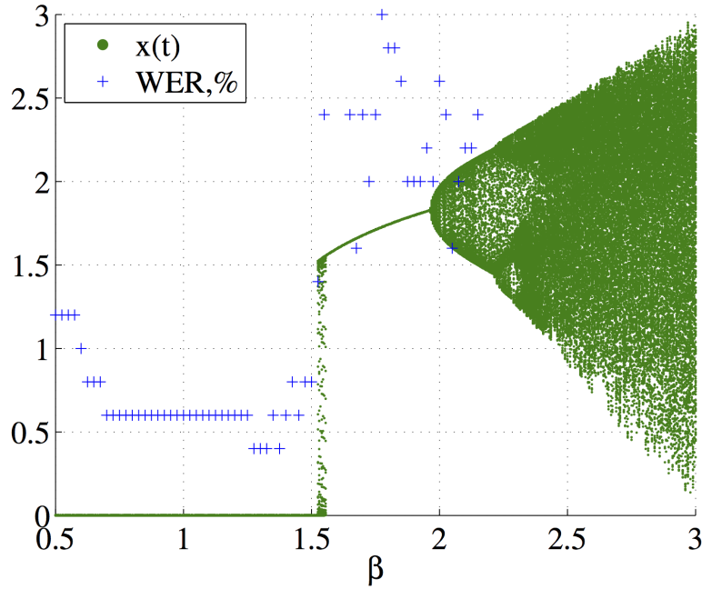
Figure 3.4.5: Accuracy of speech recognition in terms of WER (blue crosshairs) depending on the control parameter \beta and corresponding bifurcation diagram (green dots) of Ikeda delay dynamics underlying RC.
