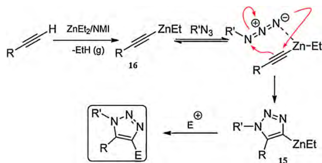
Fig. 19. Proposed mechanism explaining the reactivity in the system mediated by \text{ZnEt}_2 .
