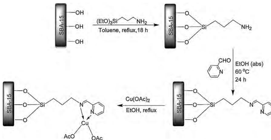
Fig. 25. Synthesis of the Cu@PyIm-SBA-15 catalyst.
