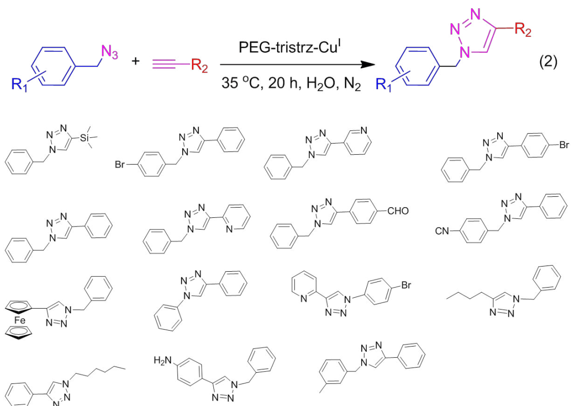
Figure 12. Substrate scope of CuAAC reactions between various azides and alkynes using the PEG-tris-trz-Cu I catalyst.
