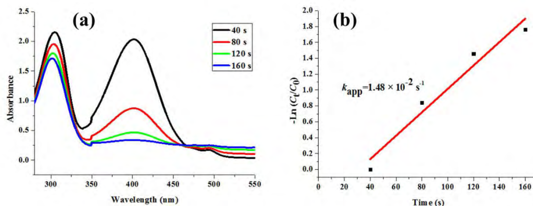
Figure 2. (a) UV-vis. spectra of the 4-NP reduction by NaBH 4 catalyzed by RhAg 0.5 /rGO (top); (b) consumption rate of 4-NP: -\ln(C_t/C_0) vs. reaction time .
