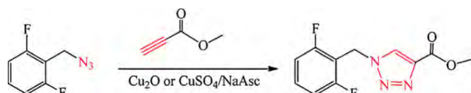
Fig. 27. AAC reactions catalyzed by Cu 2 O-NP and CuSO 4 /NaAsc. Reproduced with permission from Ref. [142]. Copyright 2013, Elsevier B.V.
