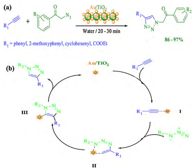
Fig. 14. (a) Titania-supported gold nanostructure-catalyzed 1,2,3-triazole synthesis. (b) Plausible mechanism for the formation of triazole.
