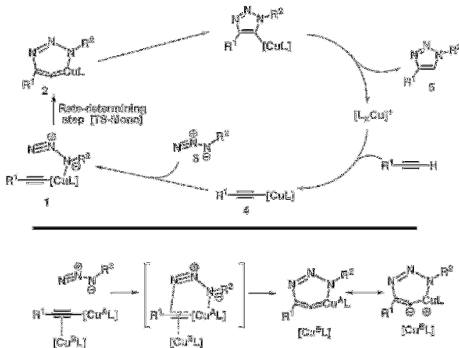
Fig. 1. The CuAAC mechanisms (Sharpless-type catalysis) proposed by Fokin and coworkers from their DFT calculations. Top: proposed mononuclear mechanism. Bottom: proposed dinuclear mechanism.
