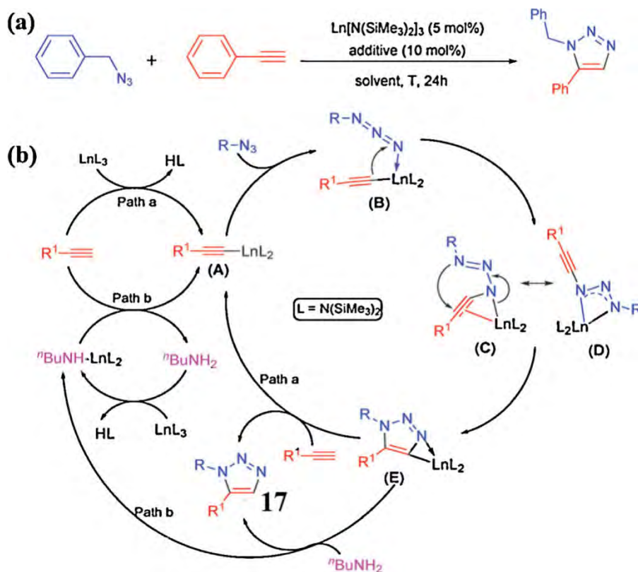
Fig. 20. (a) [\text{Ln}\{\text{N}(\text{SiMe}_3)_2\}_3] -catalyzed cycloaddition of terminal alkynes with azides ( \text{Ln} = \text{Sm}, \text{Nd}, \text{Y}, \text{Gd} ). (b) Reaction pathway for [\text{Ln}\{\text{N}(\text{SiMe}_3)_2\}_3] -catalyzed cycloaddition between terminal alkynes and azides.
