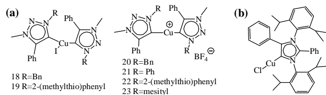
Fig. 23. (a) Copper(I)-triazolyldene complexes. (b) aNHC coordinated copper(I) chloro complex.
