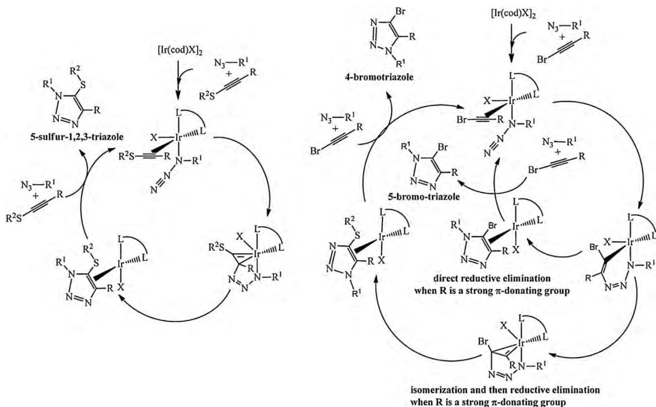
Fig. 16. The different IrAAC mechanisms proposed in the case of the addition of thioalkynes and bromoalkynes to azides in the presence of the [\text{Ir}(\text{cod})\text{X}]_2 ( \text{X} = \text{Cl} or \text{OMe} ) dimer.
