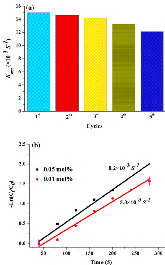
Figure 3 a Reusability of the RhAg 0.5 /rGO catalyst for the 4-NP reduction by NaBH 4 . b Plot of -\ln(C_t/C_0) versus time for the reduction of 4-NP by NaBH 4 in the presence of 0.05 and 0.01% RhAg 0.5 /rGO catalysts.
