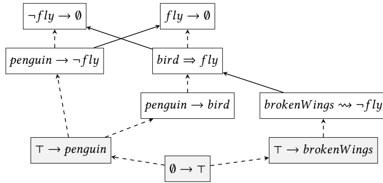
Figure 4.1: SG generated from \mathcal{KB} in Example 2.15.
