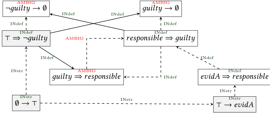
Figure 4.9: \mathbb{S}\mathbb{G}_{\mathcal{K}\mathcal{B}}^{\text{BDL}} of Example 4.7 with evidence for responsibility.
