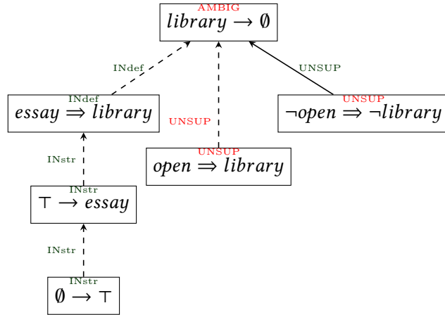
Figure 5.13: \mathbb{S}\mathbb{G}_{\mathcal{KB}_2}^{SUP} of Example 5.14.
