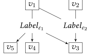
Figure 3.13: Bipartite depiction of the hypergraph in Example 3.2
