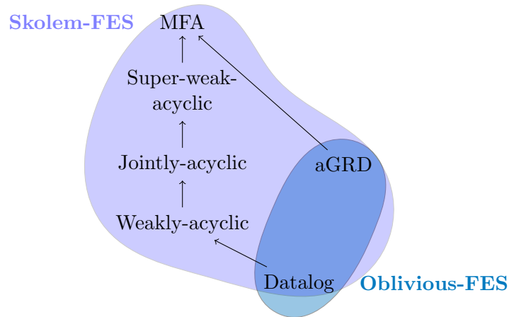
Figure 2.2: Known concrete FES classes and chases finiteness (all skolem-FES concrete classes are restricted-FES and core-FES cf. Proposition 3.4.)
