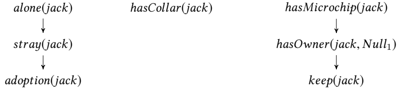
Figure 3.11: Chase graph for \sigma_{res} -chase( \mathcal{F}, \mathcal{R} ) if r_3 is applied before r_2
