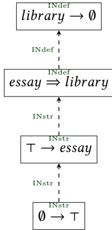
Figure 5.12: \mathbb{S}\mathbb{G}_{\mathcal{KB}_1}^{SUP} of Example 5.14.
