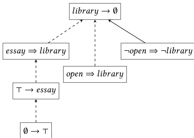
Figure 5.11: \text{SG}_{\mathcal{KB}_2} of Example 5.14.
