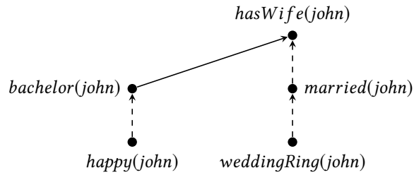
Figure 2.10: Inheritance Network of Example 2.21
