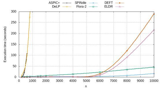
Figure 4.16: Response time for chain(n)
