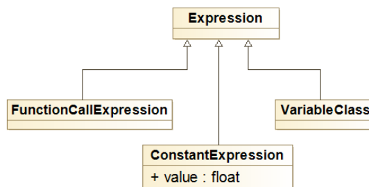
Figure 5.12 – Expression class diagram
