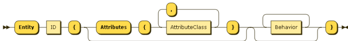
Figure 5.17 – Syntax diagram for an entity definition
