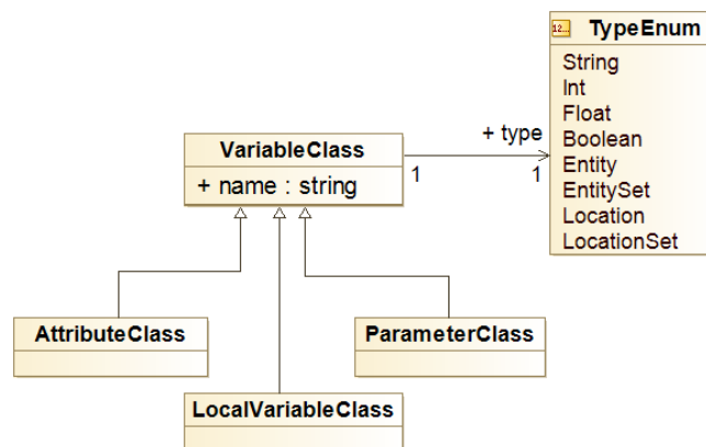
Figure 5.13 – VariableClass class diagram
