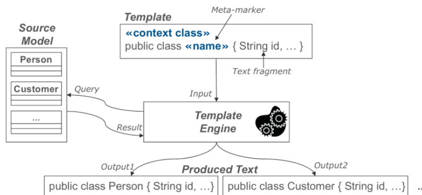
Figure 3.14 – Template approach mechanism in M2T. Source : Brambilla et al., 2012
