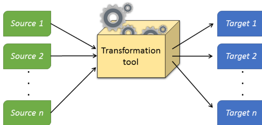
Figure 3.6 – Model Transformation.
