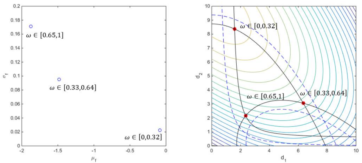
Fig. 1.36. Results for Formulation 7
