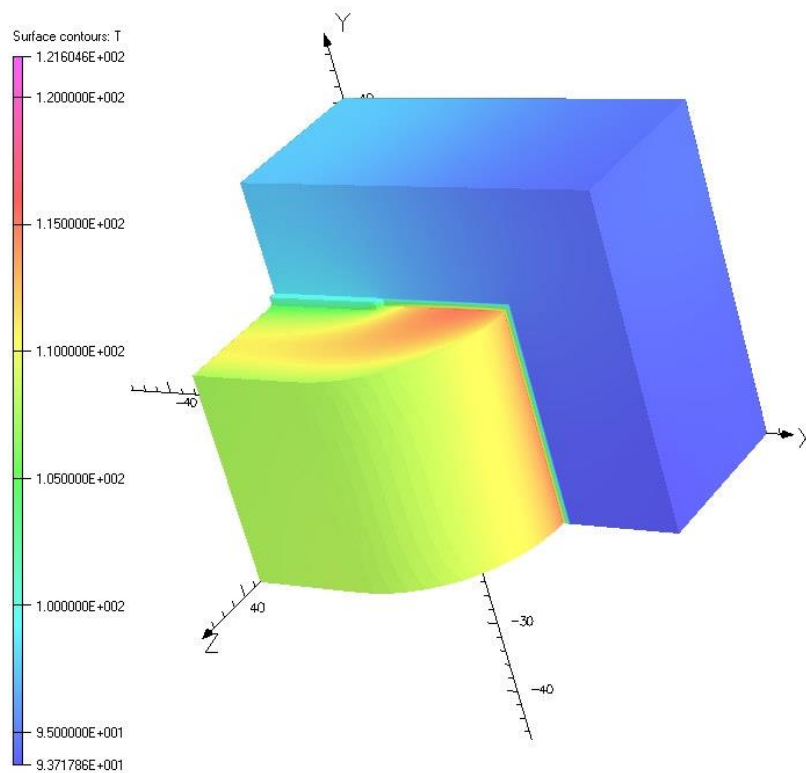
Fig. 3.7. 3D Finite element thermal simulation (Tran, 2009)
