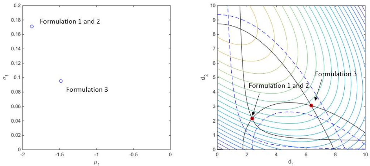
Fig. 1.31. Results for the formulation 1, 2 and 3
