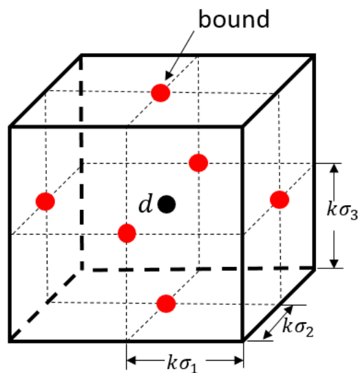
Fig. 1.5. A hyper-rectangular uncertainty set and the bound points for a three-dimensional variables
