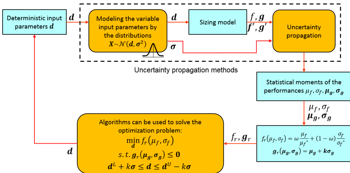
Fig. 1.9. Process of Robust Design Optimization
