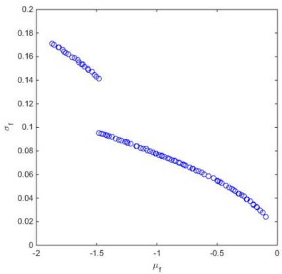
Fig. 1.40. Results for Formulation 9 using NSGA2
