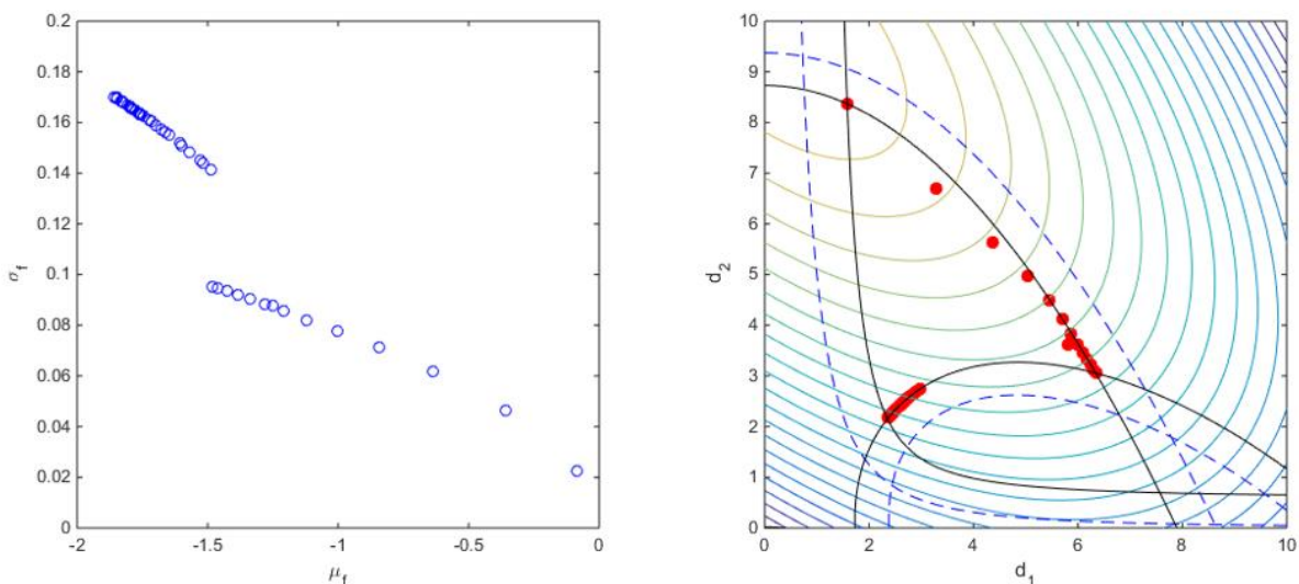
Fig. 1.37. Results for Formulation 8 using goal-attainment
