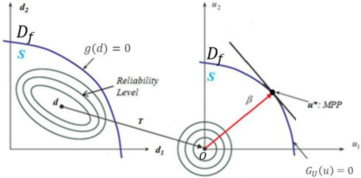
Fig. 1.11. The first order reliability method (Lopez & Beck, 2012)
