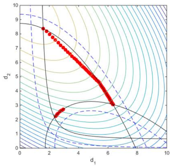
Fig. 1.39. Results for Formulation 9 using goal-attainment
