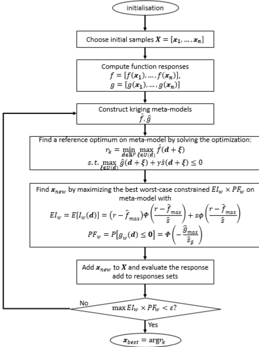
Fig. 2.7. The flowchart of worst-case optimization with constrained problems
