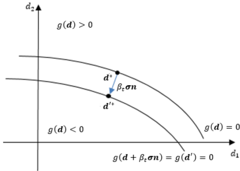
Fig. 1.21. Principle of the SLA approach
