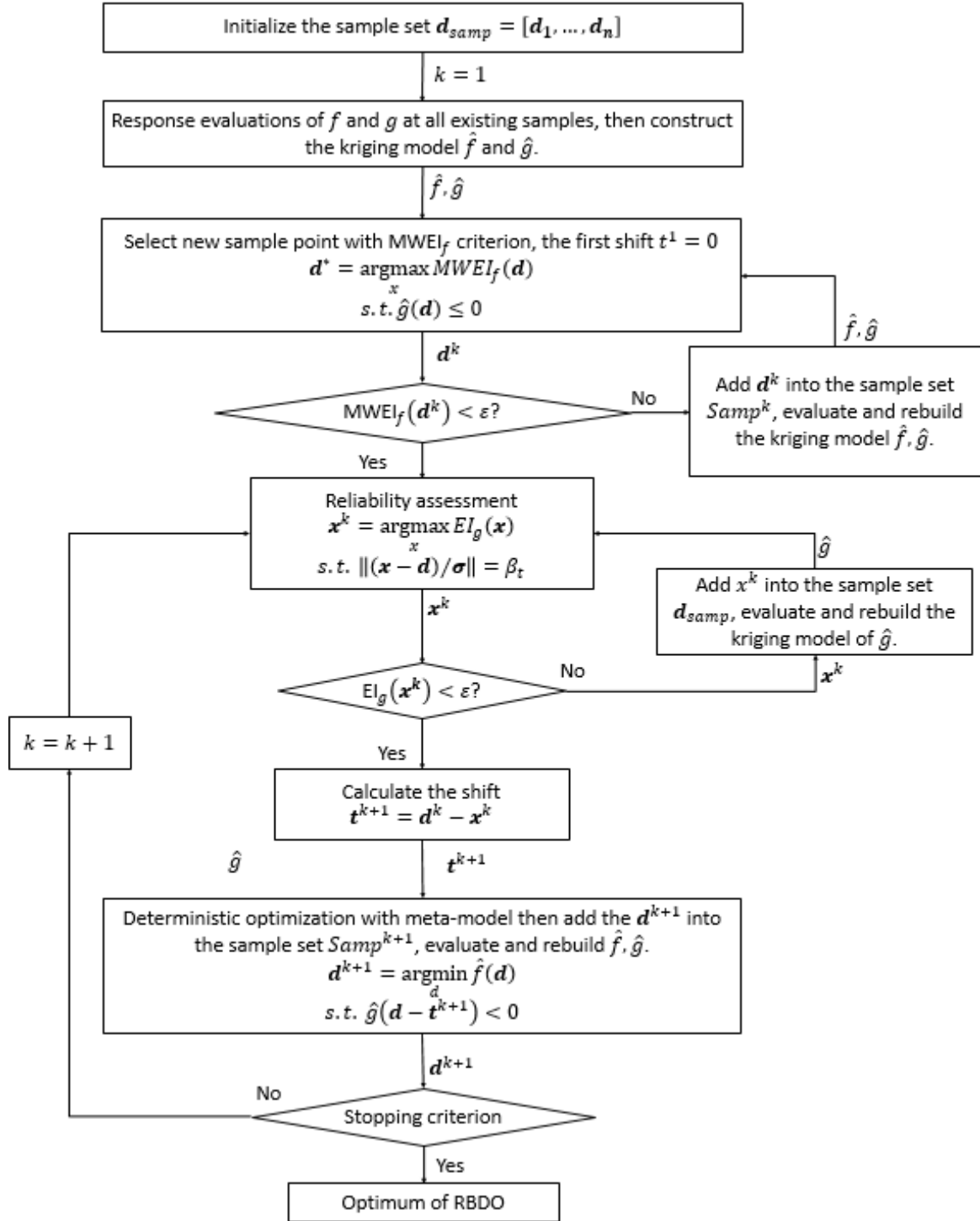
Fig. 2.20. The process of SORA2 strategy
