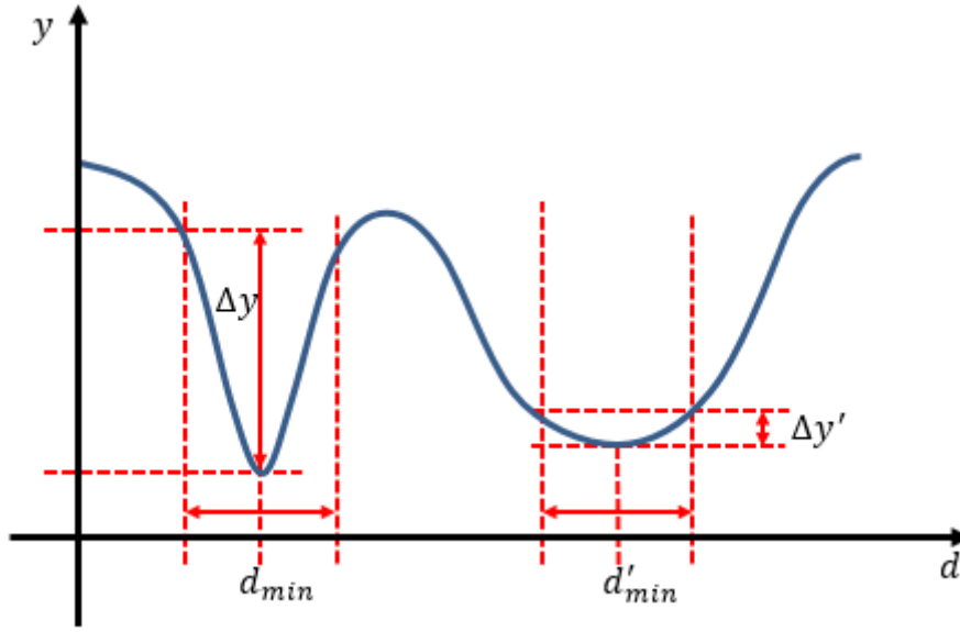
Fig. 1.7. Deterministic optimum and robust optimum
