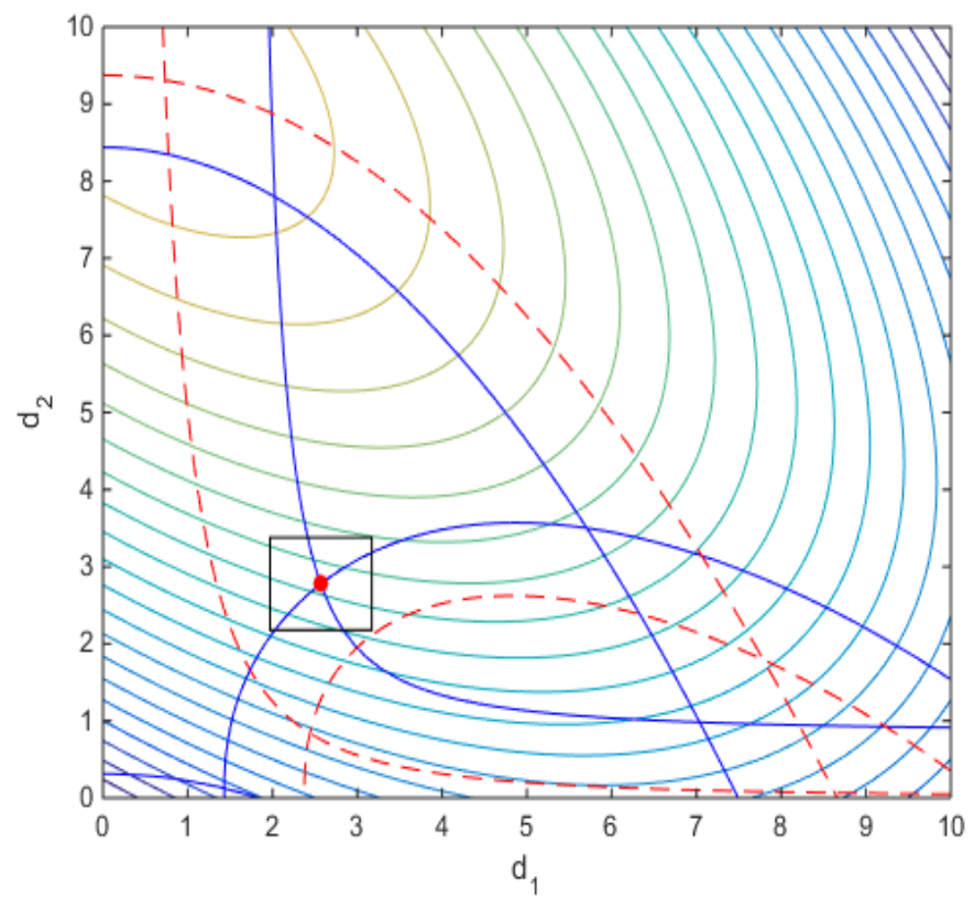
Fig. 1.30. Optimum and worst-case of constraints obtained by first order GWCO
