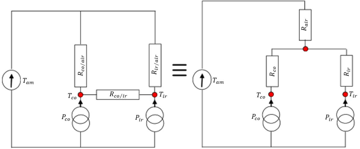
Fig. 3.4. Transform equivalent of the nodal thermal model (Tran, 2009)
