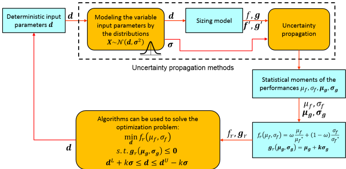
Fig. 1.9. Process of Robust Design Optimization
