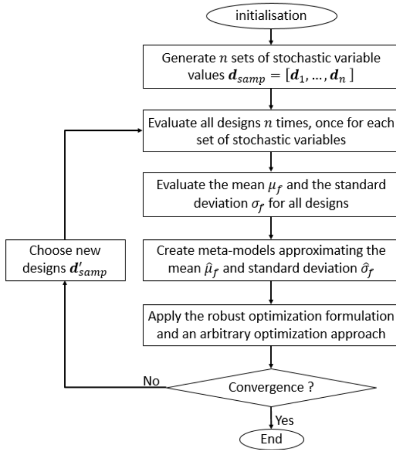
Fig. 2.10. Flowchart for the methodology used in (David, Fyllingen & Nilsson, 2008)
