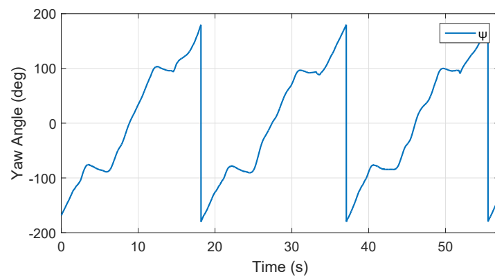
Figure 5.49: The yaw angle changes according to its position during the following.
