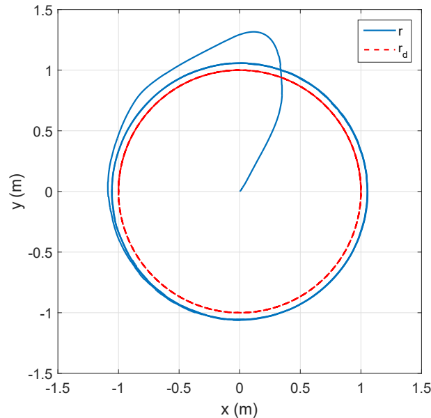
Figure 4.6: Following of a circular path by using a nonlinear control in ground mode. The thrust is constant and the algorithm must control the pitch angle in order to track the trajectory. The addition of an external force in simulation creates a gap between the two trajectories.
