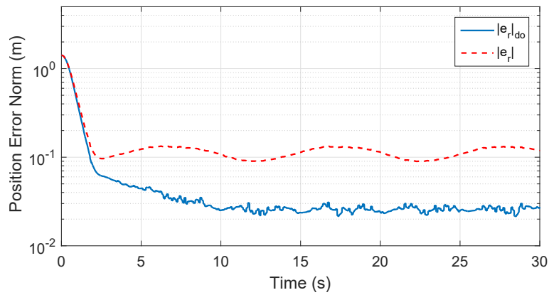
Figure 4.33: The norm of the position error with compensation using the disturbance observer (do). The new error in solid line is lower than the error without compensation in dashed line.
