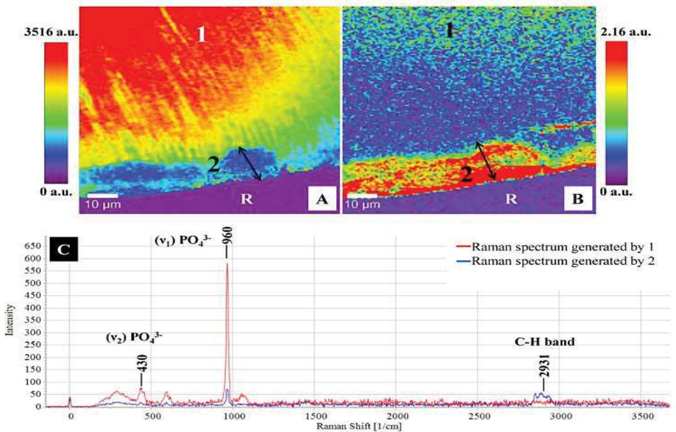
Figure 1. (A) Raman phosphate map built from phosphate peak intensity at 960\text{ cm}^{-1} . (B) Image constructed from organic to mineral ratio at (2931/430\text{ cm}^{-1}) . Individual Look Up Tables (LUT) on both sides. Region 1: Sound enamel, Region 2: Lesion area, R: Resin. (C) Corresponding Raman spectra generated by region 1, 2 respectively.
