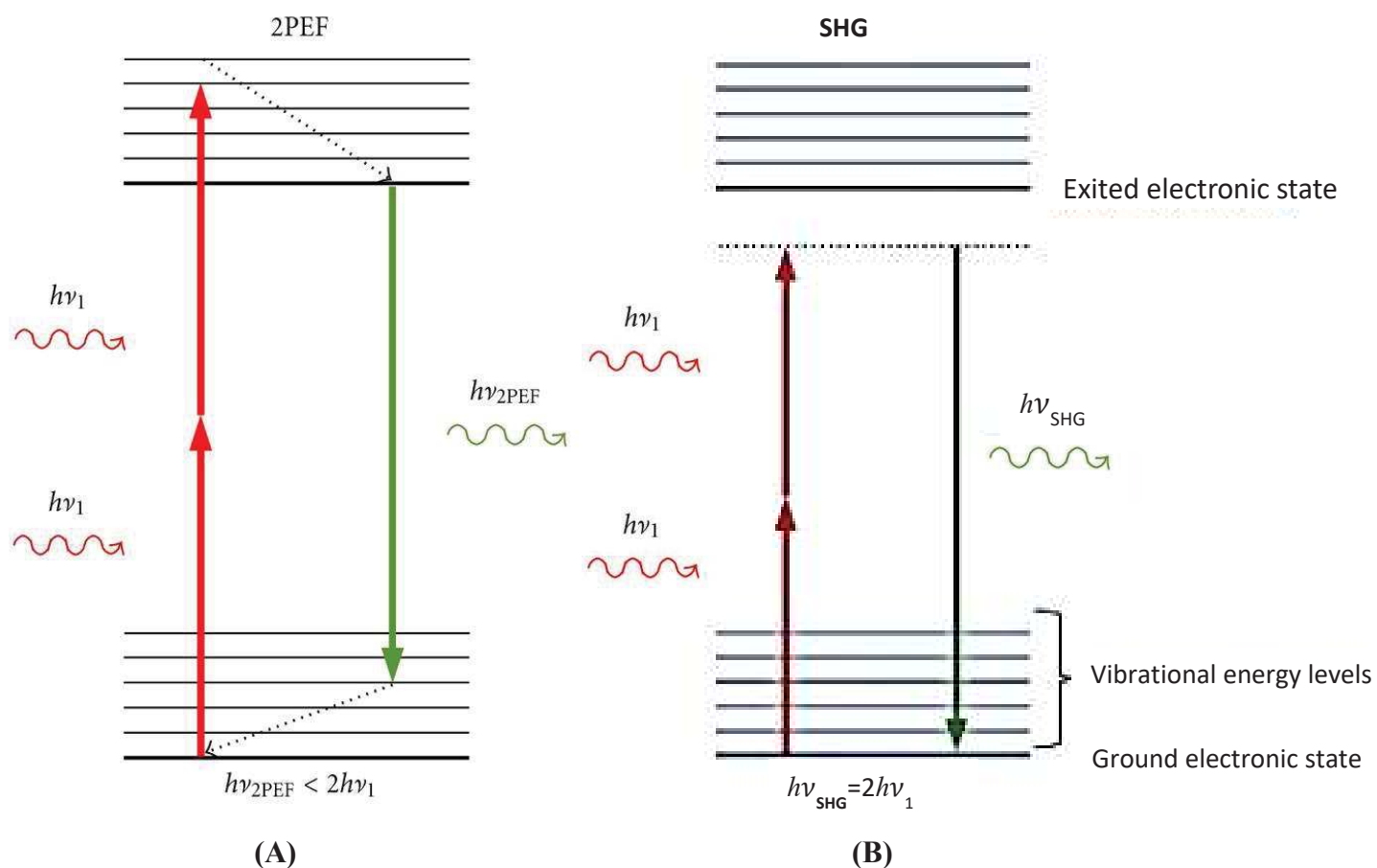
Figure 4. Jablonski diagram showing the interaction of multiple infrared photons with the electronic and vibrational energy levels of a molecule. (A) In two-photon excitation fluorescence (2PEF), the molecule absorbs two infrared photons that stimulate it to the excited electronic state. After non-radiant relaxation to a lower vibrational level, the molecule emits a lower energy (red-shifted) photon. (B) In second harmonic generation (SHG), two infrared photons are instantaneously up converted to a single photon of twice the energy.
