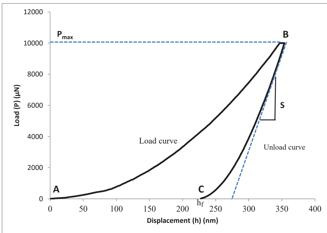
Figure 2. Schematic illustration of nano-indentation load–displacement curve showing important measured parameters
